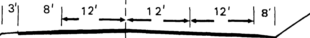
ALTERNATIVES C, E Sections With Uphill Truck-Passing Lane
