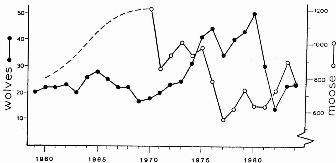
Figure 1. Isle Royale wolf and moose population levels, 1959-84.
