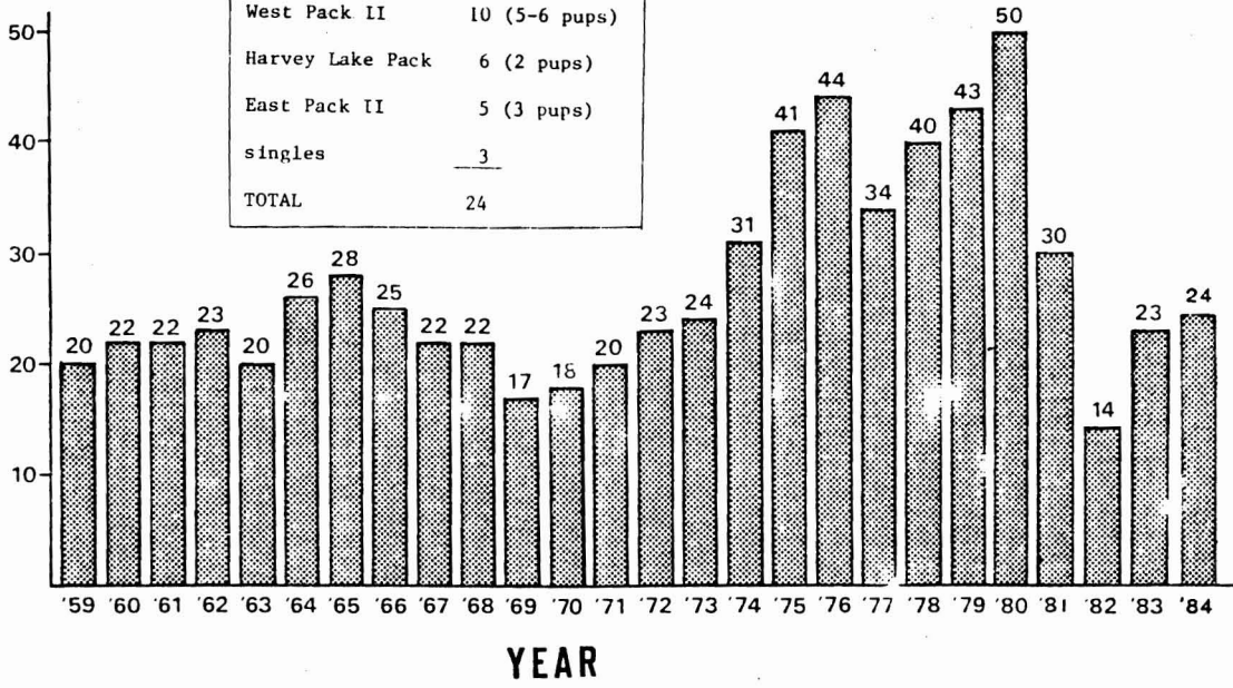
Figure 3. Isle Royale wolf population fluctuations, 1959-84.
