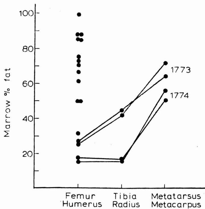
Figure 6. Marrow fat values from wolf-killed moose on Isle Royale, 1984. Connected values are from a single leg.
