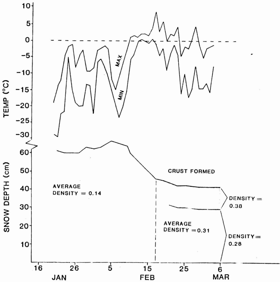
Figure 8. Precipitation and snow depth in open areas at Windigo, 1984.
