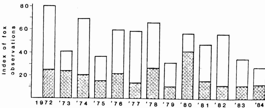
Figure 9. Midwinter fox index, 1972-84. The lower bar is the number of foxes seen more than 1 km from a moose carcass/100 hrs flying time, while the upper bar is the sum of the maximum number of foxes seen on each moose carcass.
