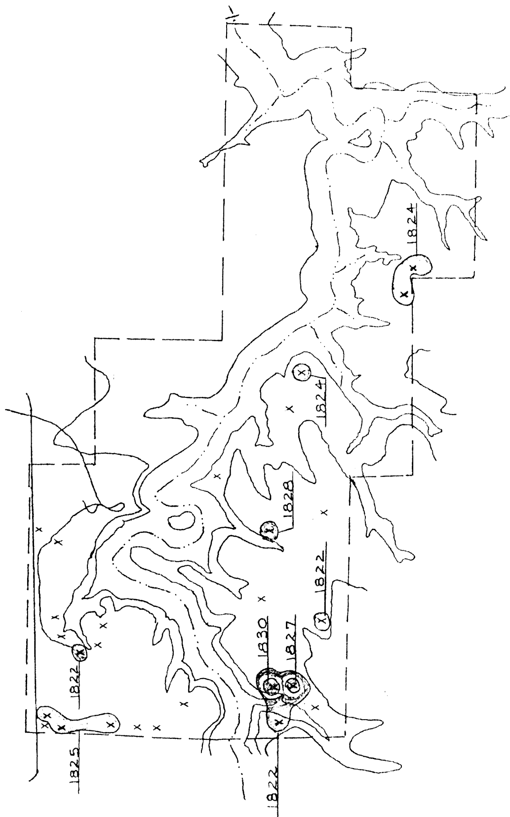
Figure 3g. Relative fire spread for fires in 1830, 1828, 1827, 1825, 1824, and 1822.
