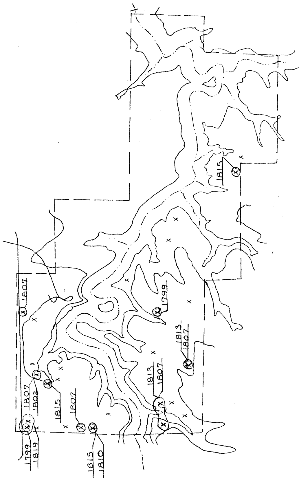
Figure 3h. Relative fire spread for fires in 1819, 1815, 1810, 1807, 1802, and 1799.
