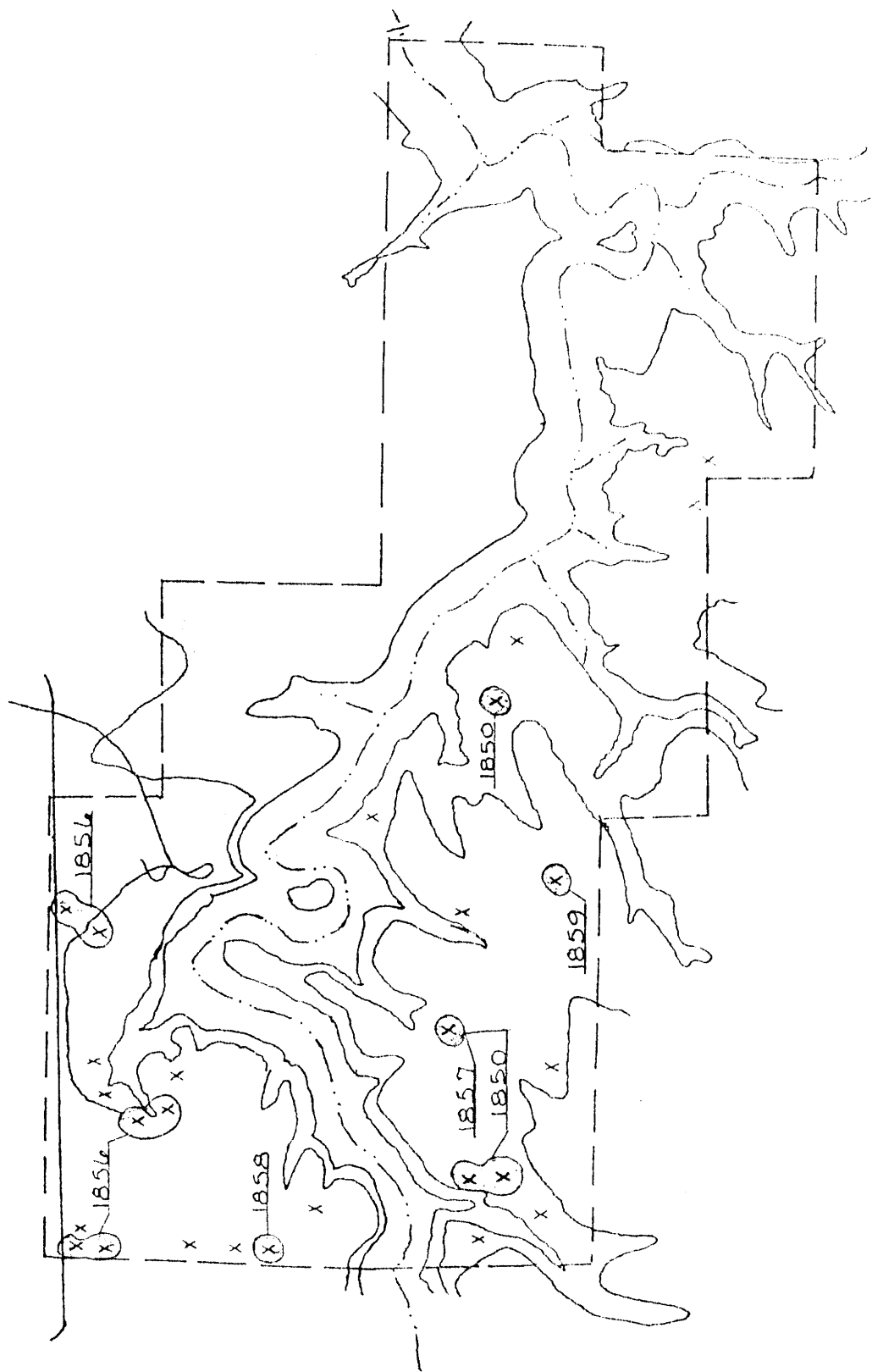
Figure 3d. Relative fire spread for fires in 1859, 1858, 1857, 1856, and 1850.
