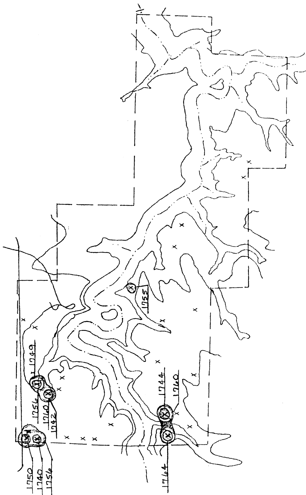
Figure 3k. Relative fire spread for fires in 1764, 1760, 1756, 1755, 1750, 1749, 1744, 1742, and 1740.
