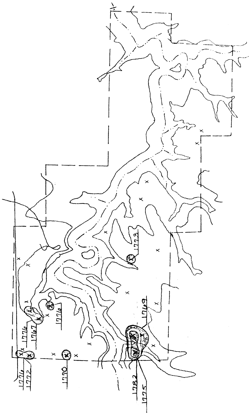
Figure 3j. Relative fire spread for fires in 1782, 1776, 1773, 1775, 1772, 1770, 1769, and 1767.
