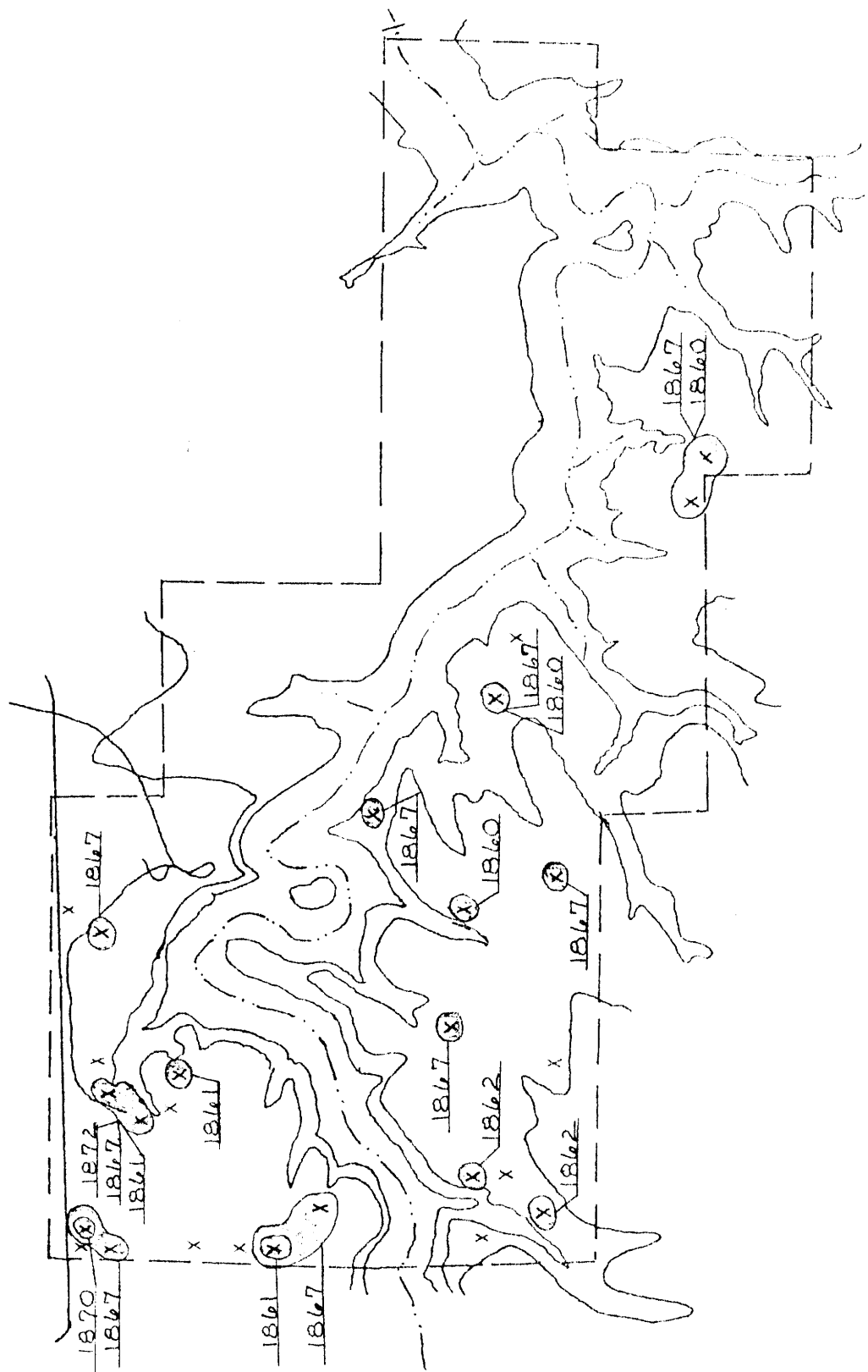
Figure 3c. Relative fire spread for fires in 1872, 1870, 1867, 1862, 1861, and 1860.
