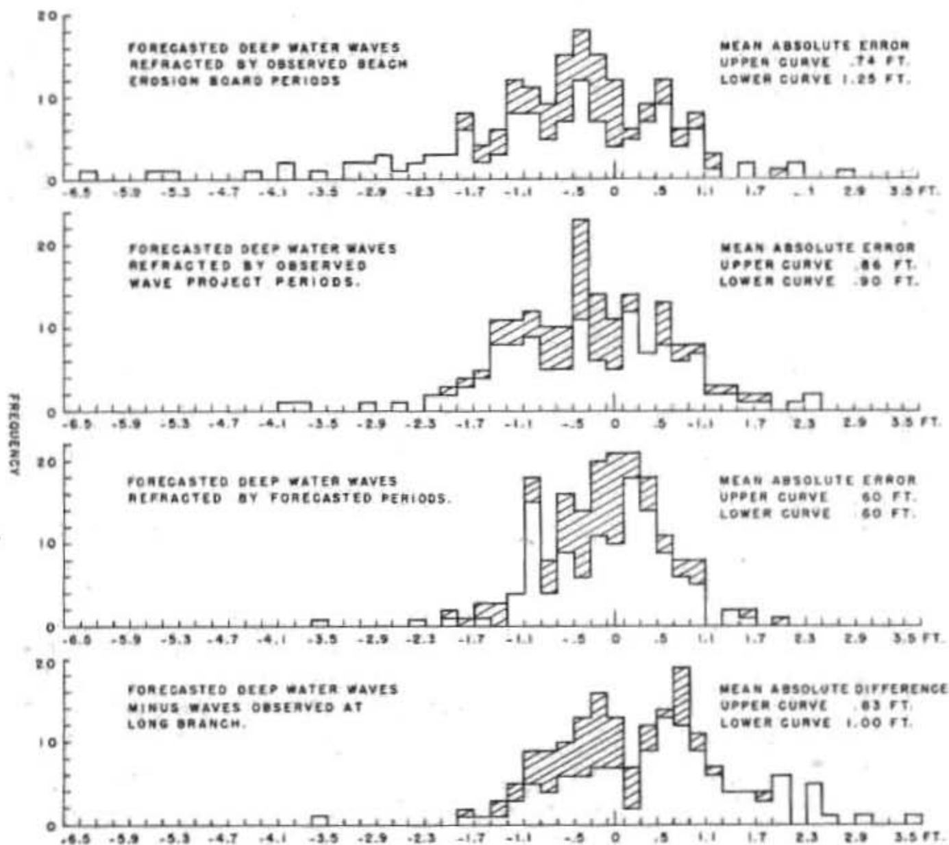
FIG. 25 ATTEMPTED VERIFICATION OF REFRACTION DIAGRAM
