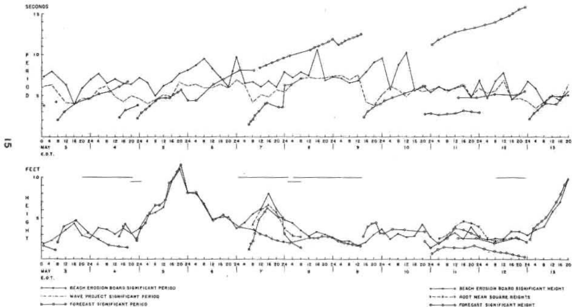
GRAPHS OF FORECAST AND OBSERVED WAVE PARAMETERS
