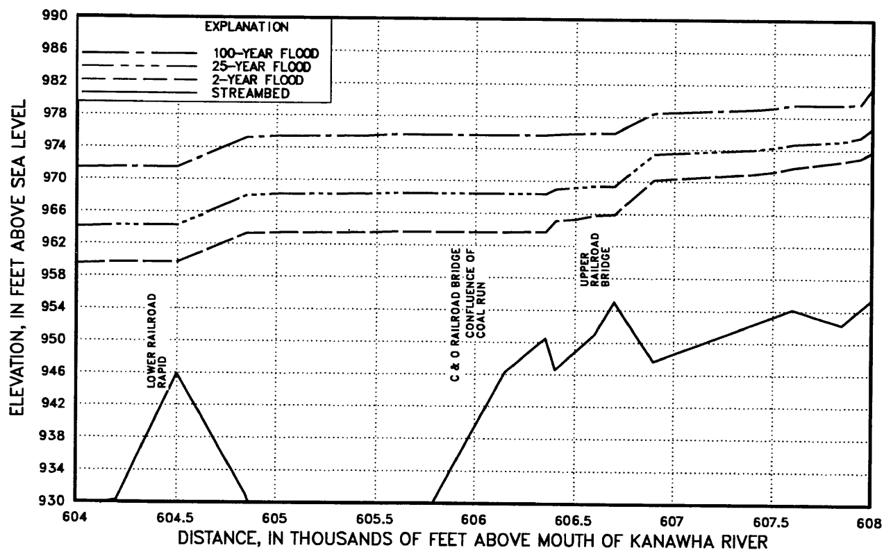
Figure 4.--Flood and streambed profiles for the New River.--Continued
