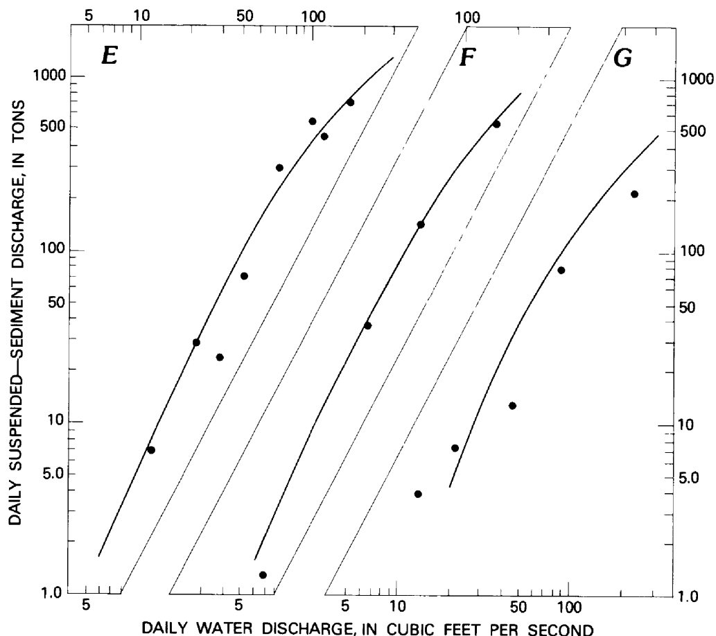
1968–Mar. 1969, (C) Apr. 1969–Mar. 1971, (D) Apr. 1971–Dec. 1971, (E) Jan. 1972–Sept. 1976; North Branch Rock Creek near Norbeck.
