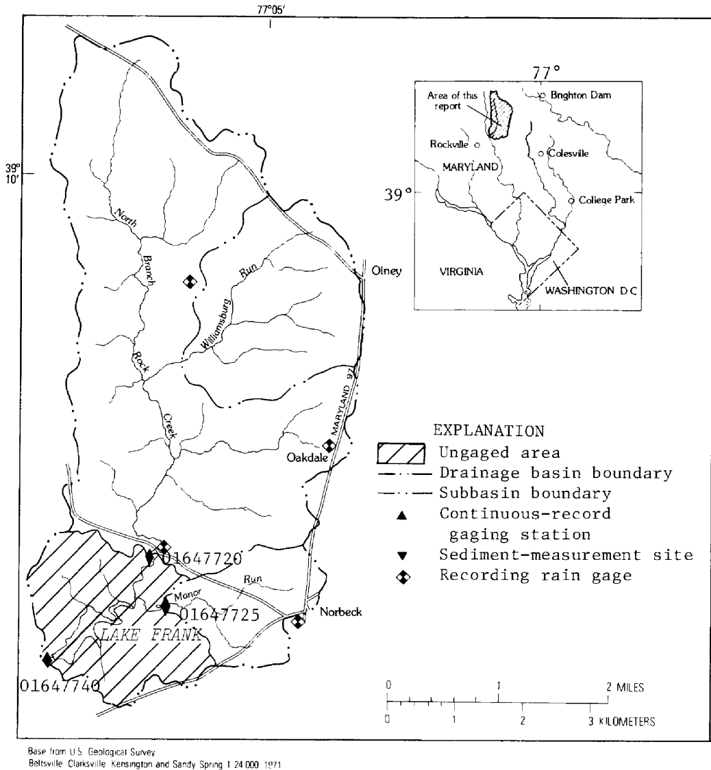
FIGURE 1.—Location of North Branch Rock Creek basin.
