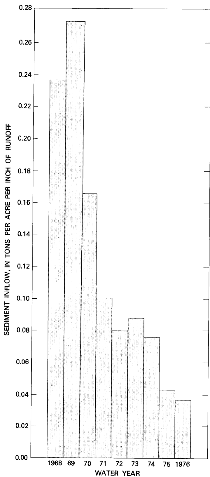
FIGURE 18.—Annual sediment inflow to Lake Bernard Frank per inch of runoff.
