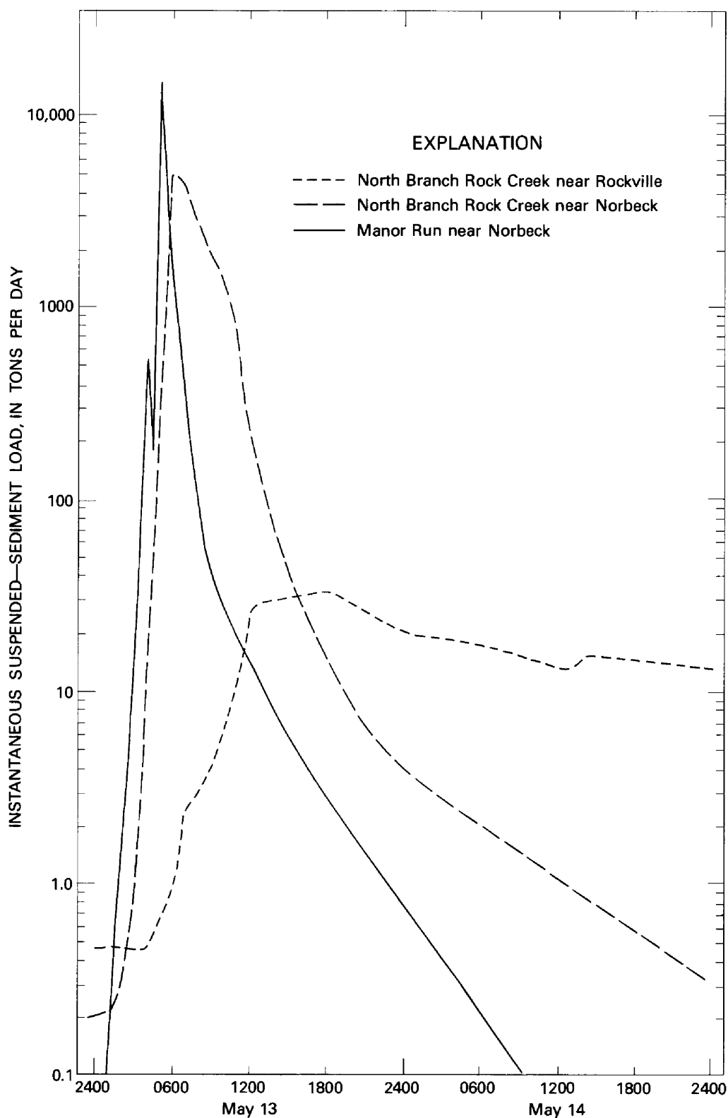
FIGURE 13.—Instantaneous suspended-sediment load for storm of May 13-14, 1971.
