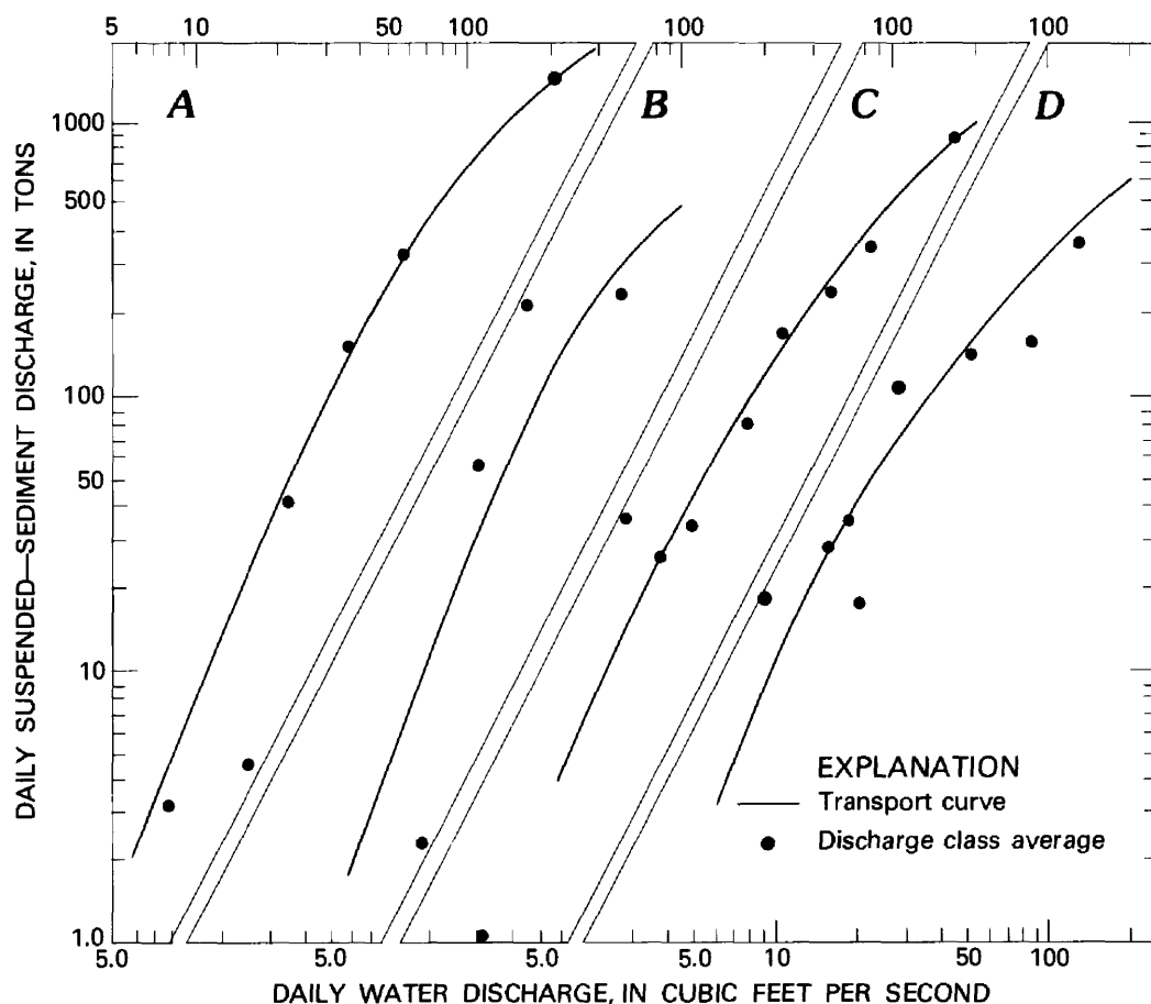
FIGURE 9.—Suspended-sediment transport curves (A) Oct. 1967-Mar. 1968, (B) Apr. Dec. 1973, (C) Jan. 1974-Sept. 1974, (D) Oct. 1974-
