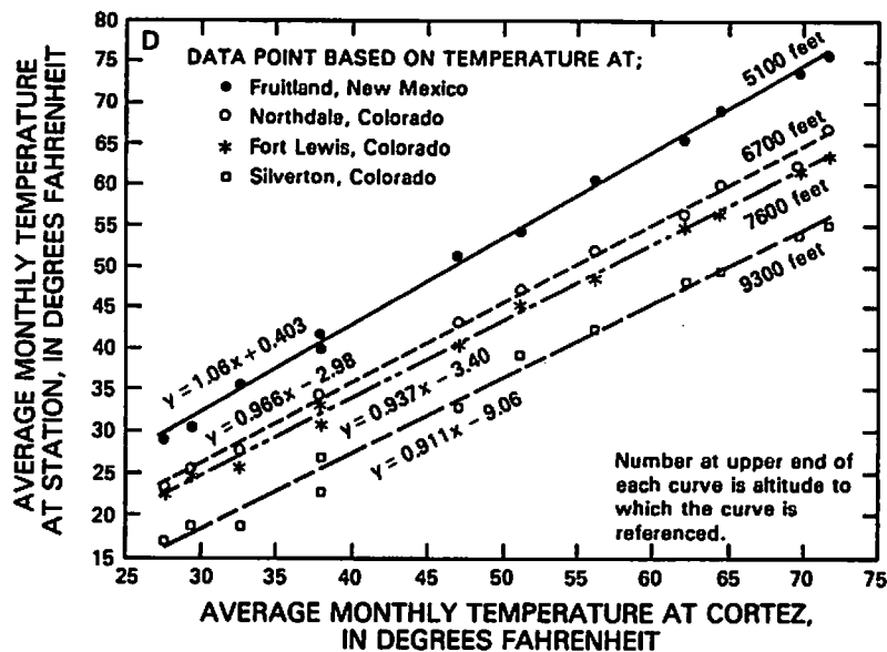
Figure 4.--Relations of precipitation and temperature to altitude in the Four Corners area, 1930-80.
