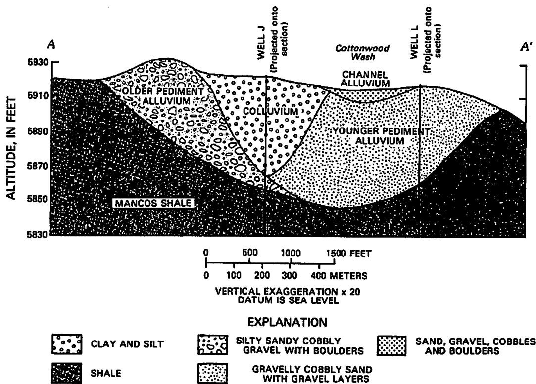
B. GEOLOGIC SECTION ACROSS COTTONWOOD WASH (LOCATION SHOWN ON FIGURE 2)
