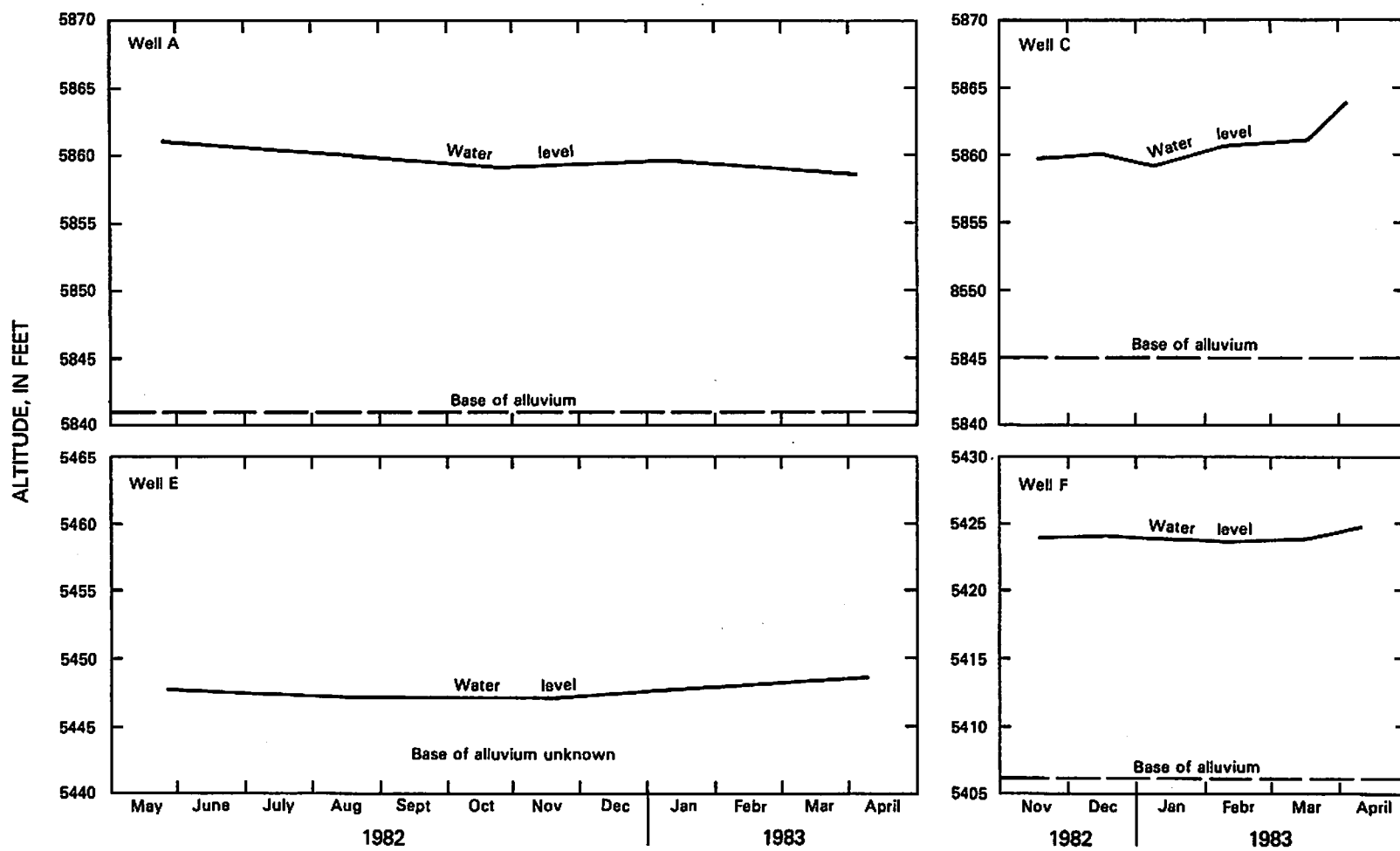
Figure 10.--Recorded water levels in alluvium, 1982-83.
