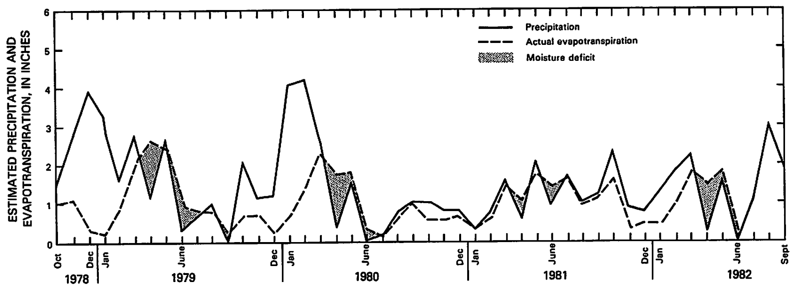
Figure 6.--Estimated monthly precipitation, evapotranspiration, and moisture deficits, calendar years 1978-82.
