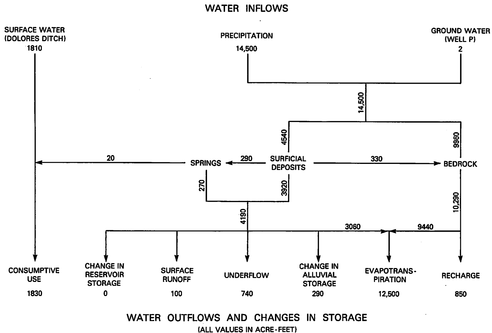
Figure 12.--Generalized water budget for 1982 water year.
