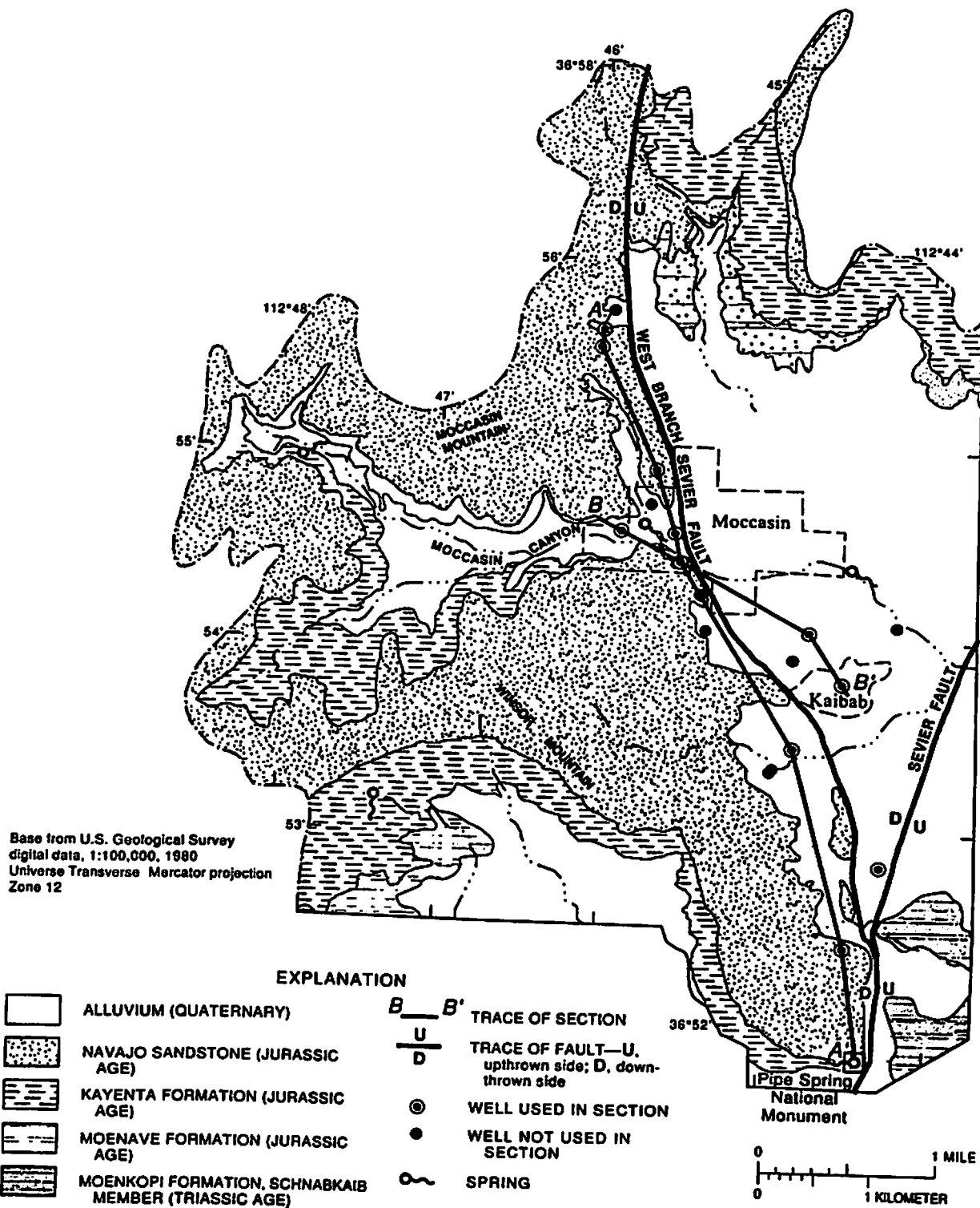
Figure 6. Surface geology and geologic structure, Pipe Spring National Monument area, northern Arizona (modified from Hemphill, 1956; Marshall, 1965; and Pillmore, 1956; by Robert Rosé, volunteer geologist, NPS, written commun., 1998).
