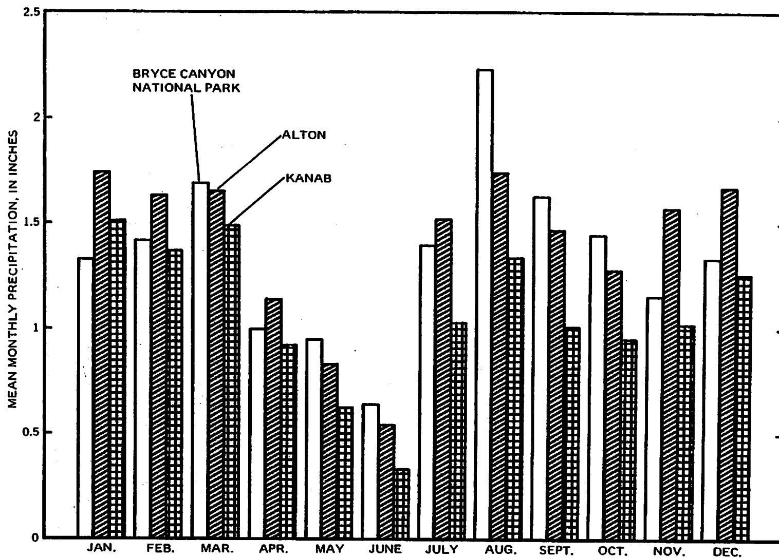
Figure 5.—Monthly variation in precipitation at the Bryce Canyon National Park, Alton, and Kanab climatologic stations (1931-86).
