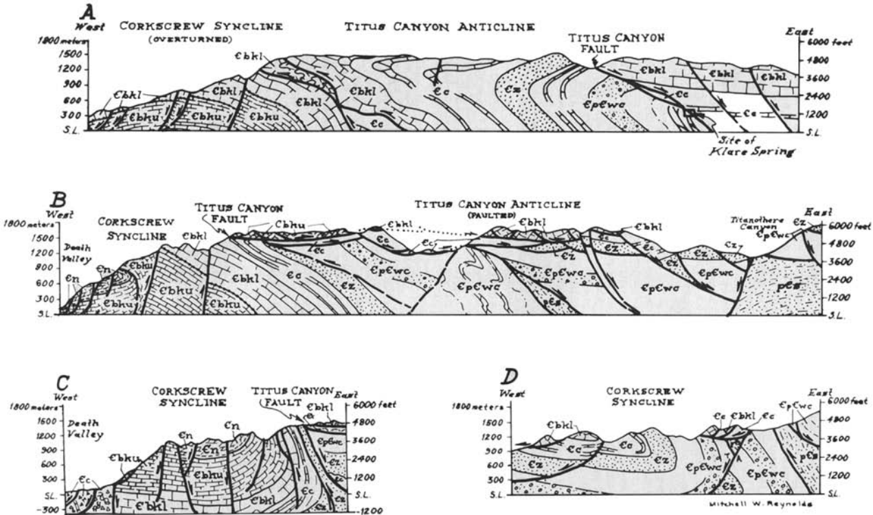
Figure 3. Generalized geologic sections of part of the southern Grapevine Mountains, Death Valley, California.
