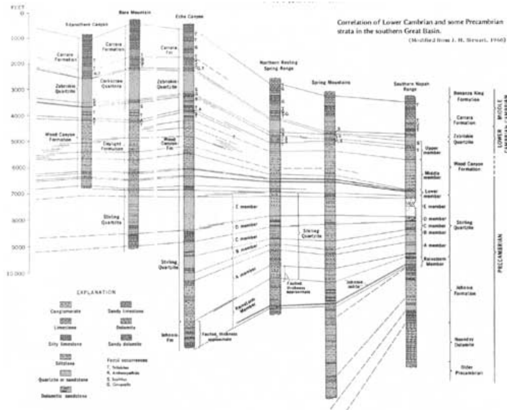
Correlation of Lower Cambrian and some Precambrian strata in the southern Great Basin. (Modified from J. H. Stewart, 1966) ( click on image for a PDF version )
