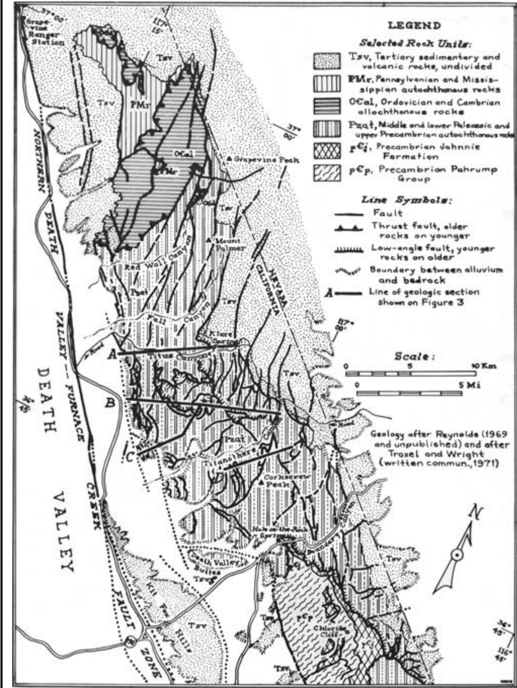
Figure 1. Generalized geologic map of the Grapevine and northern part of the Funeral Mountains, Death Valley, California, showing localities referred to in the text. (click on image for a PDF version)
