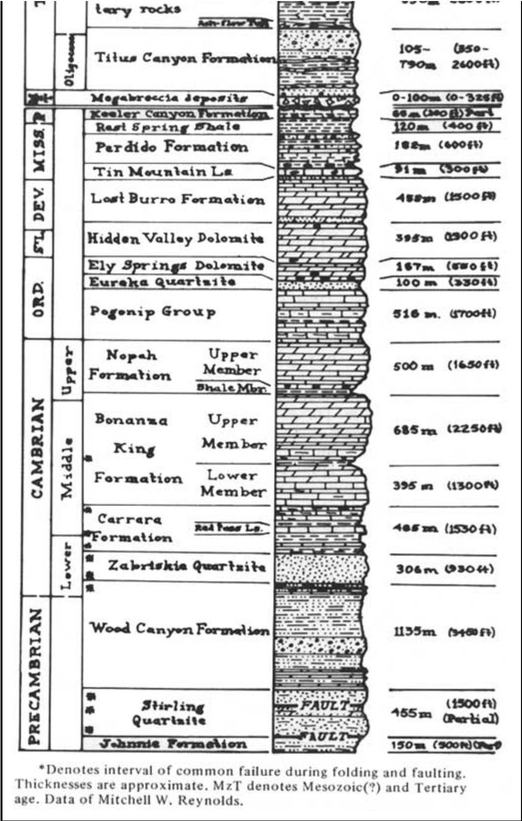
Figure 2. Generalized columnar section of rocks exposed in the Grapevine Mountains, Death Valley, California.
