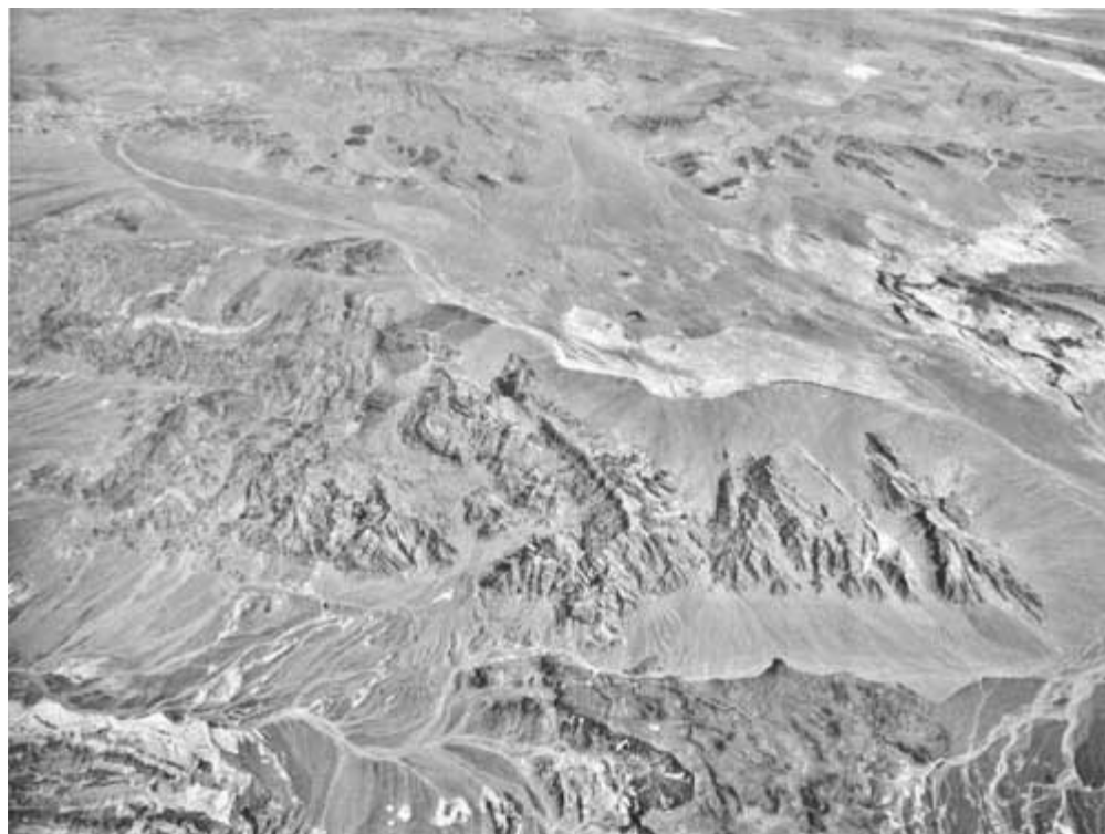
High-altitude oblique aerial photograph to northeast across southern Funeral Mountains taken from a point barely south of Ryan (lowermost center). Trace of Northern Death Valley-Furnace Creek fault zone extends across lower one-third of photograph. Rocks mostly Tertiary in age lie on near side of fault zone; late Precambrian and Paleozoic rocks lie beyond the fault, in Funeral Mountains. Rocks on left in the range are older and are moderately to strongly folded; rocks on right are younger and deformed mainly by eastward tilting. Tertiary sedimentary rocks lie at extreme right end of range. All rocks are repeated by abundant west-dipping normal faults. A major part of the Basin and Range province occupies rest of photograph. Ranges are dark-colored; basins contain pale-colored playa sediment. Photo U.S. Air Force 374L 193, 6 September 1968; courtesy of the U.S. Geological Survey.
