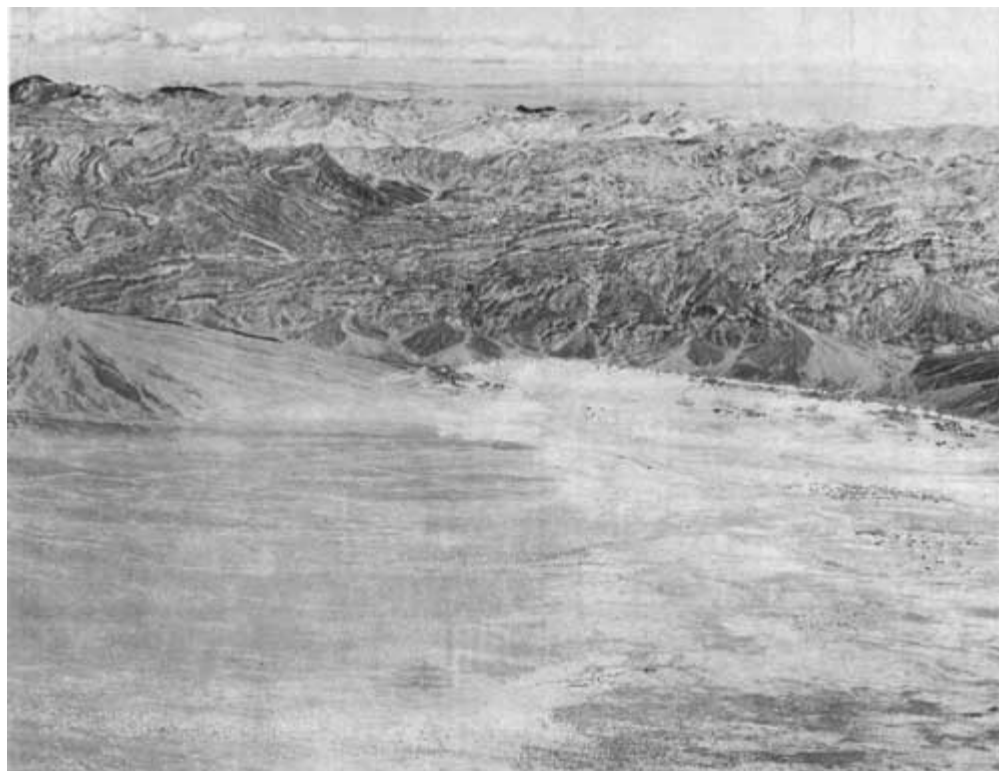
Low altitude oblique aerial photograph across Death Valley northeast of Grapevine Mountains between mouth of Titus Canyon (left) and Titanother Canyon (right). Pale rocks just below skyline are Tertiary rocks, mostly volcanic. Stratified rocks in Grapevine Mountains range in age from early Cambrian (right) to late Paleozoic (left) and are highly deformed. See article that follows. Photo W16 by John H. Maxson; courtesy of the National Park Service.
