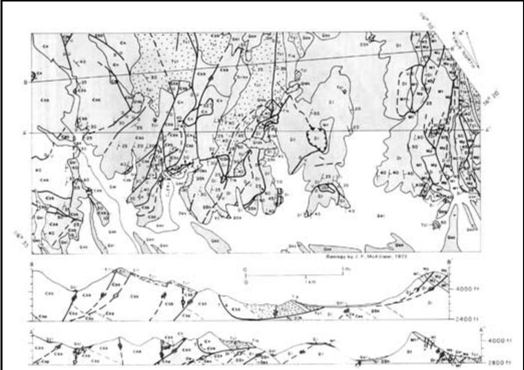
Figure 2. Geology at southeast end of Funeral Mountains. Explanation of map units in Table 1. (click on image for a PDF version)
