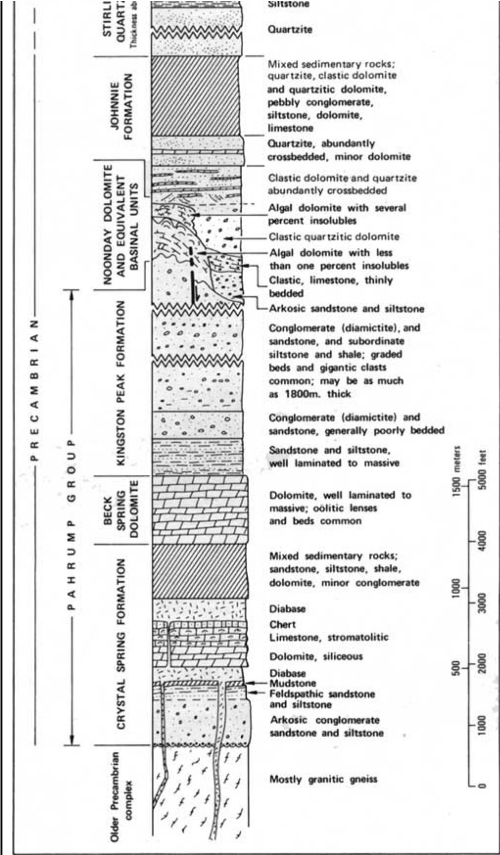
Figure 1. Generalized columnar section of Precambrian to Lower Cambrian strata, Death Valley region.
