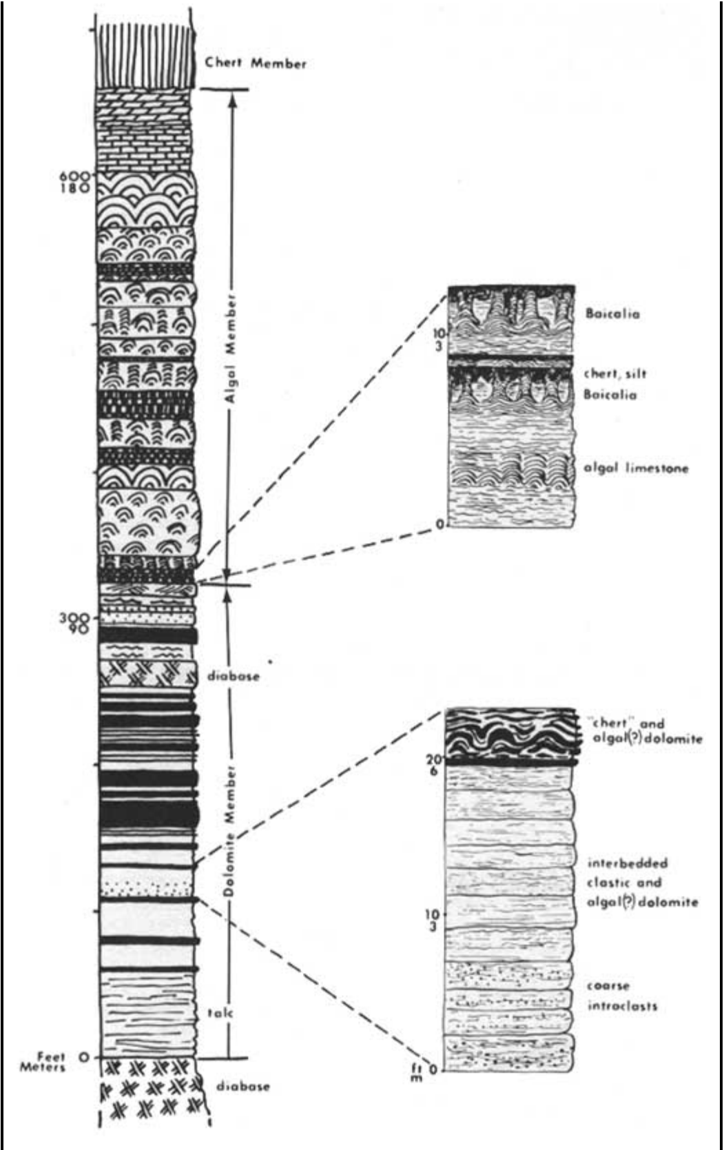
Figure 5. Stratigraphic column of carbonate members in Alexander Hills area. Lower inset details lithologies of single cycle of dolomite member (solid black units of column correspond to upper, ribbed strata of inset; solid white units of column correspond to lower strata of inset). Upper inset details stromatolite cycles within basal zone of larger stromatolitic cycles of algal member. At top of dolomite member is zone of rippled and cross-stratified clastic limestone.
