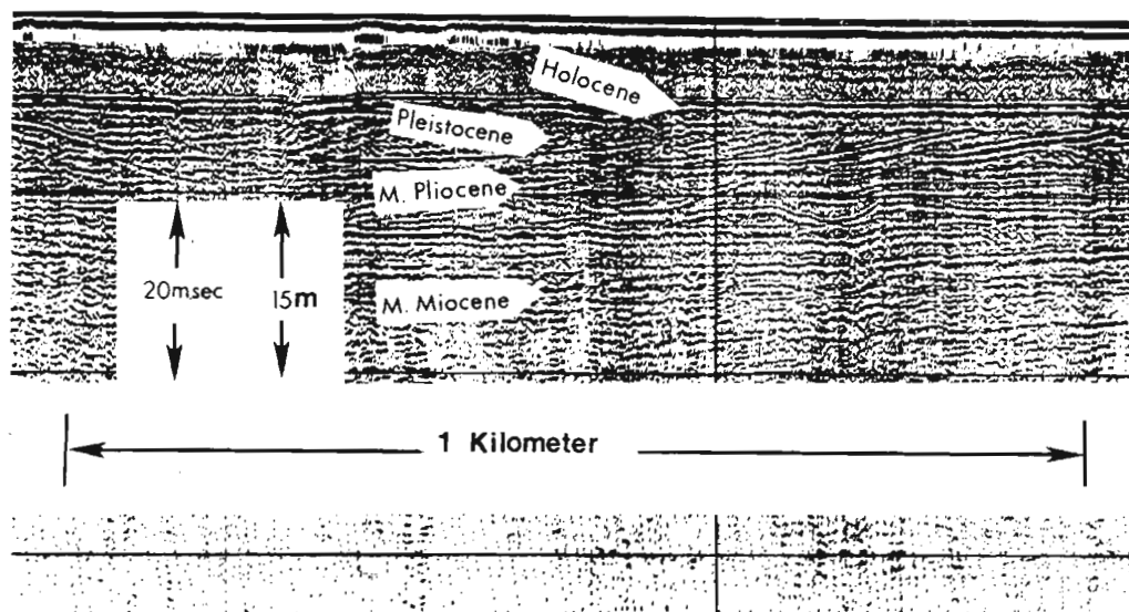
Figure 4—10. Seismic profile in Cumberland River, 2 km south of Cumberland Wharf, showing thin Holocene deposits unconformably overlying sediments of Pleistocene crossbedded deposits. The latter overlie middle Pliocene sediments. A horizontal unconformity defines the boundary between Pliocene sediments and the limestone (middle Miocene).
