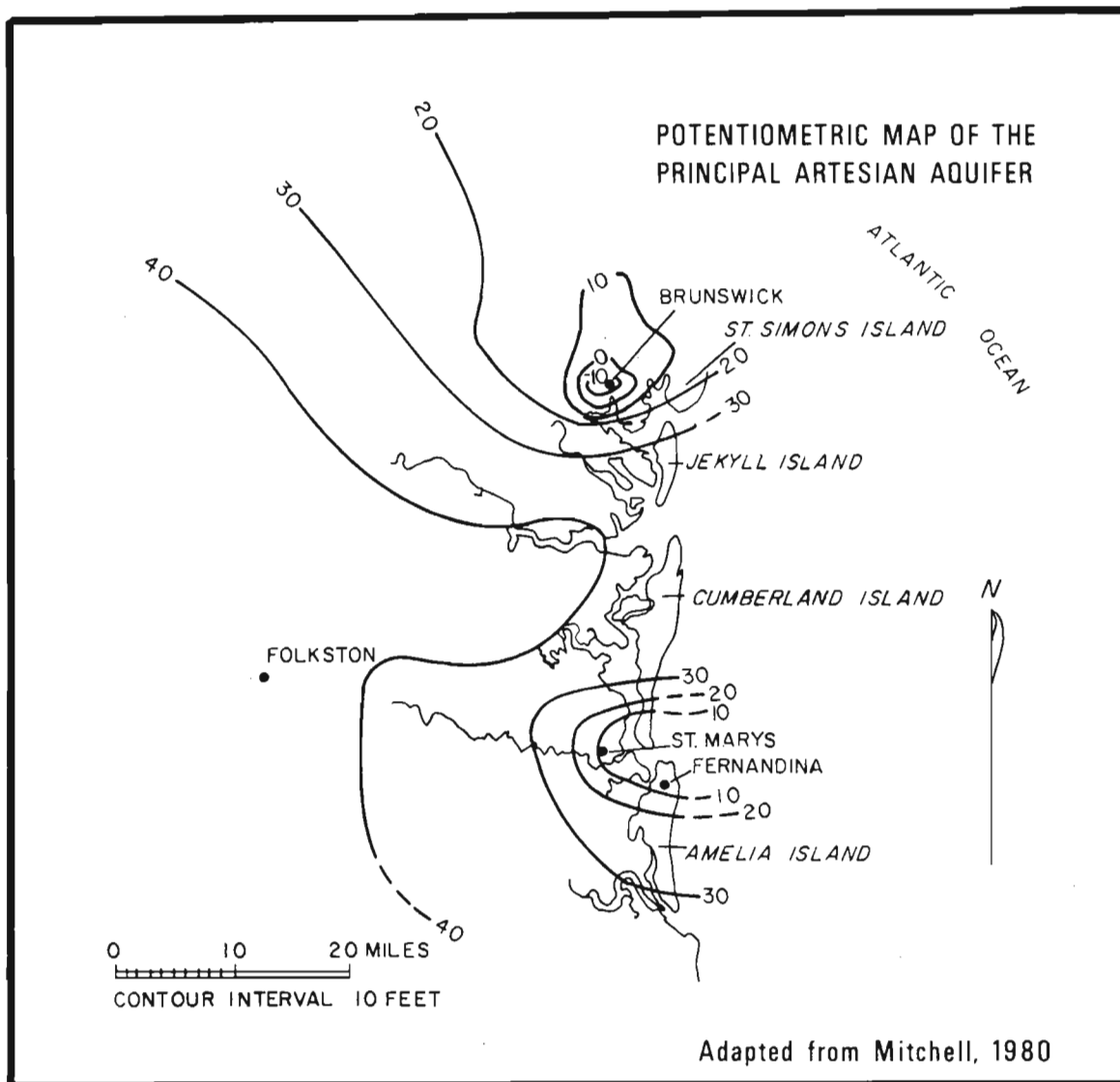
Figure 5-3. Potentiometric map of the Principal Artesian Aquifer in southeast Georgia.
