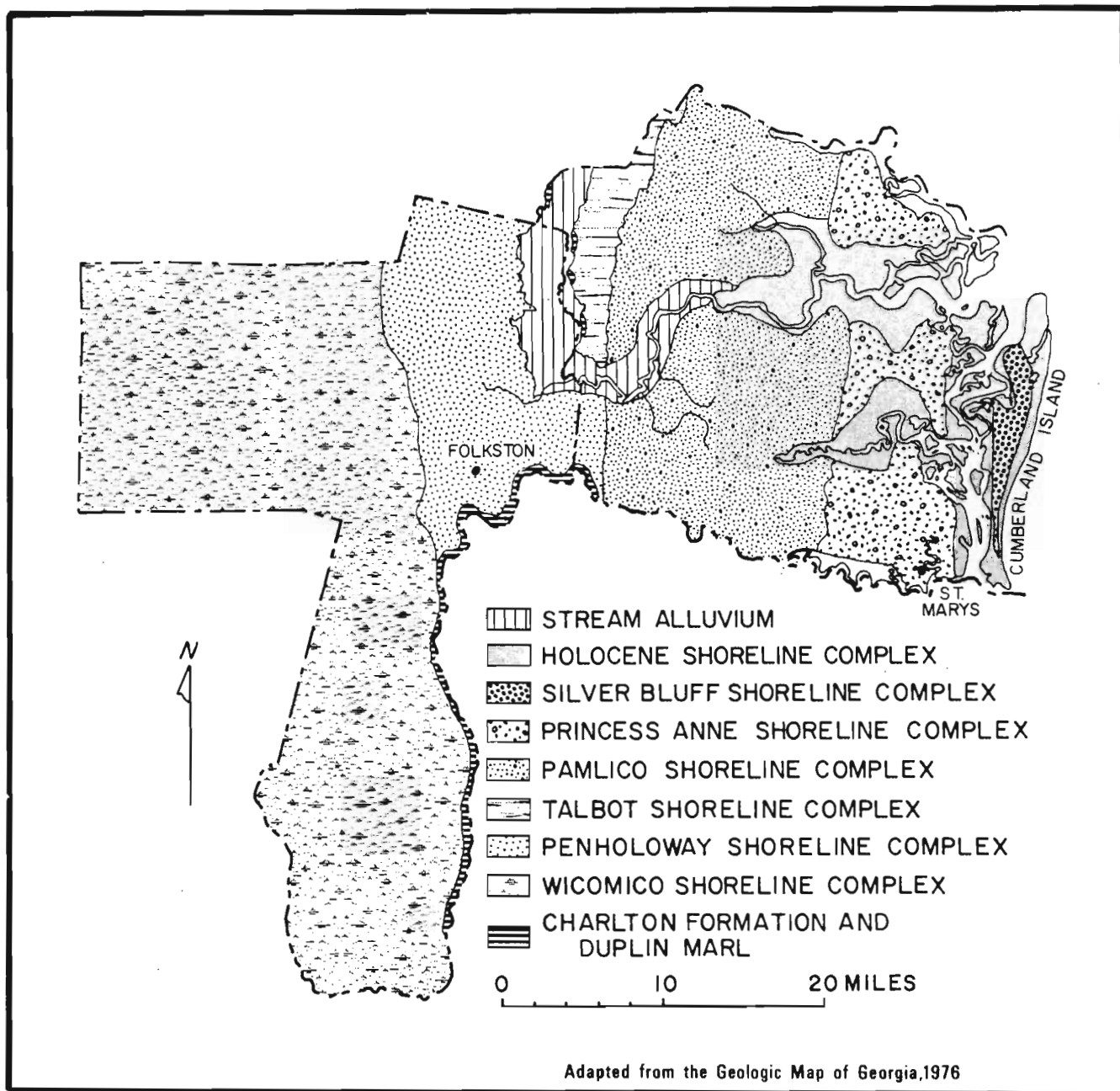
Figure 3—1. Regional geology of southeast Georgia.
