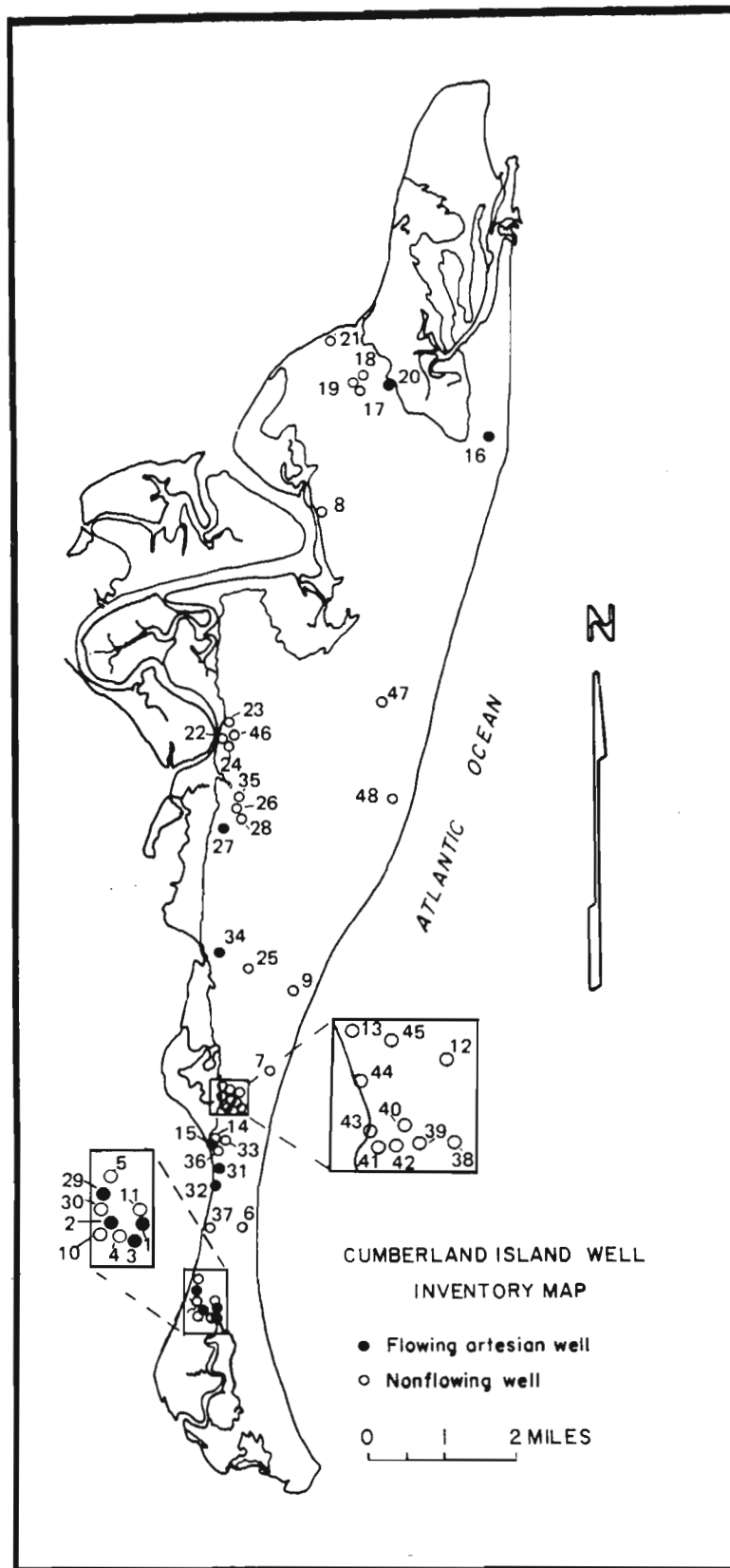
Figure 5-1. Cumberland Island well inventory map.
