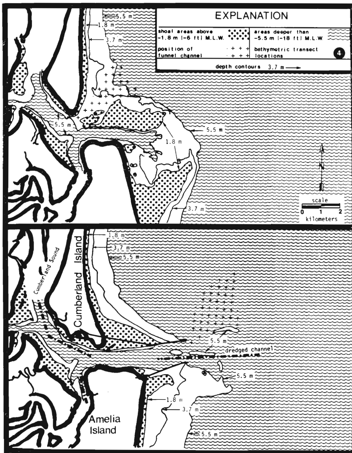
Figure 8-12. Configuration of St. Marys Entrance and Cumberland Sound, Georgia prior to the construction of the jetties, 1876 (upper figure) and present configuration, 1976 (lower figure).
