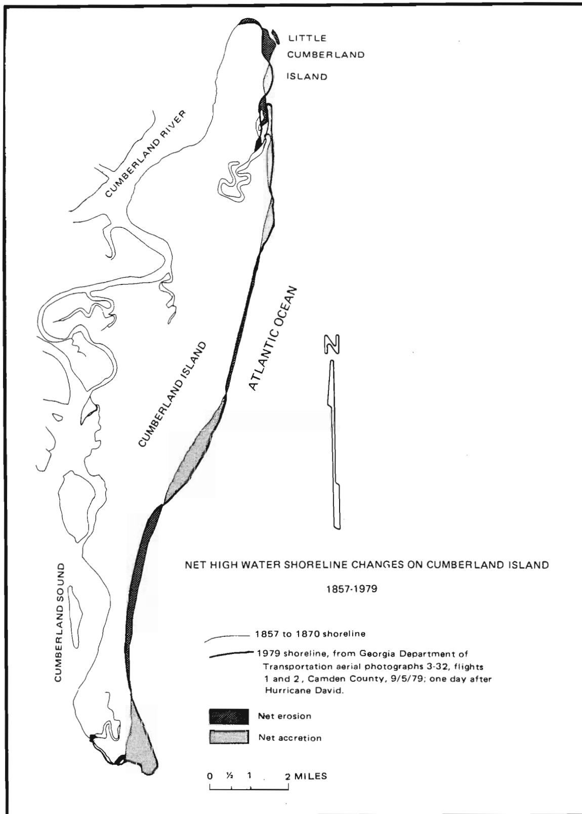
Figure 8-8. Map of net shoreline changes on Cumberland Island from 1857-1979.
