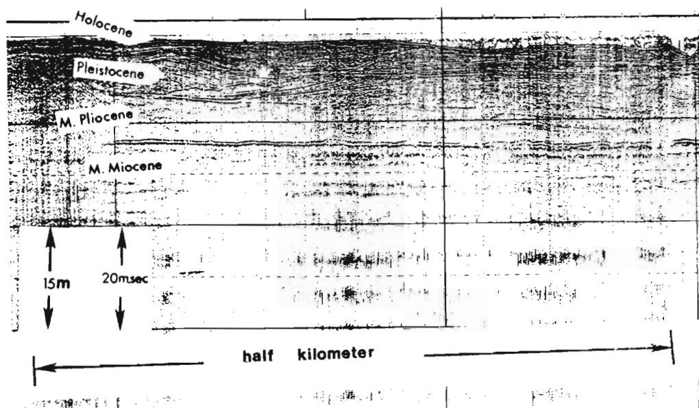
Figure 4-12. Seismic profile in Beach Creek (seismic line 188), 1 km southeast of Dungeness, showing Holocene channel deposits unconformably overlying bedded sediments of back barrier facies of Pleistocene age. A strong reflector defines the boundary between the middle Miocene and middle Pliocene sediments.
