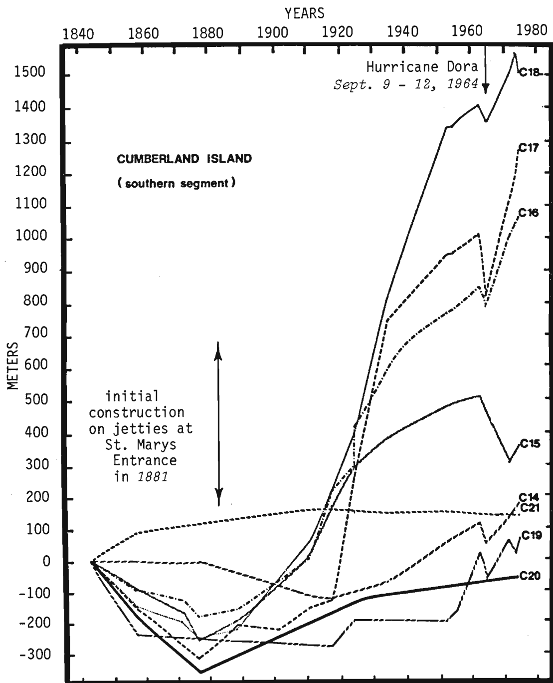
Figure 8-3. Cumulative changes in the M.H.W. shoreline on the south end of Cumberland Island, Georgia between 1843 and 1974. C14 through C21 refer to transect locations on Cumberland Island shown in figure 8-1.
