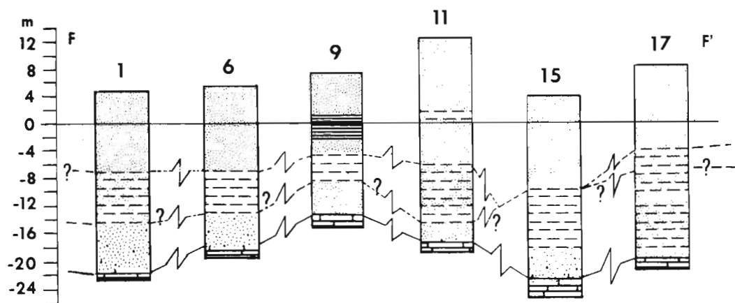
COLUMNAR SECTIONS OF WELLS SHOWING CORRELATION OF LITHOLOGIES
