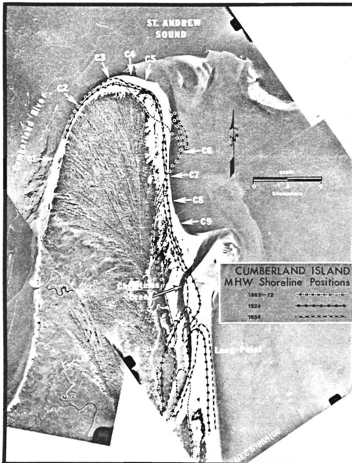
Figure 8-4. M.H.W. shoreline changes in the north end of Cumberland Island, Georgia. C1 through C9 refer to transect locations. U.S. C&GS aerial photograph taken in 1965.
