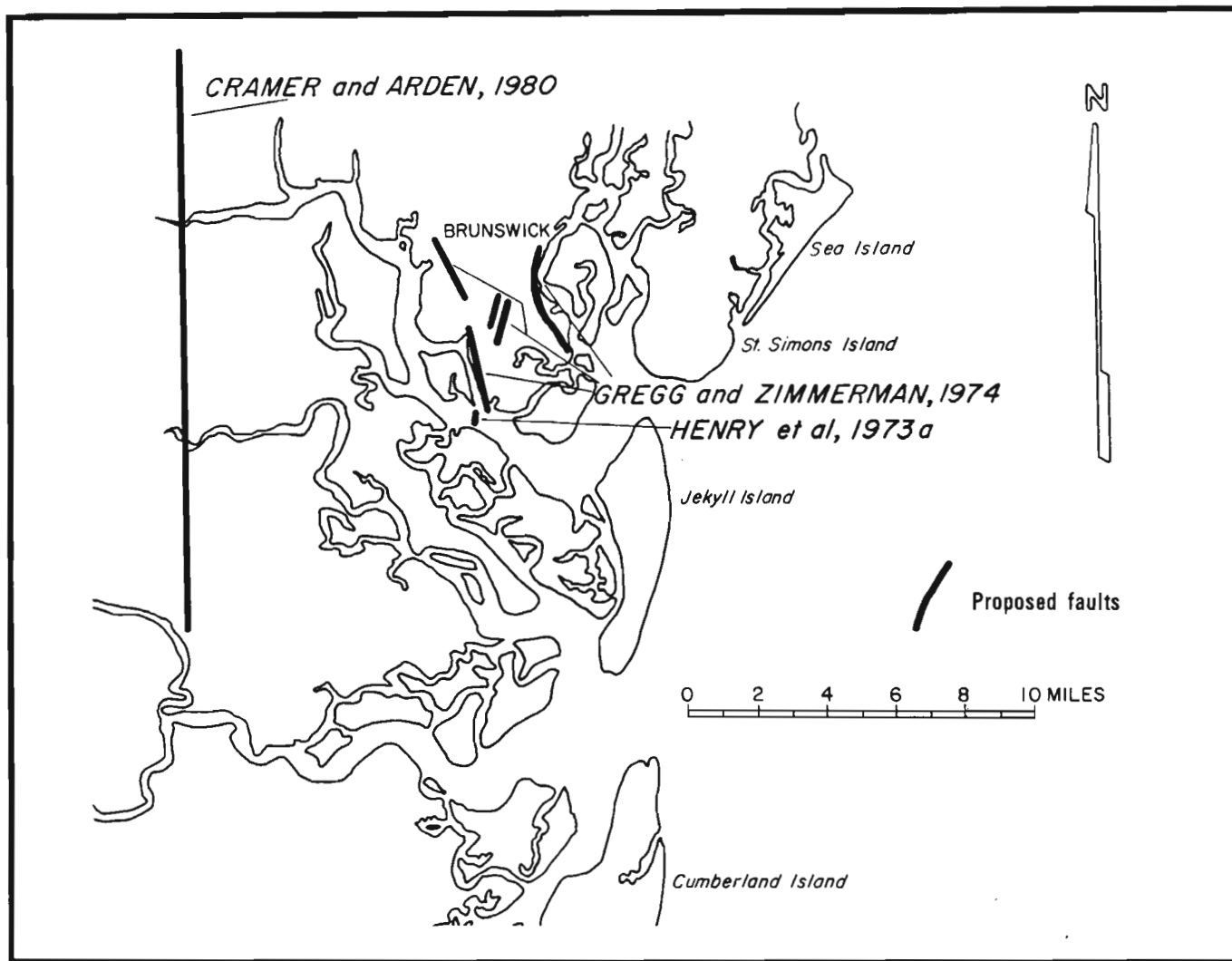
Figure 3—3. Geologic structure proposed in the Cumberland Island region.
