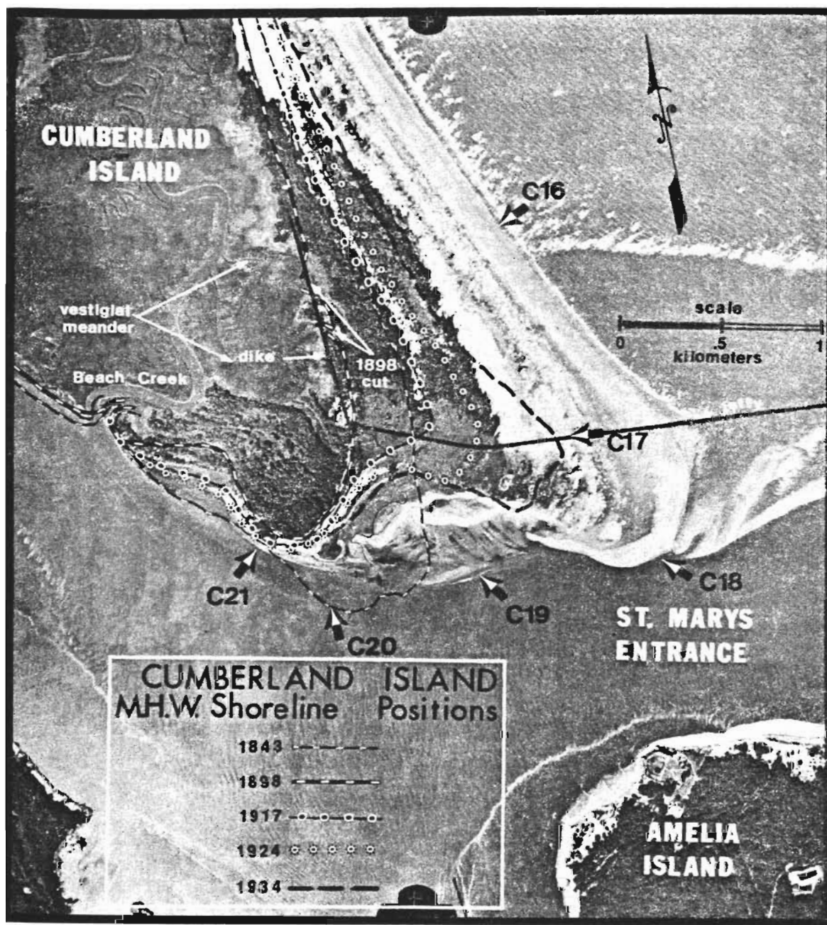
Figure 8-6. M.H.W. shoreline changes on the south end of Cumberland Island, Georgia. C16 through C21 refer to transect locations. U.S. National Ocean Survey aerial photograph taken in 1971.
