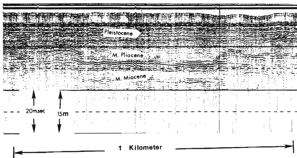
Figure 4-15. Seismic profile in southern end of the seismic line 171, showing karst. Quaternary deposit overlies coarse material of the Duplin Formation (middle Pliocene). The latter deposits overlie an irregular surface developed by karstification on the limestone (middle Miocene).
