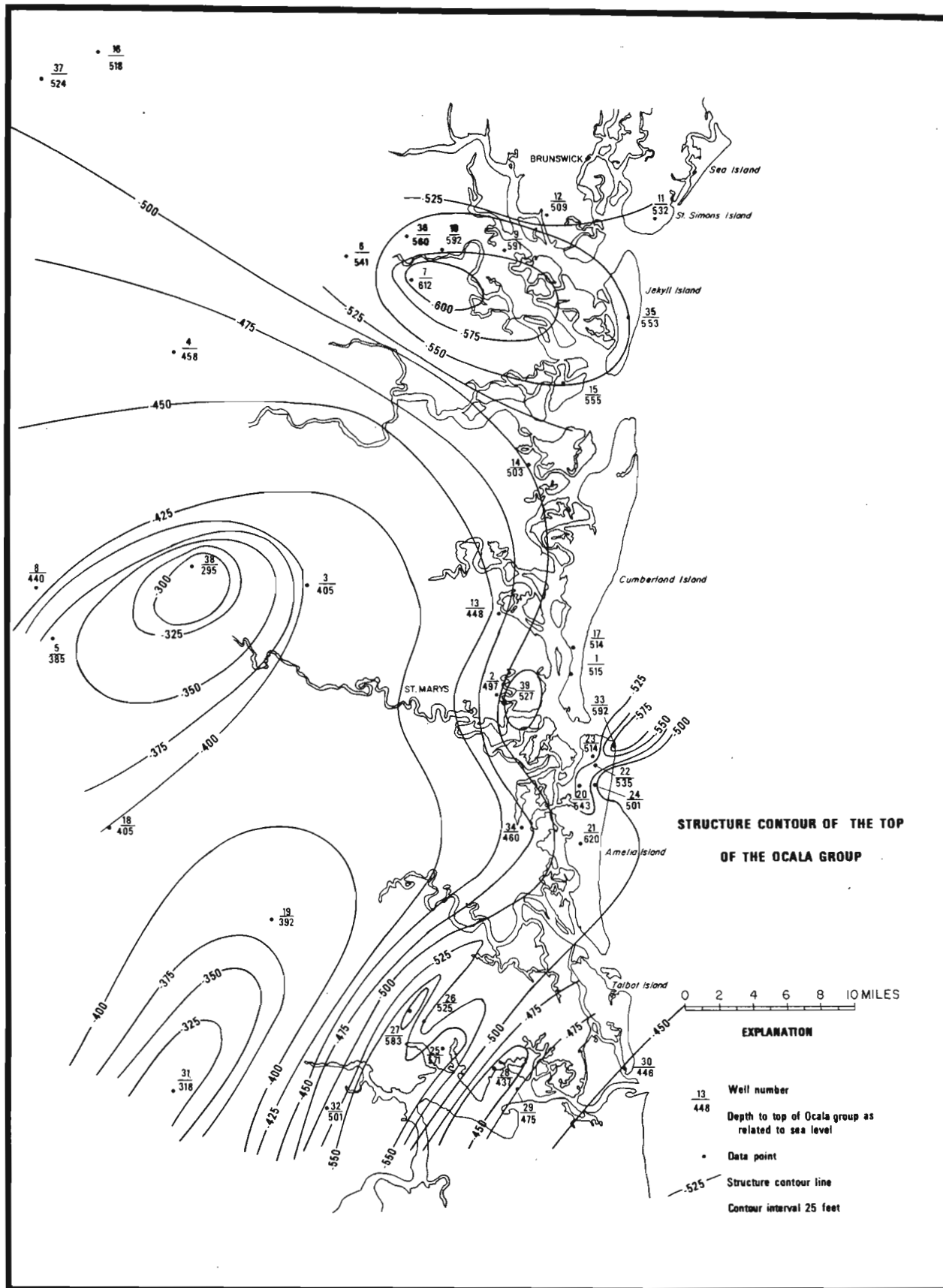
Figure 3-2. Structure contour of the top of the Ocala Group.
