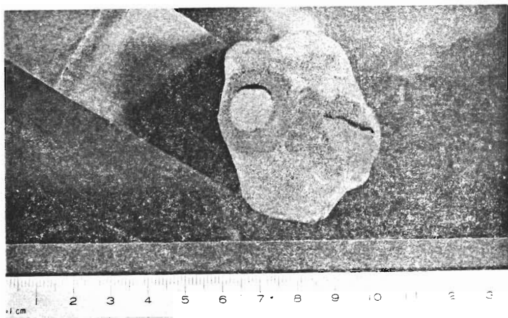
Figure 4-8. Ophiomorpha nodosa burrow in boring 3, at 7 m below surface, illustrating well-preserved wall structure. Note smooth mud in the interior surface of burrow.
