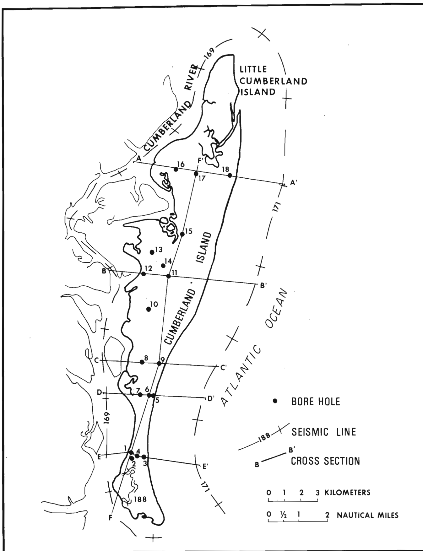
Figure 4-1. Bore hole, seismic line, and cross section locations, Cumberland Island, Georgia.
