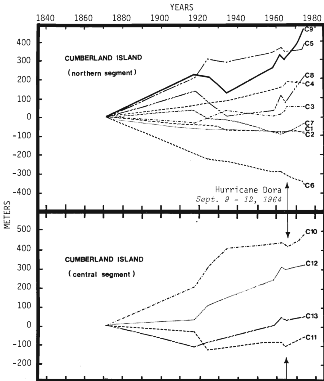
Figure 8-2. Cumulative changes in the M.H.W. shoreline of Cumberland Island, Georgia between 1871 and 1974. C1 through C13 refer to transect locations on Cumberland Island shown in figure 8-1.
