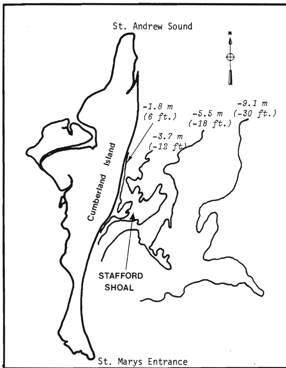
Figure 8-14. Configuration of Stafford Shoal off Cumberland Island, Georgia. Bathymetric data from 1924 hydrographic survey.
