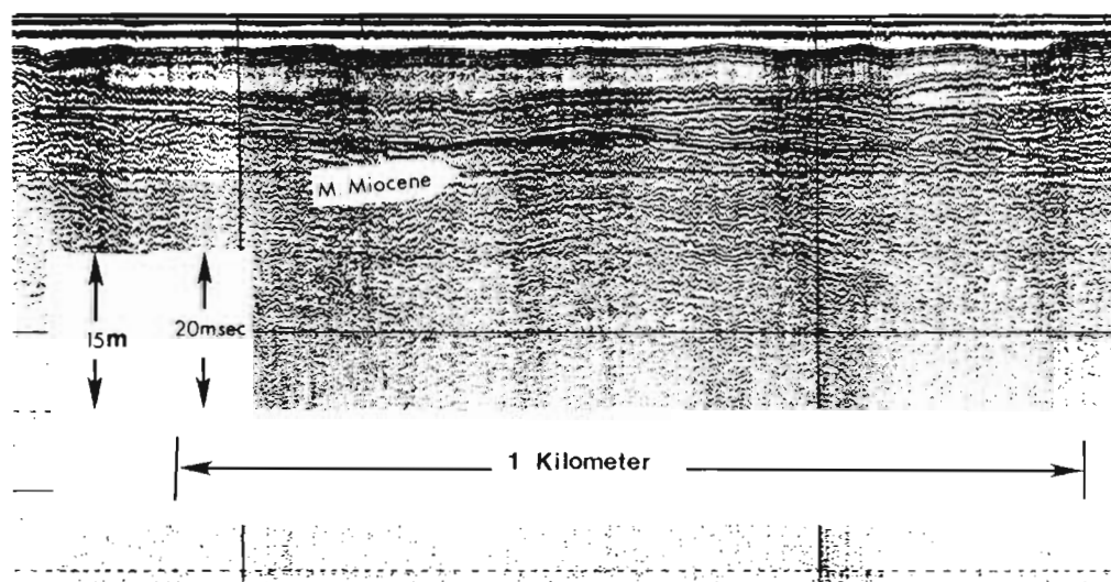
Figure 4-13. Seismic profile in Cumberland River (seismic line 169), in front of Stafford Island. Reworked sediments of Pliocene-Holocene age directly overlie the middle Miocene Charlton limestone.
