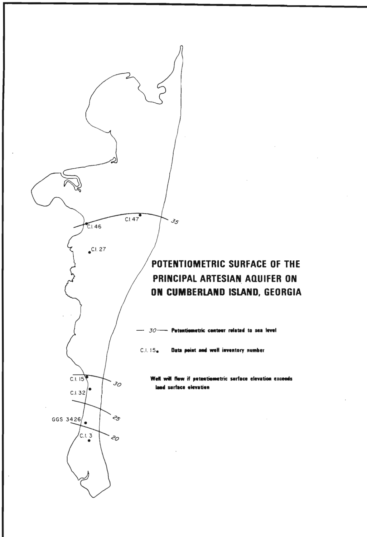
Figure 5—2. Map of the potentiometric surface of the Principal Artesian Aquifer on Cumberland Island, Georgia.
