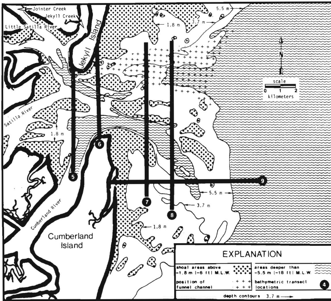
Figure 8-9. Present configuration of St. Andrew Sound and ebb-tidal delta, 1976.
