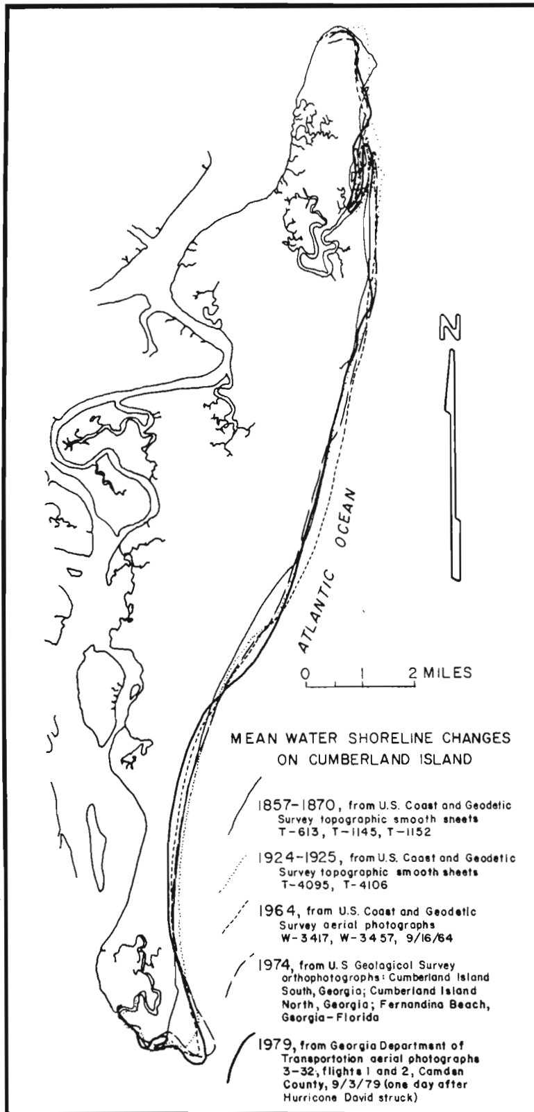
Figure 8-7. Map of shoreline changes on Cumberland Island from 1857-1979.
