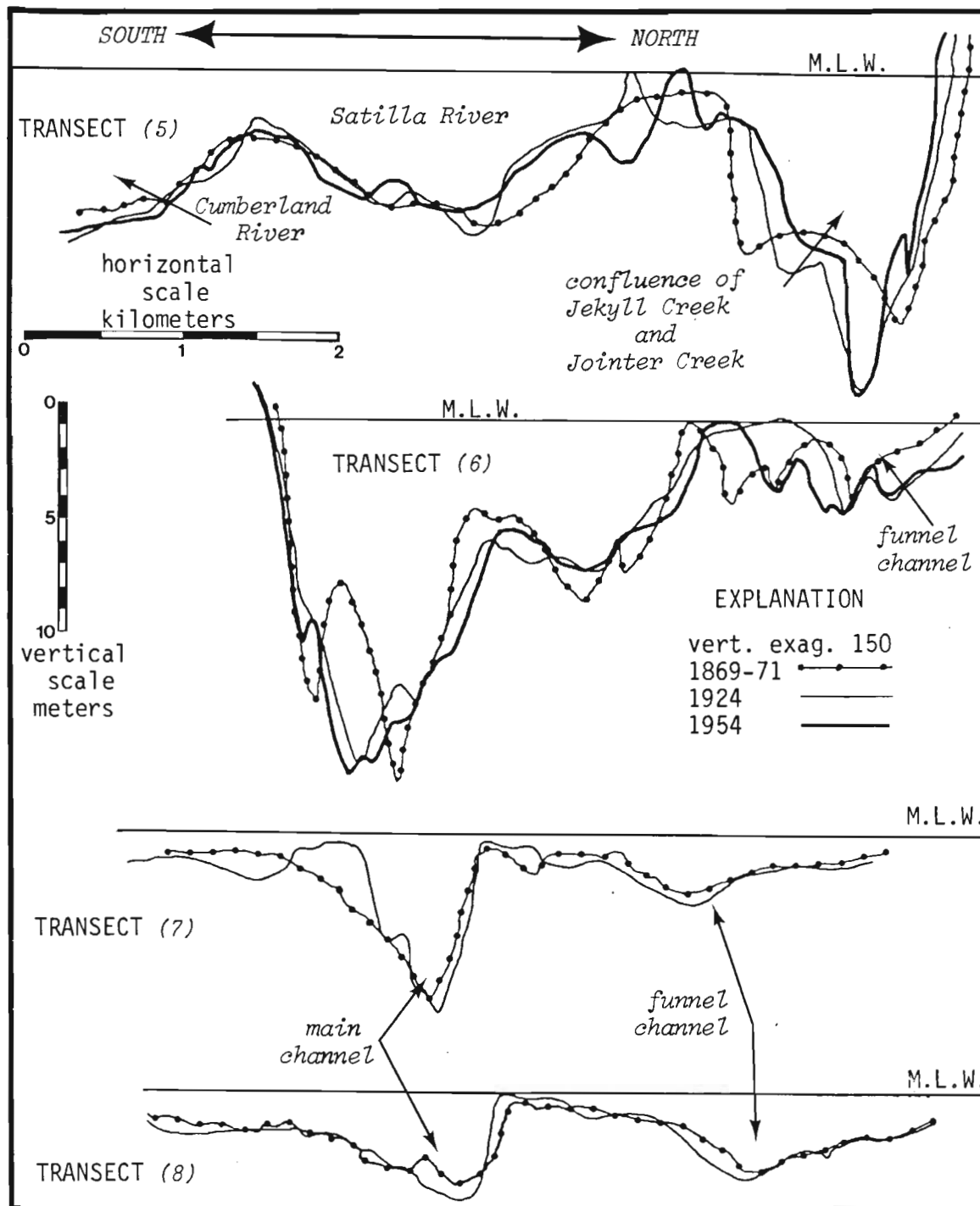
Figure 8-10. Bathymetric profiles taken at transects off St. Andrew Sound, Georgia. Transect locations are shown in figure 8-9.
