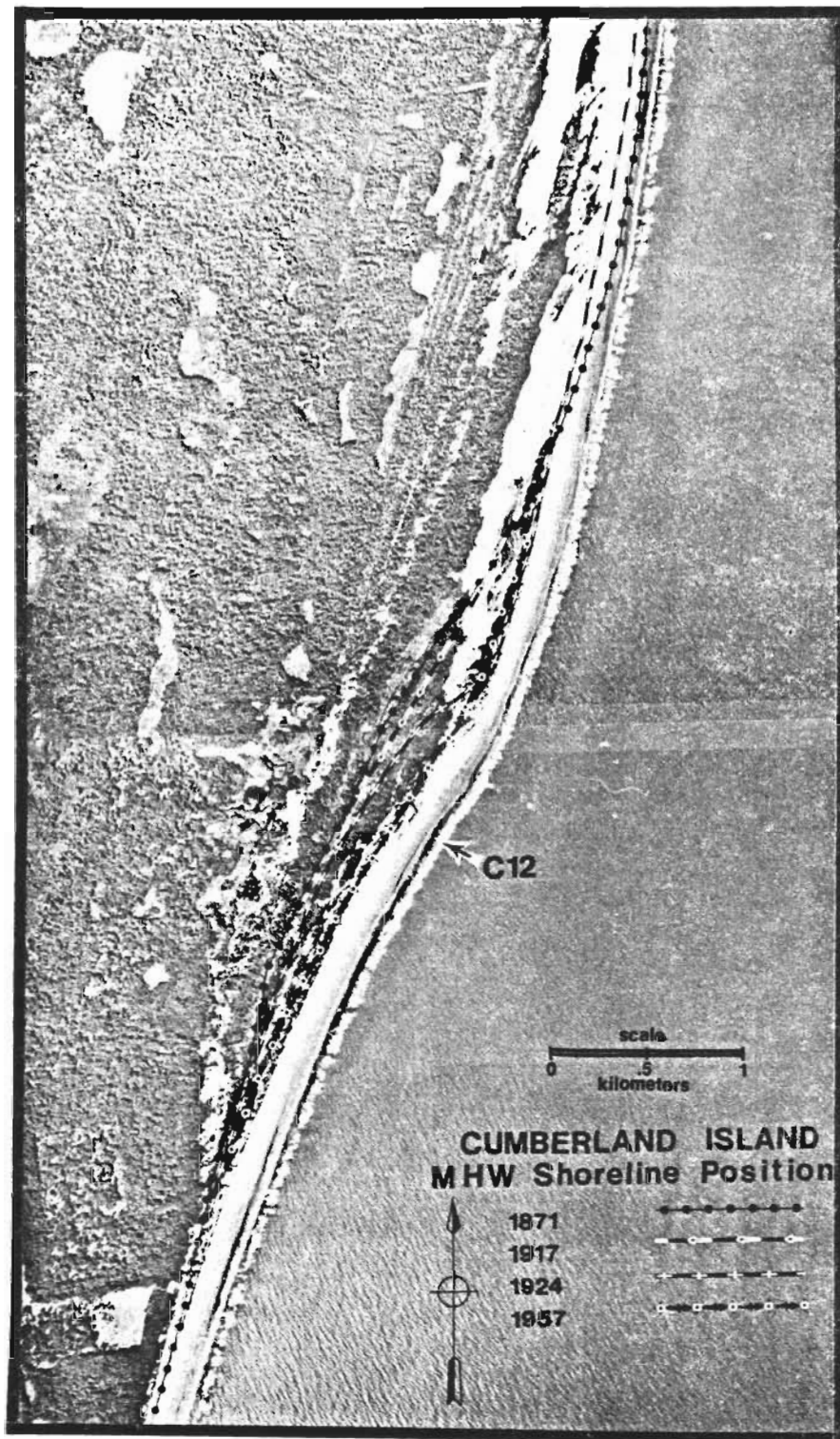
Figure 8-5. M.H.W. shoreline changes in the central part of Cumberland Island, Georgia. C12 refers to a transect location. U.S. C&GS aerial photograph taken in 1962.
