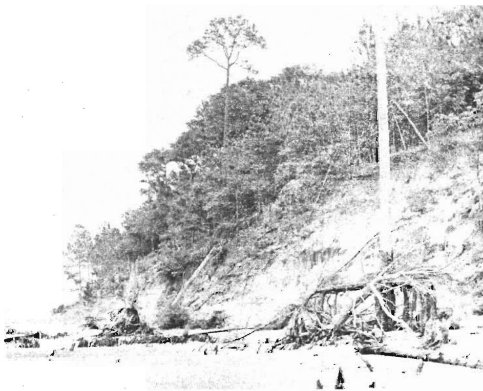
Figure 4-9. Cumberland Island Wharf outcrop. Pleistocene barrier island deposits (foreshore facies) on 12 m high erosional scarp.
