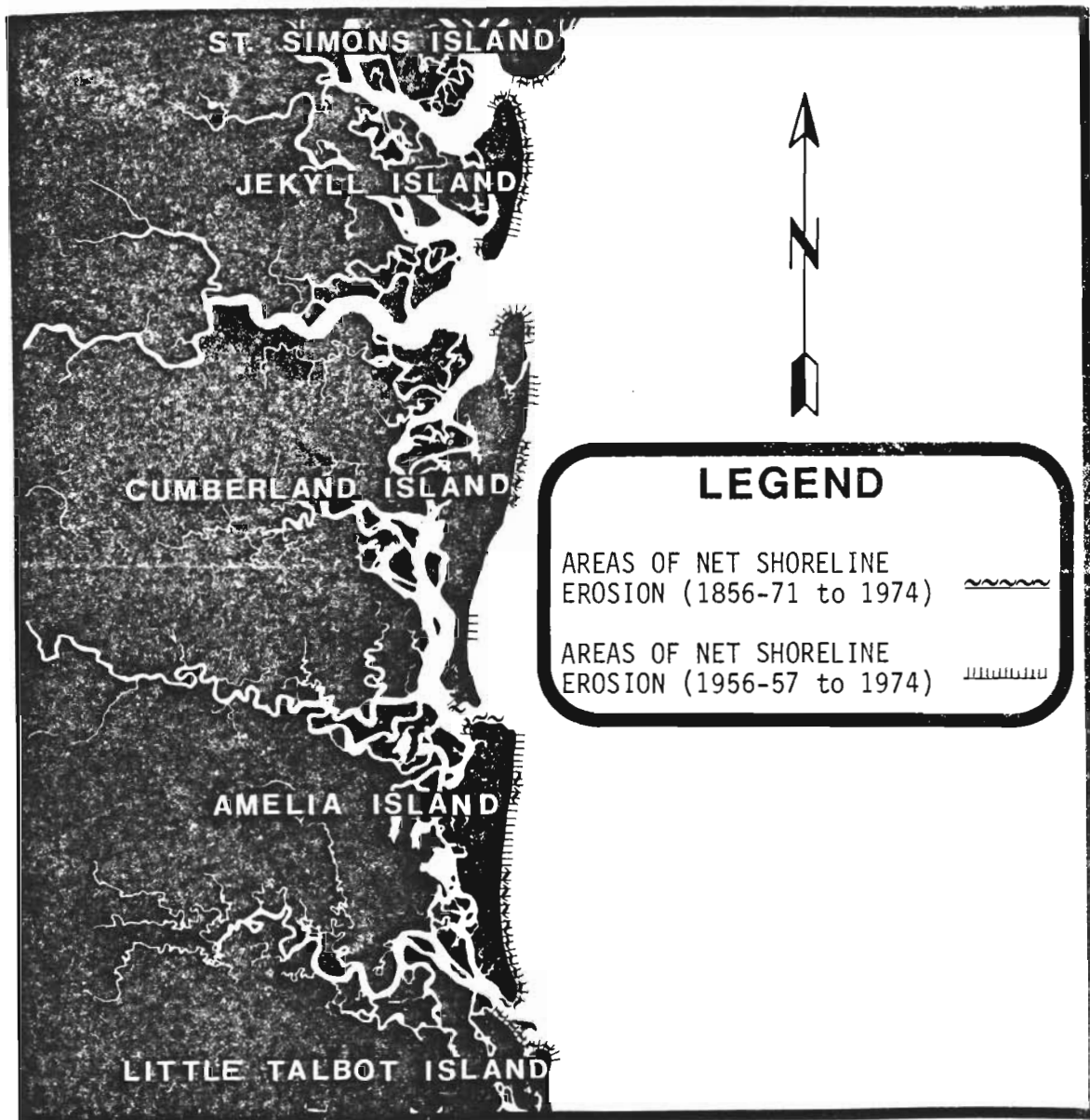
Figure 8-13. Coastal areas of south Georgia and north Florida showing sections of shoreline which have undergone long term and recent net erosion.
