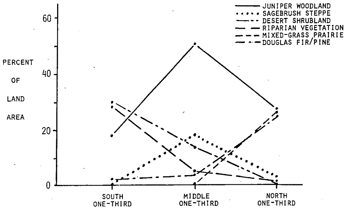
Fig. 2. The percent land area in different vegetation types in the southern, middle, and northern thirds of the BCNRA. The changes can be attributed to topographic differences, the somewhat higher elevations in the middle third, and the change in annual precipitation from 18 cm in the south to 49 cm in the north.
