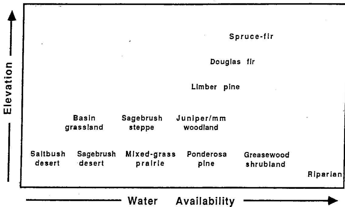
Fig. 9. The hypothesized relationships between water availability, elevation, and the major vegetation types of the BCNRA. The elevation gradient extends from approximately 1100 to 2600 m (3630 to 8580 ft). See text for explanation.
