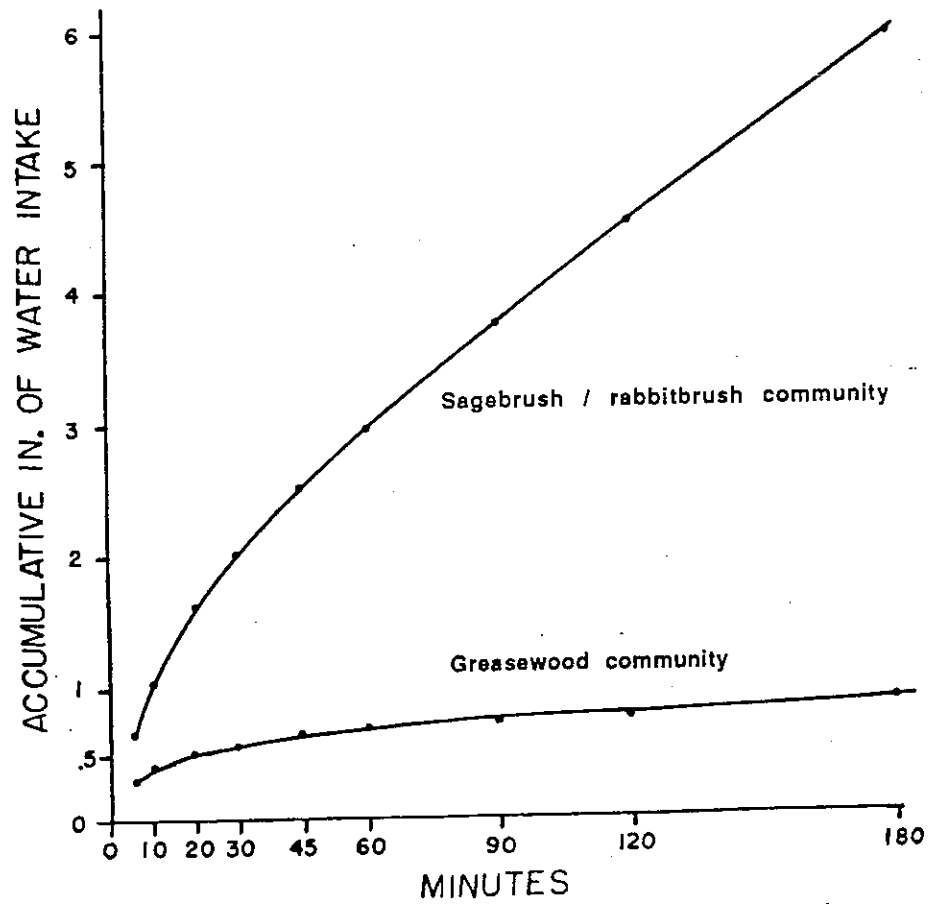
Fig. 5. Data which show how greasewood desert shrubland in the Big Horn Basin has a lower soil infiltration capacity than a stand dominated by big sagebrush and rabbitbrush. The vertical axis is accumulative inches of water intake (1 inch = 2.54 cm). From a study by Nichols (1964a) done near Worland. See Fig. 4 also.
