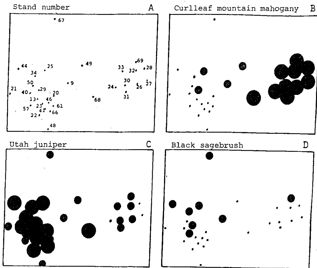
Fig. 8. An ordination of 30 stands of woodlands dominated by Utah juniper and/or curleaff mountain mahogany. Stands are identified by number in part A. Stands located close together are very similar in species composition, those located far apart are very different. The percent cover of individual species is shown in parts B, C, and D, with a small dot indicating a cover of 0-1%, a medium dot indicating 1-10%, and a large dot indicating greater than 10% cover. The stands on the right are dominated by mountain mahogany (B), those on the left by Utah juniper (C). Fendler three-awn and grass cover were also higher in stands with relatively high juniper cover. The black sagebrush pattern is shown in D. See text for additional information on the juniper/mountain mahogany woodlands of the BCNRA.
