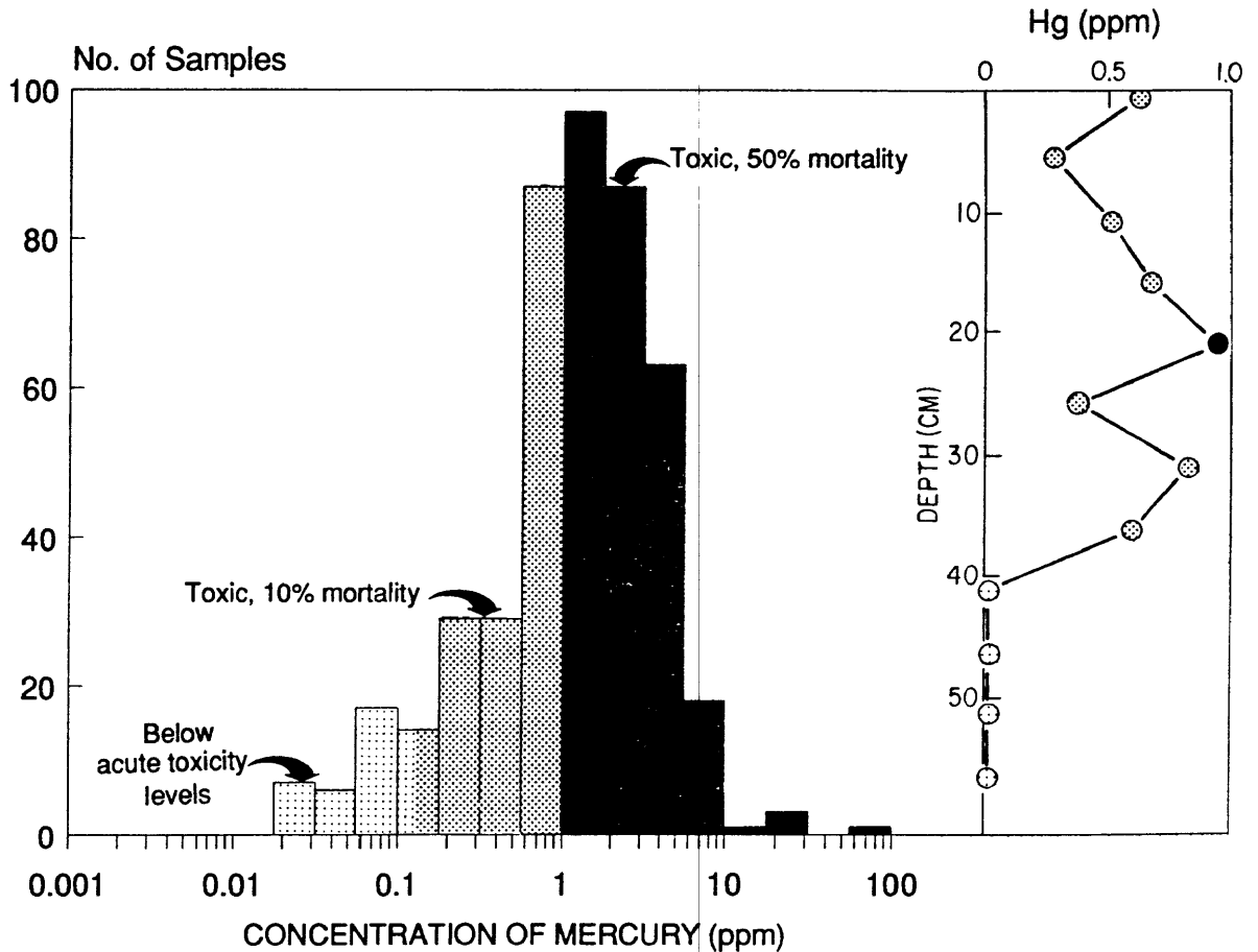
Figure 18. Histogram of the concentration of mercury in the surficial sediments in Boston Harbor. The Overall Apparent Effects Threshold of pollutant concentration (50% mortality) in sediment for consistent toxic effects on organisms is listed by Long and Morgan (1990). The profile of mercury in the sediment at one location in Boston Harbor (right panel) shows elevated concentrations in the upper 40 cm of the sediment column (data of M.H. Bothner).
