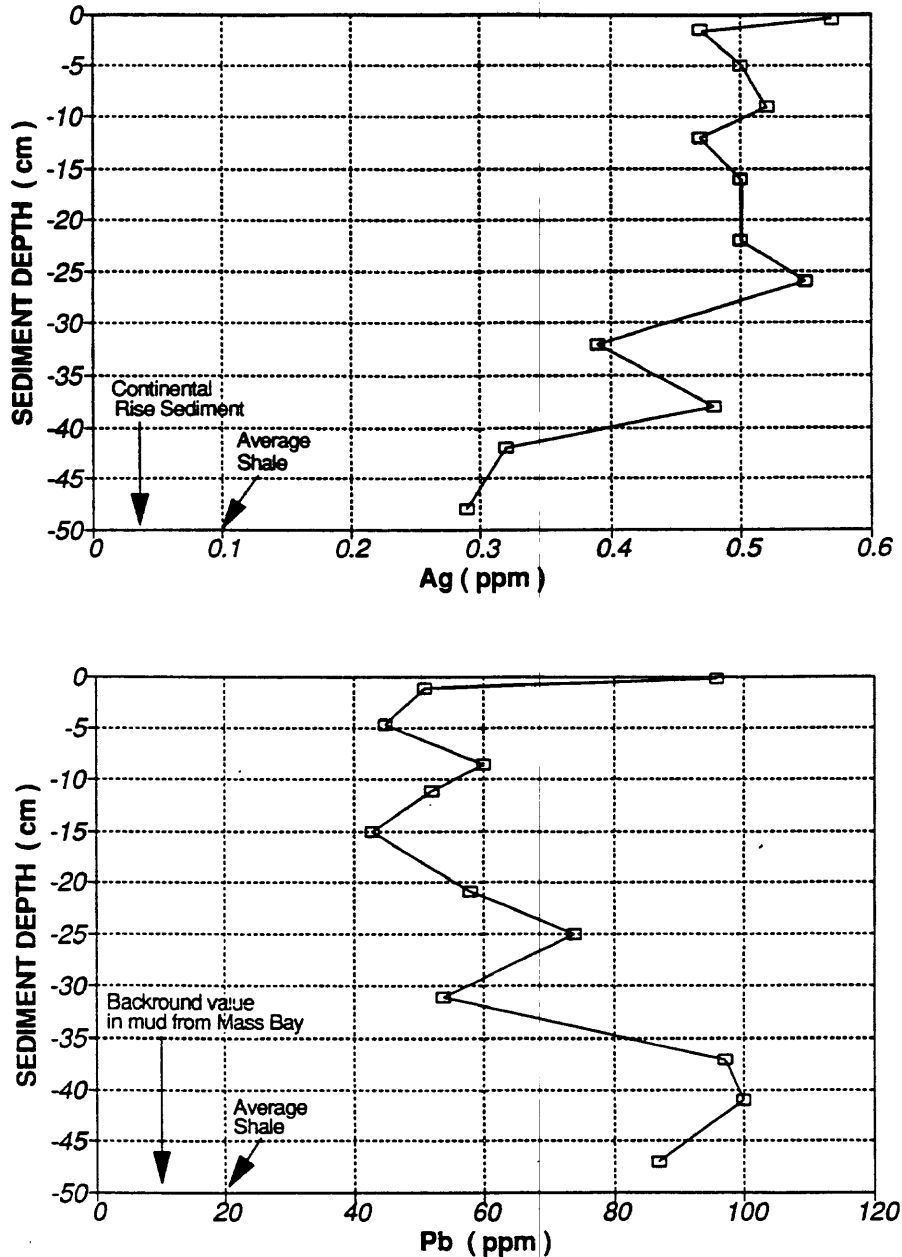
Figure 13. Top: Concentrations of silver vs. sediment depth at station 3 (fig. 5). Background concentrations of silver in muddy sediments from the Continental Rise are 0.04 ppm. The concentrations in world average shale is 0.1 ppm. The maximum concentrations of silver in this core (0.57 ppm) are 6 times higher than average shales and 14 times higher than sediments from the Continental Rise. Bottom: Concentrations of lead vs. sediment depth at station 3 (fig. 5). Background concentrations in fine-grained sediments from Massachusetts Bay are about 13 ppm. The subsurface concentration of lead (100 ppm) at 42 cm may be due to deep biological mixing or to direct dumping of waste material at this location. Glass fragments and slag have been found at depth in some cores from this location.
