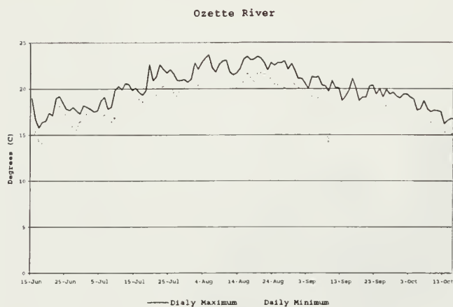
Figure 9. Daily maximum and minimum water temperatures in the Lake Ozette tributaries, 1994. The thermograph probe in Big River was exposed to air sometime before August 25 and no reliable data were collected at this site prior to that date.
