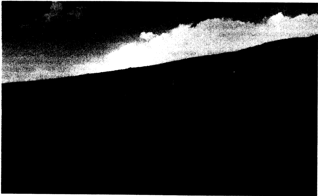
Figure 4.—Long slope of fine-textured soil which supports the Agropyron smithii / Carex filifolia habitat type.
