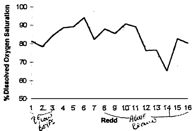
Figure 11. Percent dissolved oxygen saturation for 16 coho redds in Prairie Creek, Humboldt County, California, 1997.
