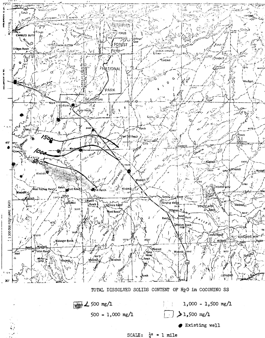
Figure 8. Map showing increasing conductivity of groundwater in the Coconino Aquifer northward from the Little Colorado River (from Witucki, 1972).
