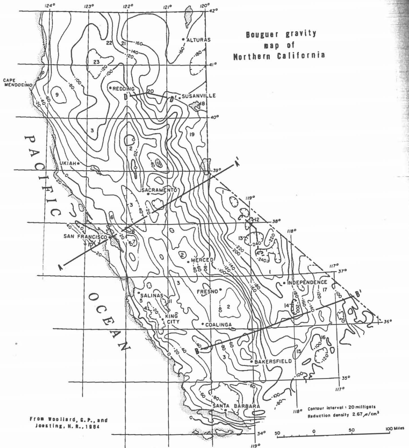
Figure 1. Bouguer gravity map of northern California (after Woollard and Joesting, 1964).
