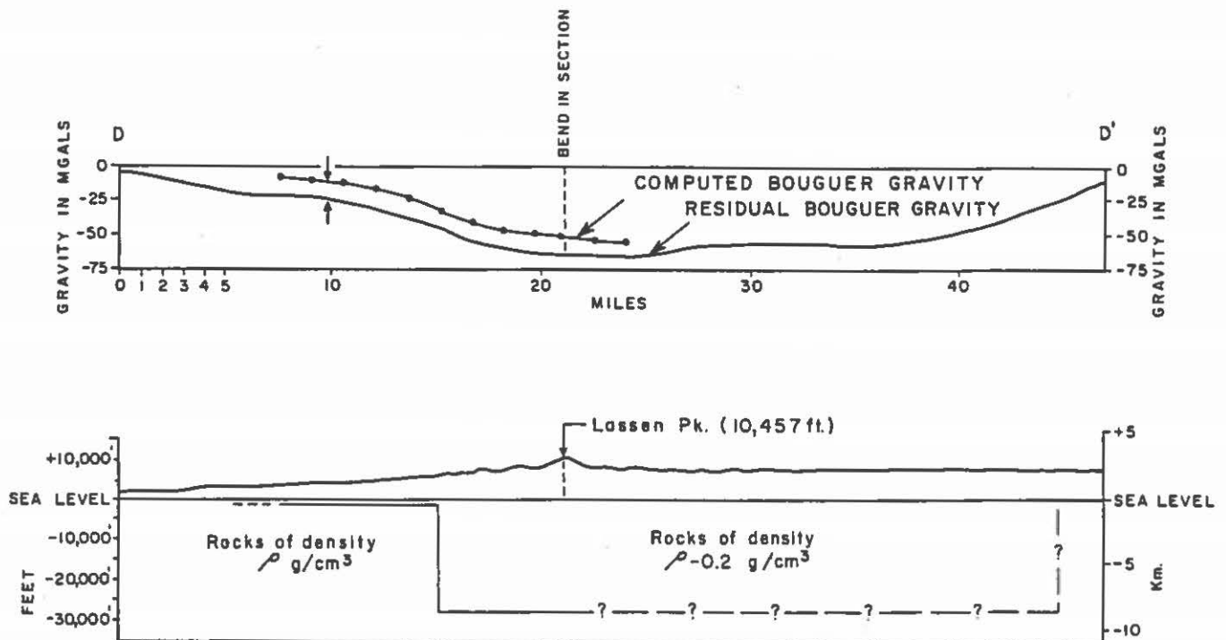
Figure 5. Bouguer gravity profile along D-D', figure 1, across Lassen Peak and the southern Cascade Range area showing assumed subsurface structure (after Pokiser, 1964, fig. 3).
