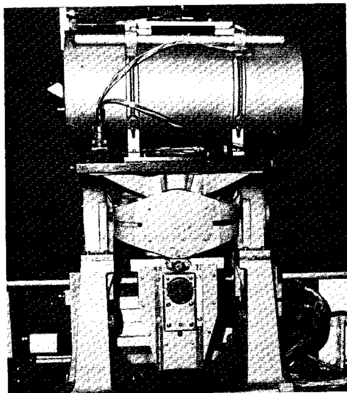
Figure 1. Graf-Askania Gss2 sea gravimeter mounted on Aero-flex gyrostabilized platform; gravimeter beam is within cylindrical drum; platform is designed to keep meter level to within 0.1
