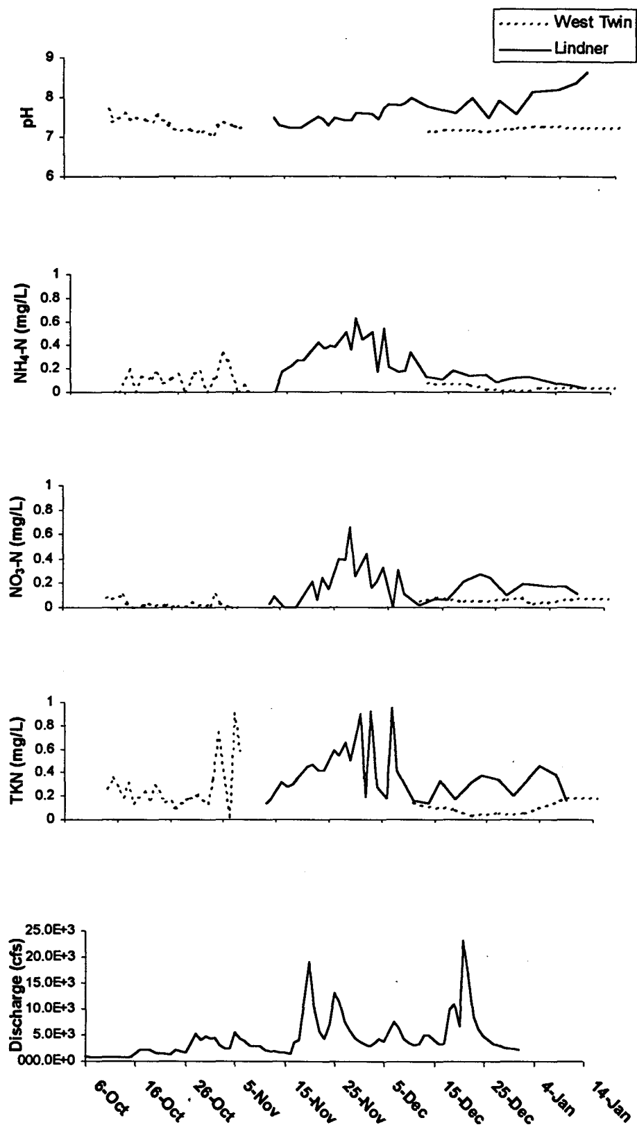
Figure 4. Nutrient analysis of 32 hour ISCO samples (a-d) and (e) Hoh River from USGS gauging station 12041200.
