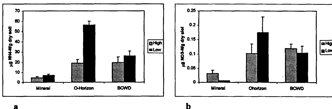
Figure 5. Extractable inorganic nitrogen in mineral soil, fine litter and BCWD from near plots 1 and 4 in the West Twin Creek watershed. a shows \text{NH}_4\text{-N} concentration \pm 1 se and b \text{NO}_3\text{-N} concentration.
