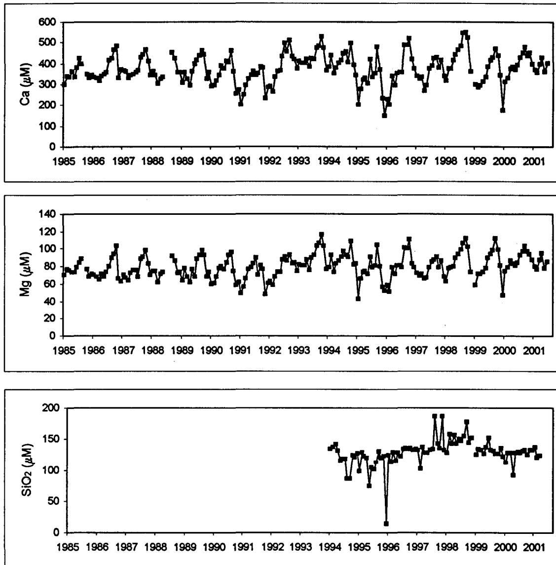
Figure 3. Multivalent cation concentration in \mu\text{M} for West Twin Creek from January 1985 – June 2001.
