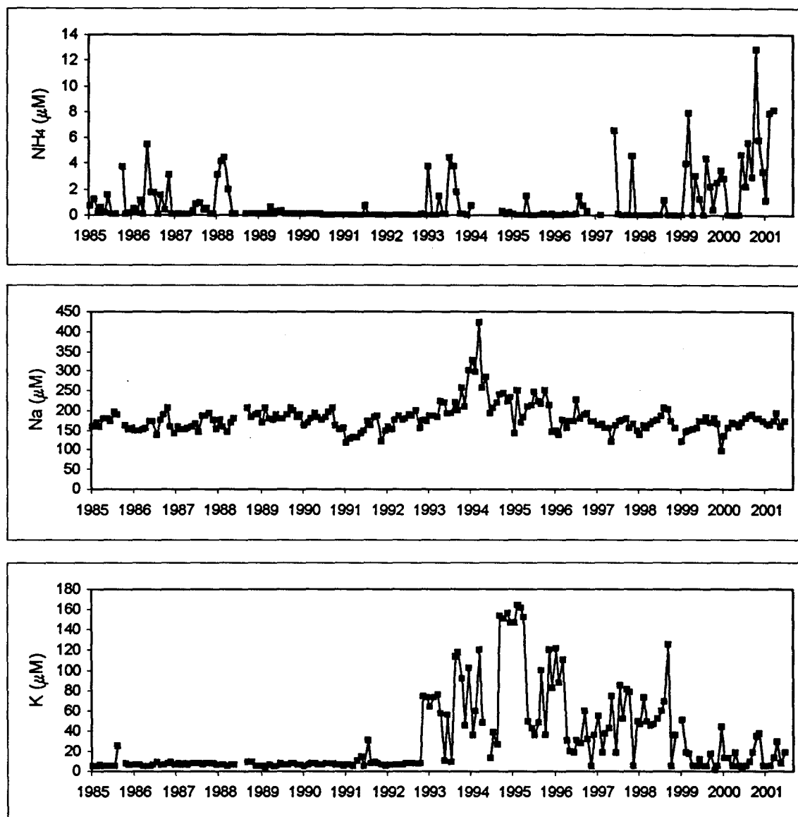
Figure 2. Monovalent cation concentration in \mu\text{M} for West Twin Creek from January 1985 – June 2001.
