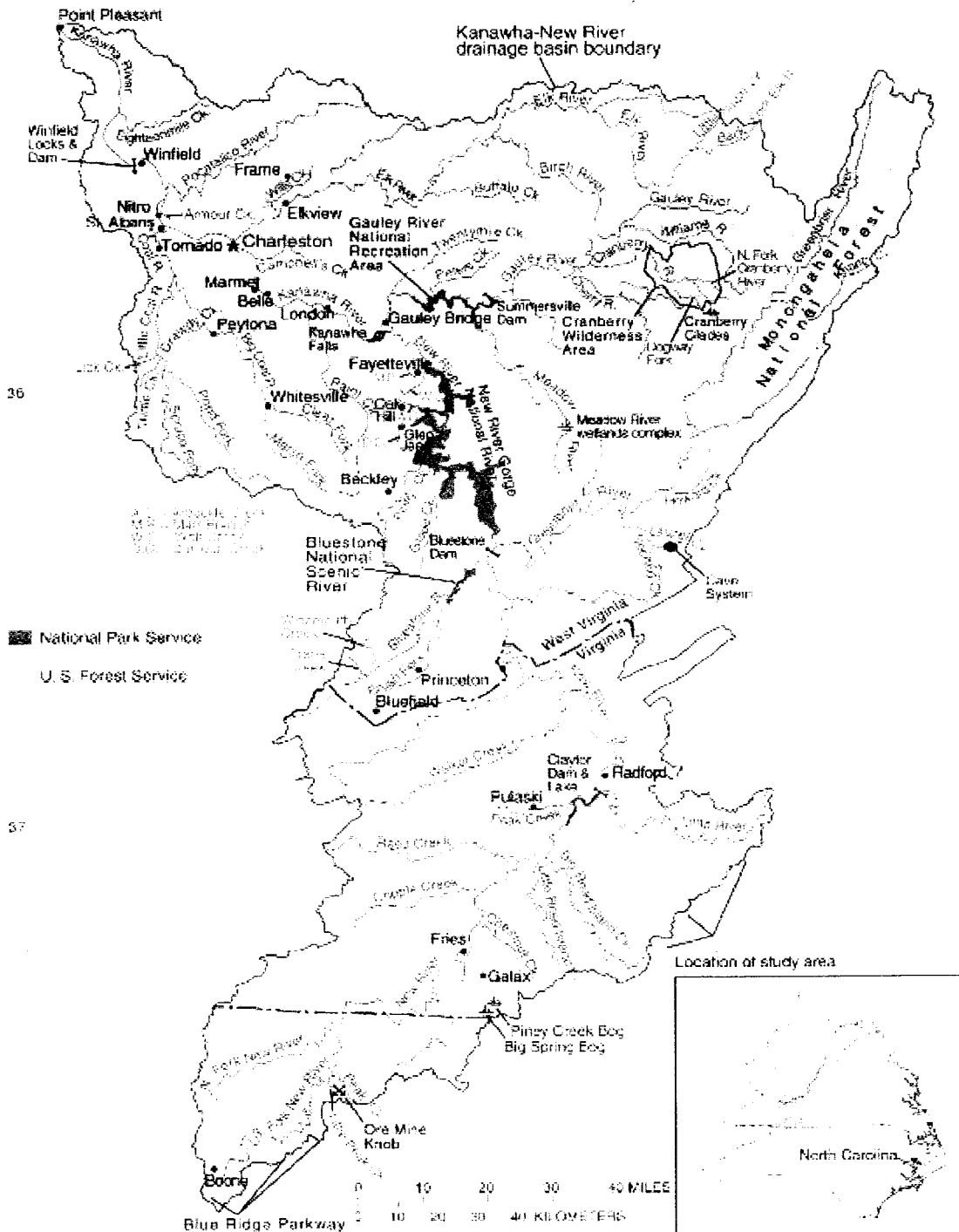
Map of the New River watershed, showing the locations of Bluestone National Scenic River, New River Gorge National River, and Gauley River National Recreation Area.
