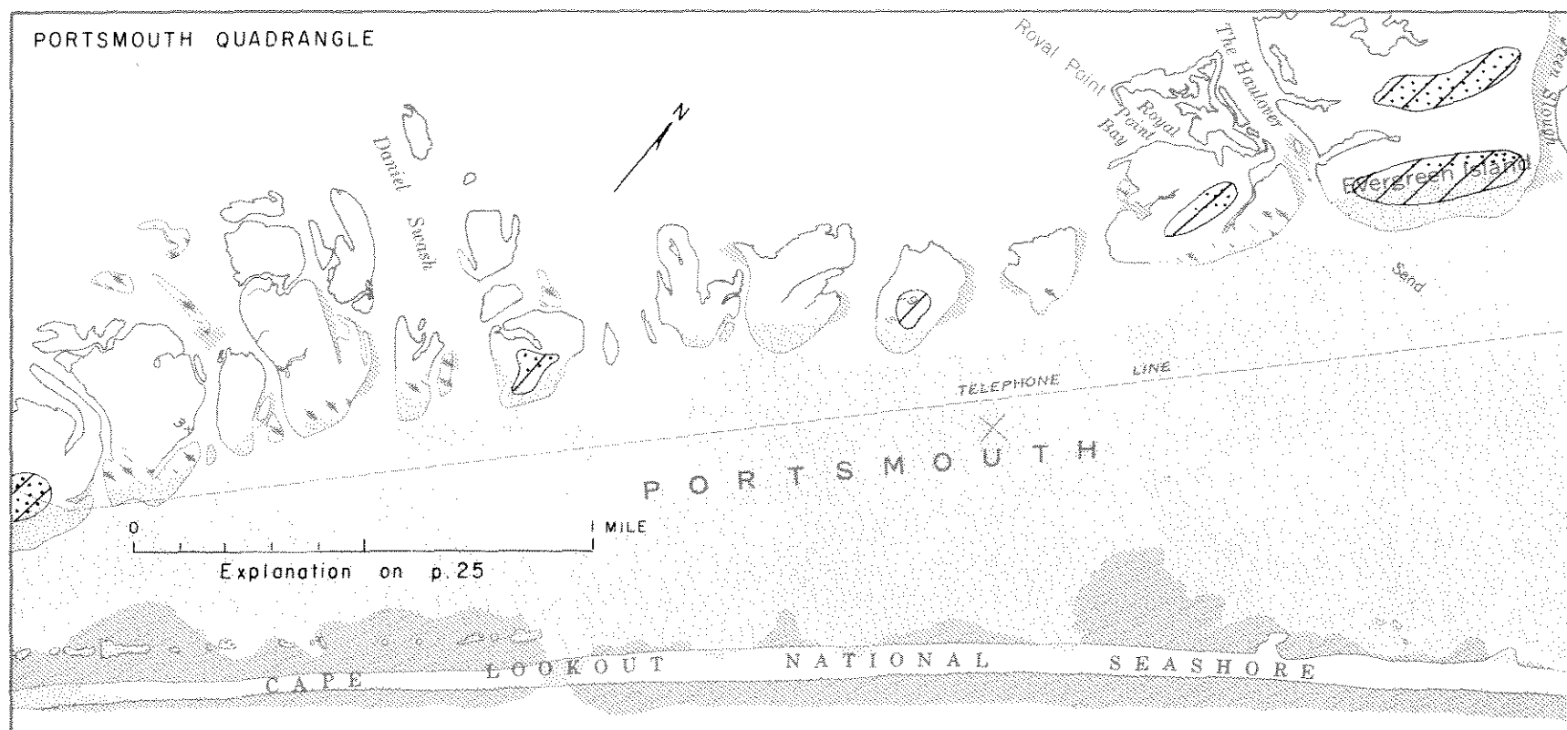
Figure 25.--Central Portsmouth Island area.
