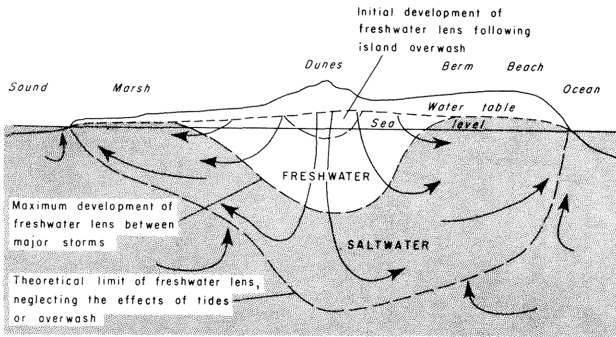
Figure 4.--Occurrence and movement of ground water and the development of a freshwater lens beneath a sandy barrier island.
