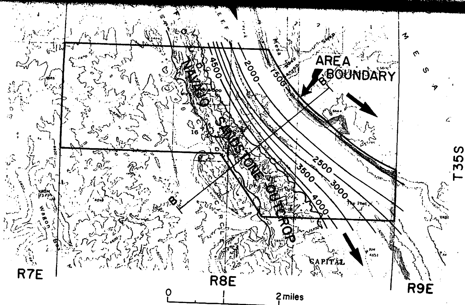
Figure 4. Elevation of the top of the Navajo Sandstone and ground water flow direction in the Ball Creek area, Capitol Reef National Park, Utah.
