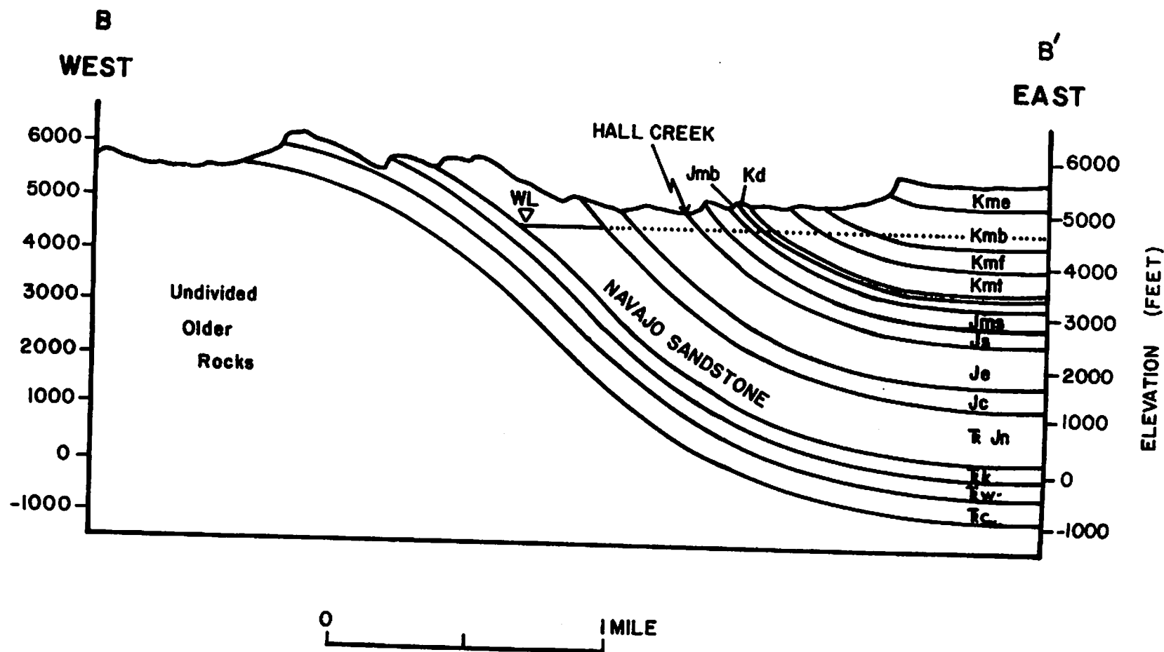
Figure 5. Structural cross section in the Hall Creek area, Capitol Reef National Park, Utah. Kme - Emery Sandstone Member, Mancos Shale; Kmb - Blue Gate Shale Member, Mancos Shale; Kmf - Ferron Sandstone Member, Mancos Shale; Kmt - Tununk Shale Member, Mancos Shale; Kd - Dakota Sandstone; Jmb - Brushy Basin Shale Member, Morrison Formation; Jms - Salt Wash Sandstone Member, Morrison Formation; Js - Summerville Sandstone; Je - Entrada Sandstone; Jc - Carmel Formation; Tr Jn - Navajo Sandstone; Tr k - Kayenta Formation; Tr w - Wingate Sandstone; Tr c - Chinle Formation; WL - water level in the Navajo Sandstone; dots indicate projection of potentiometric surface; from Harnish and others, 1964.
