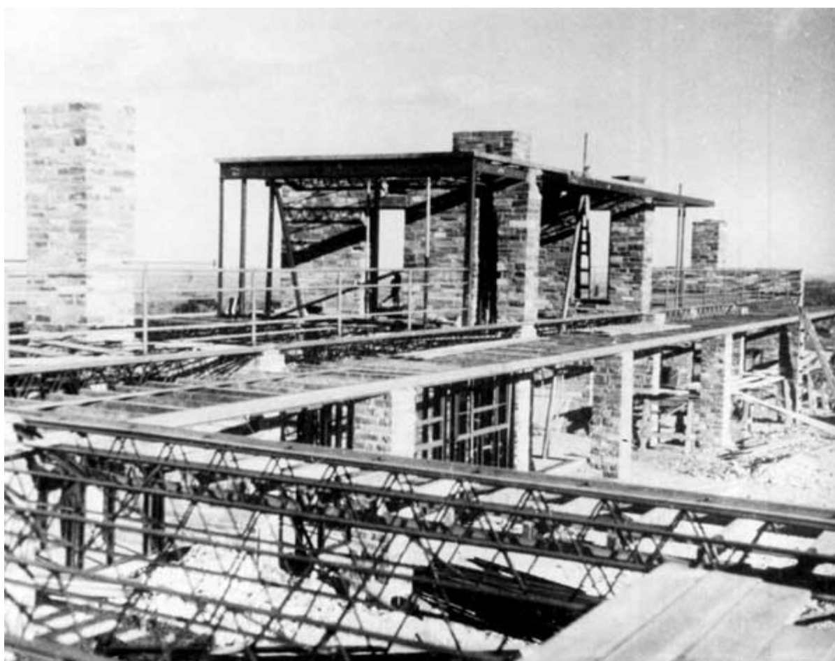
Figure 39. The Ship on the Desert during construction. The structural steel framework of the building and massive walls of natural rock are apparent. (NPS Photo)
