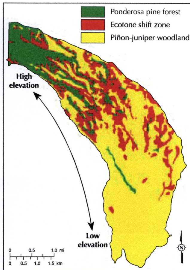
FIGURE 8—Changes in vegetation cover between 1954 and 1963 on Frijolito Mesa in Bandelier National Monument, showing persistent ponderosa pine forest (1.4 \text{mi}^2 ), persistent piñon-juniper woodland (5.9 \text{mi}^2 ), and the ecotone shift zone (1.9 \text{mi}^2 ) where forest changed to woodland due to the death of the overstory ponderosa pine trees.
