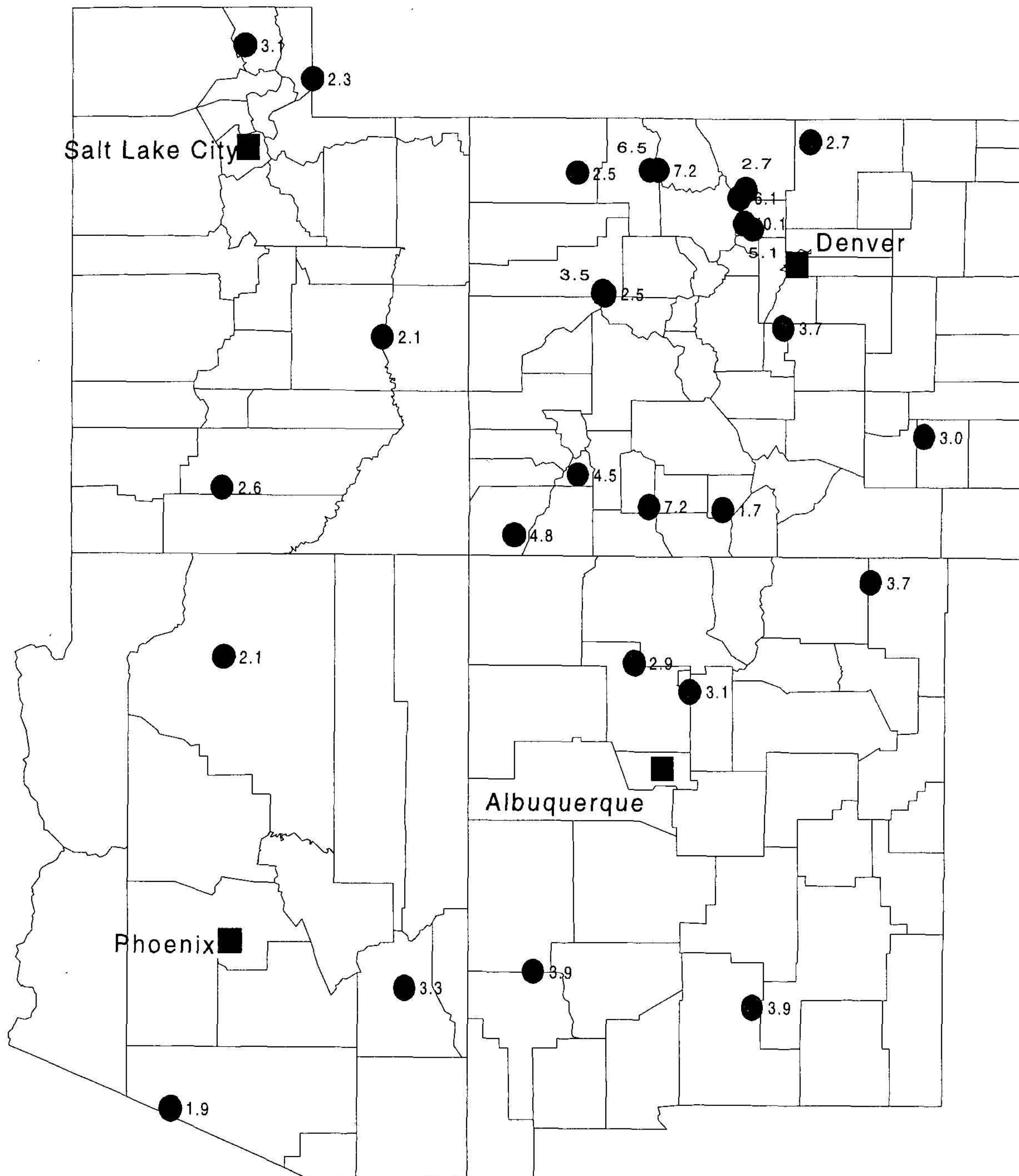
Figure 1-11. Sulfate deposition ( \text{SO}_4^{2-} ; multiply by 0.333 for S only) for the Colorado Plateau and surrounding areas. Dots represent NADP monitoring sites, squares are major cities (data from NADP, Colorado State University).
