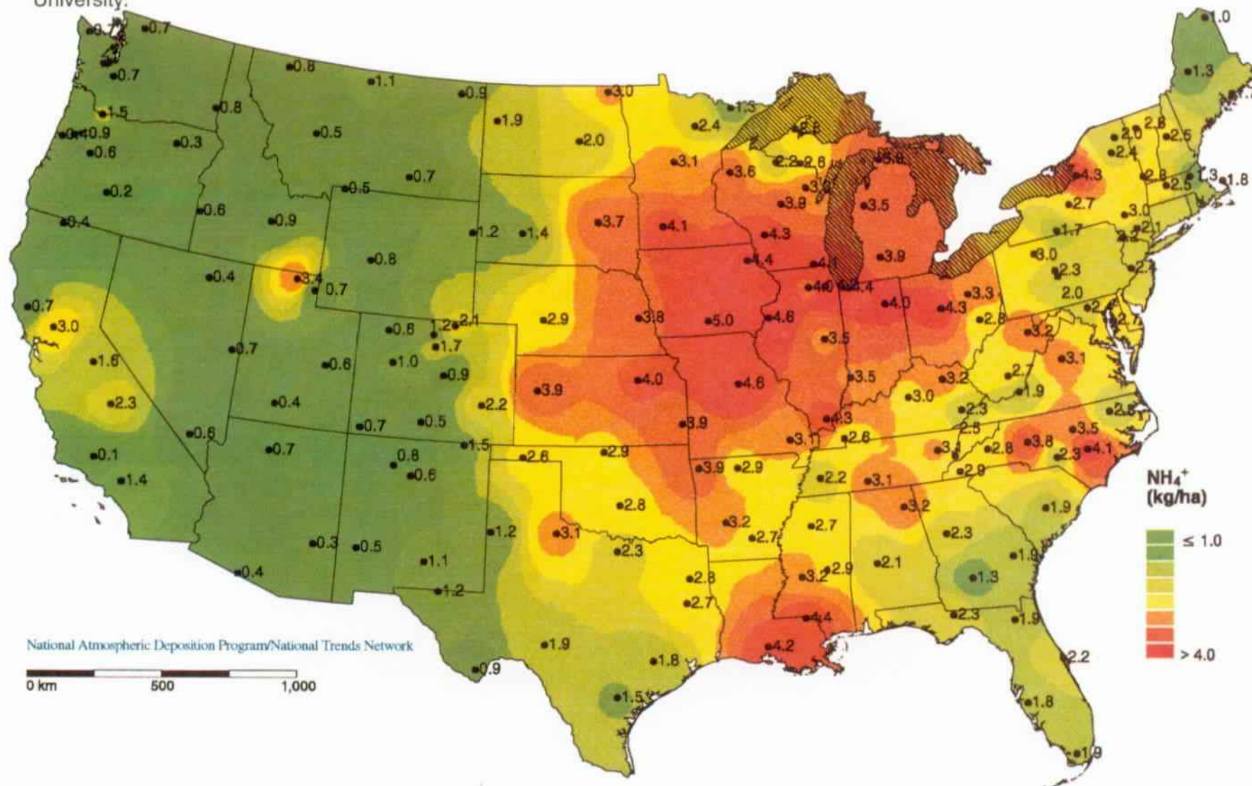
Figure 1-8. Ammonium deposition ( \text{NH}_4^+ ; multiply by 0.778 for N only) for the U.S. for 1995 (map provided by NADP, Colorado State University).
