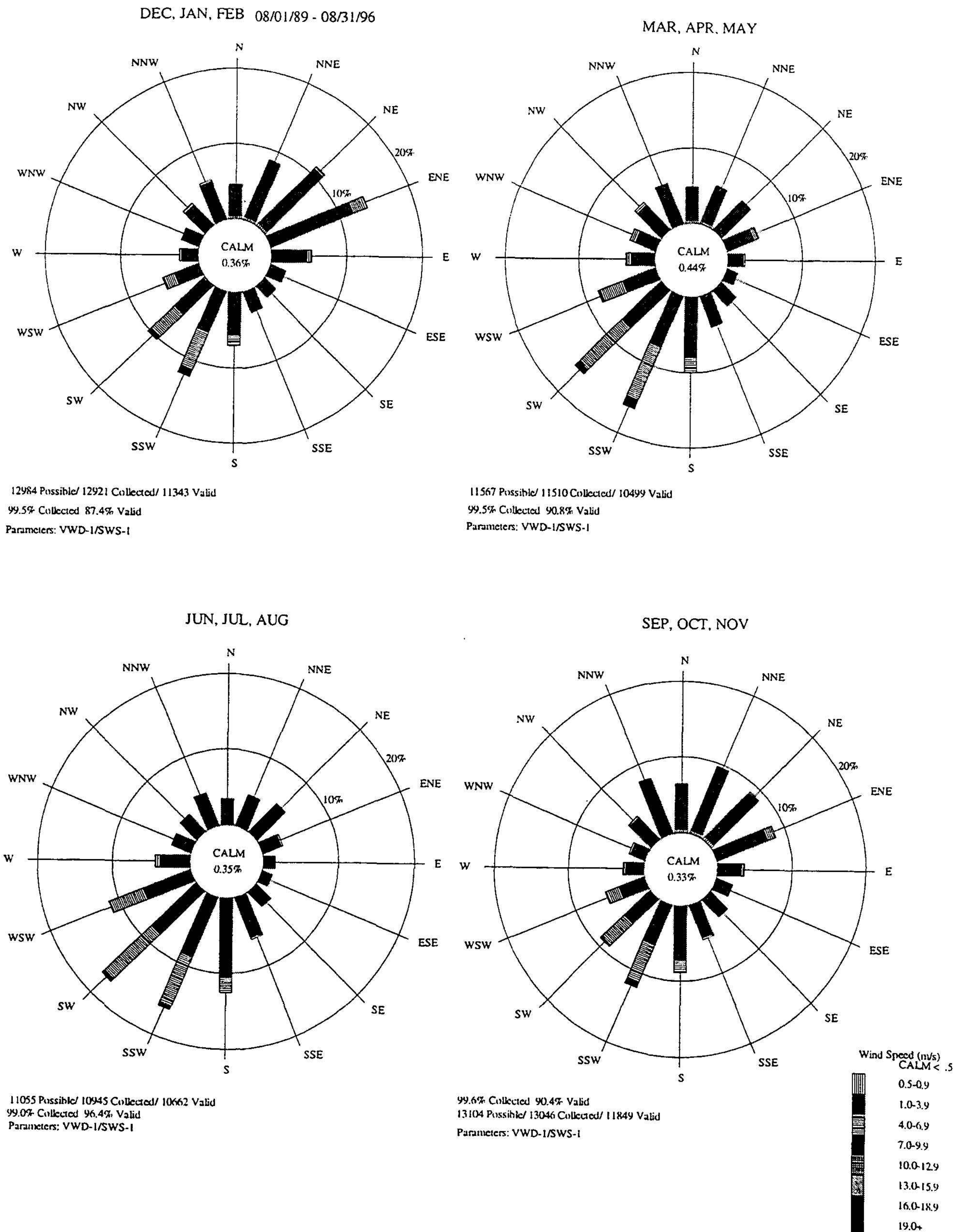
Figure 9-3. Seasonal wind roses for Grand Canyon National Park for 1989-1996.
