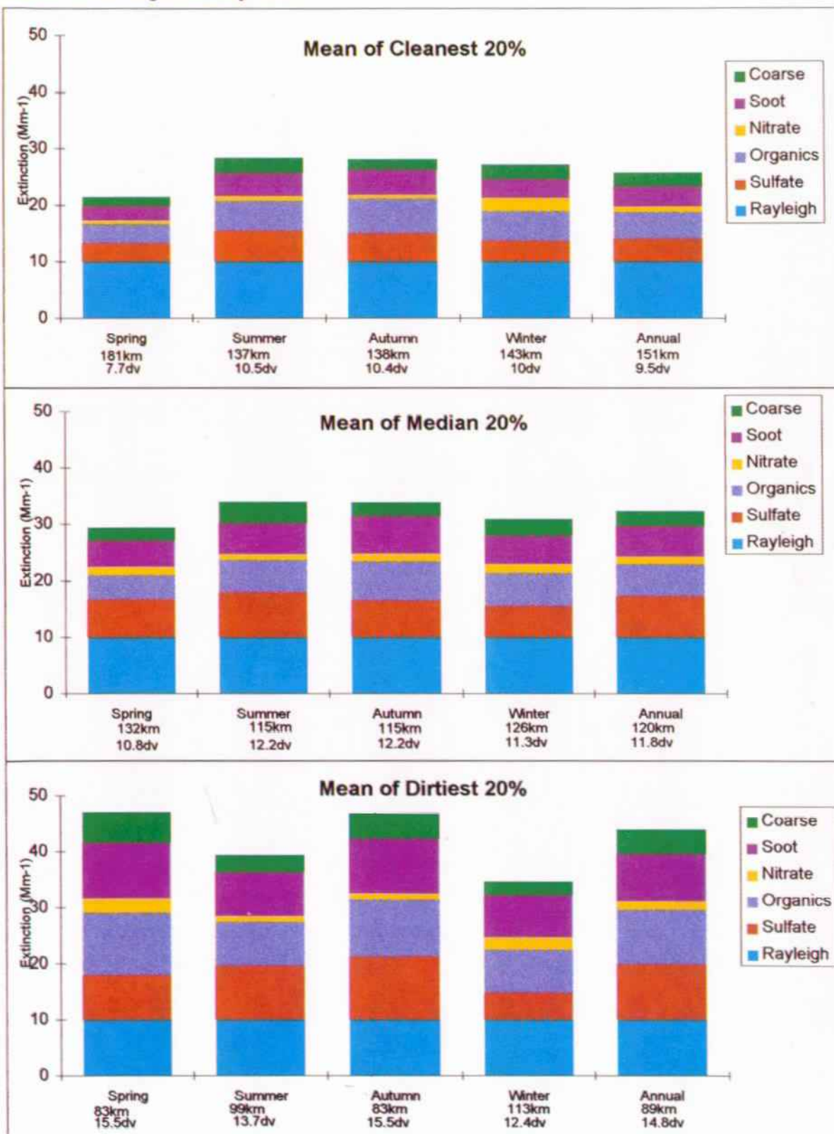
Figure 4-3. Reconstructed extinction budgets for Bandelier NM, March 1993 through February 1994.
