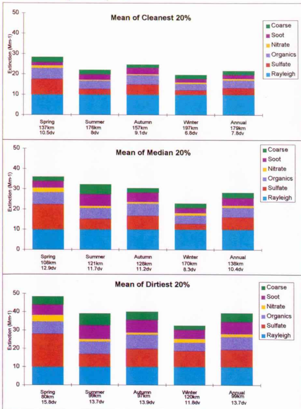
Figure 10-4. Reconstructed extinction budgets for Great Sand Dunes NM, March 1993 through February 1994.
