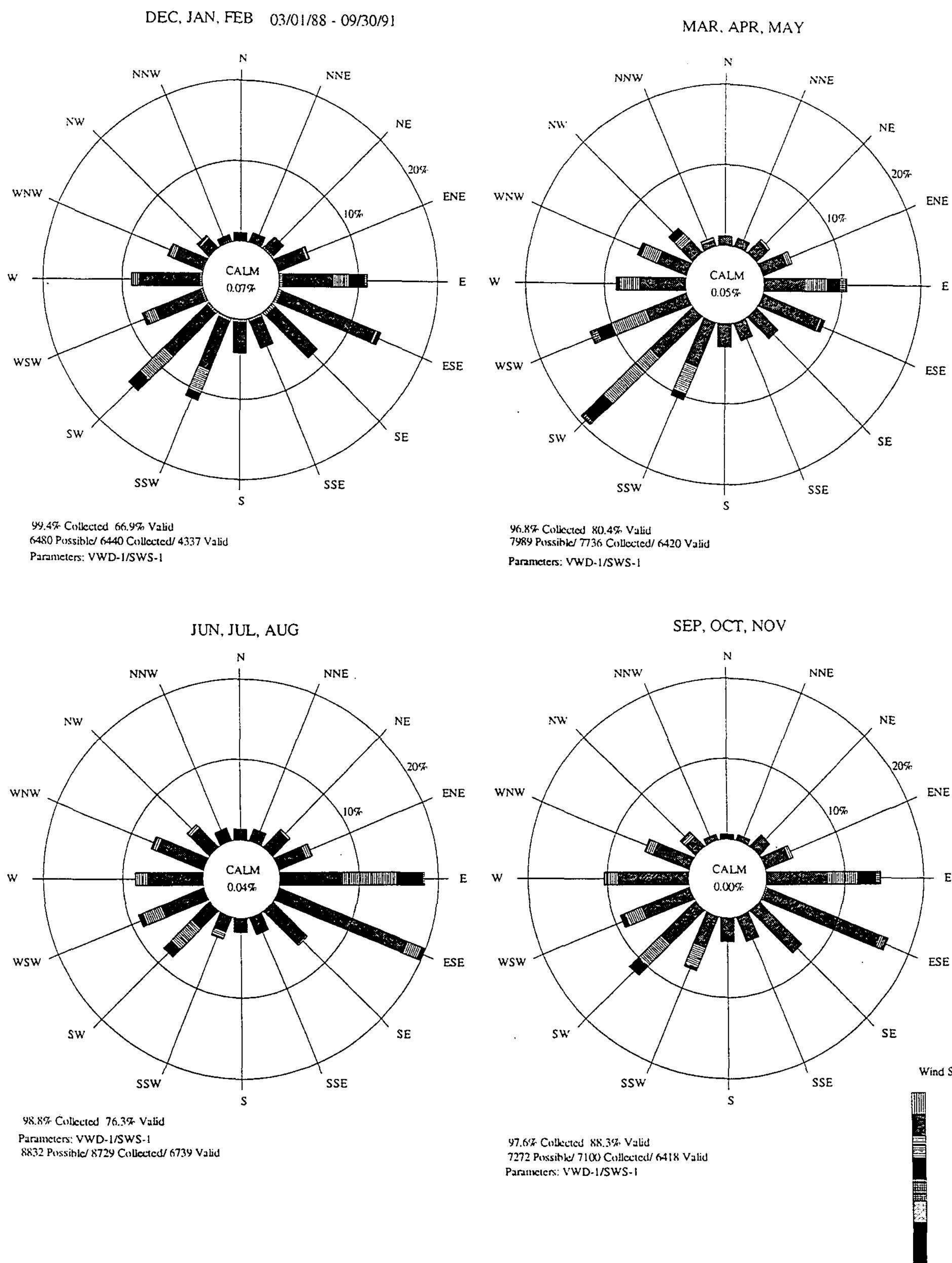
Figure 10-3. Seasonal wind roses for Great Sand Dunes National Monument, 1988-1991.
