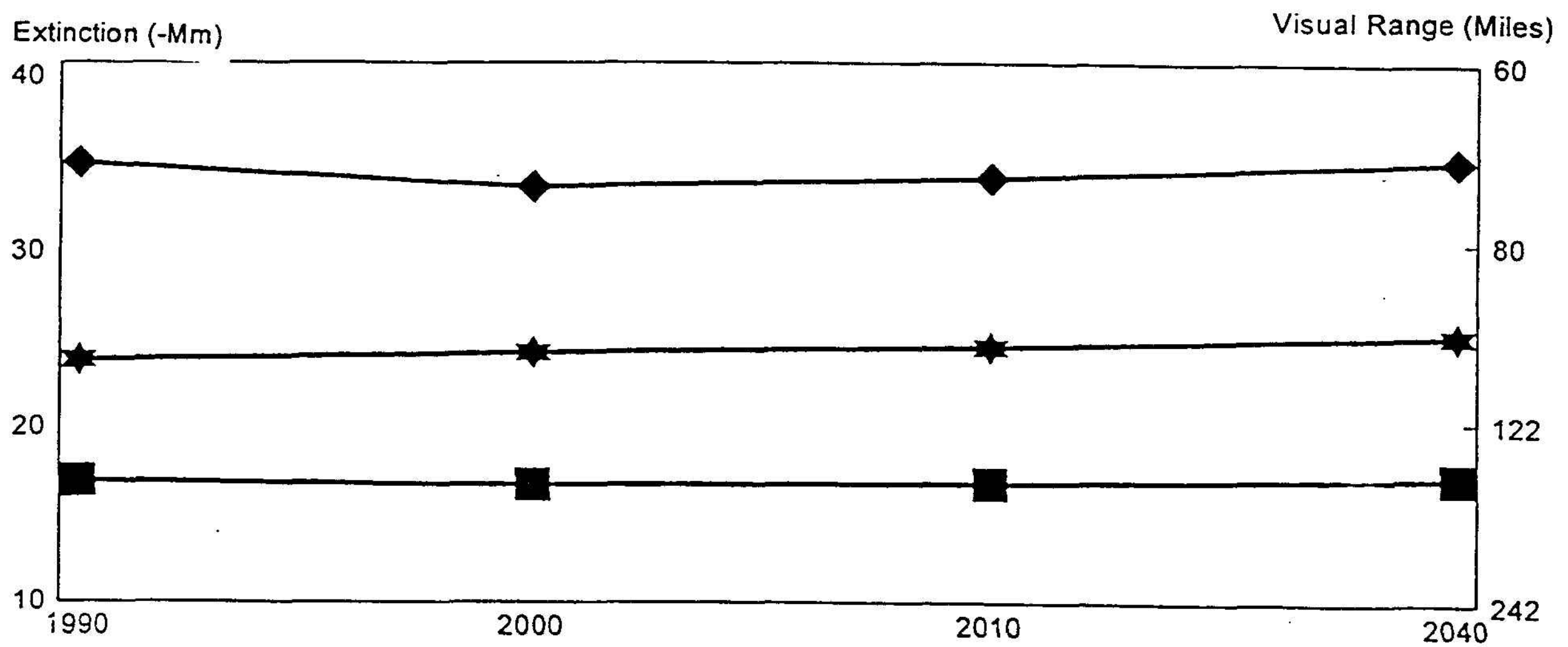
Figure 9-8. Projected "baseline" visibility for the Grand Canyon (Hopi Point) for good, average, and poor visibility conditions (from GCVTC 1996).
