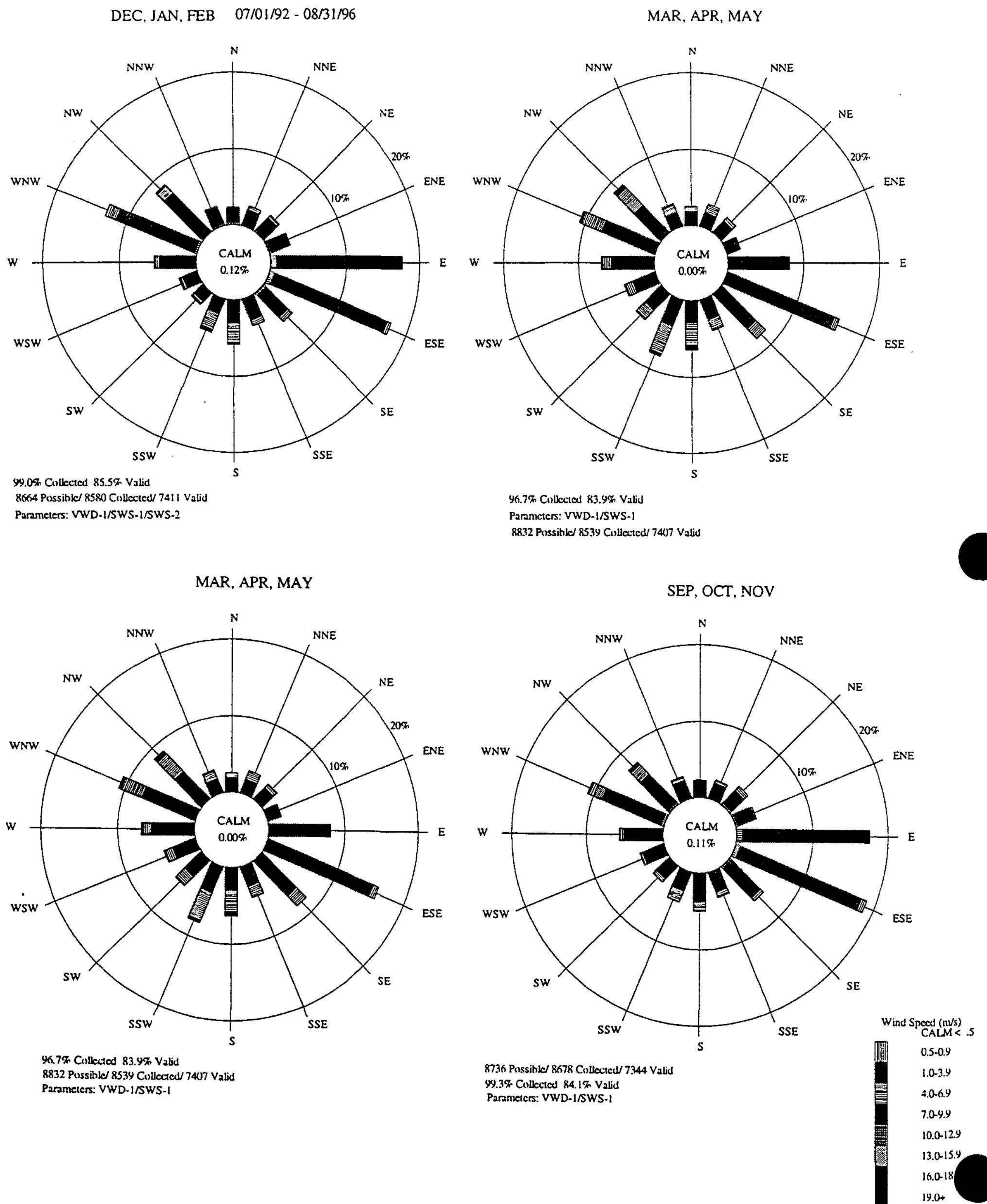
Figure 7-3. Wind rose for Canyonlands National Park, 1992-1996.
