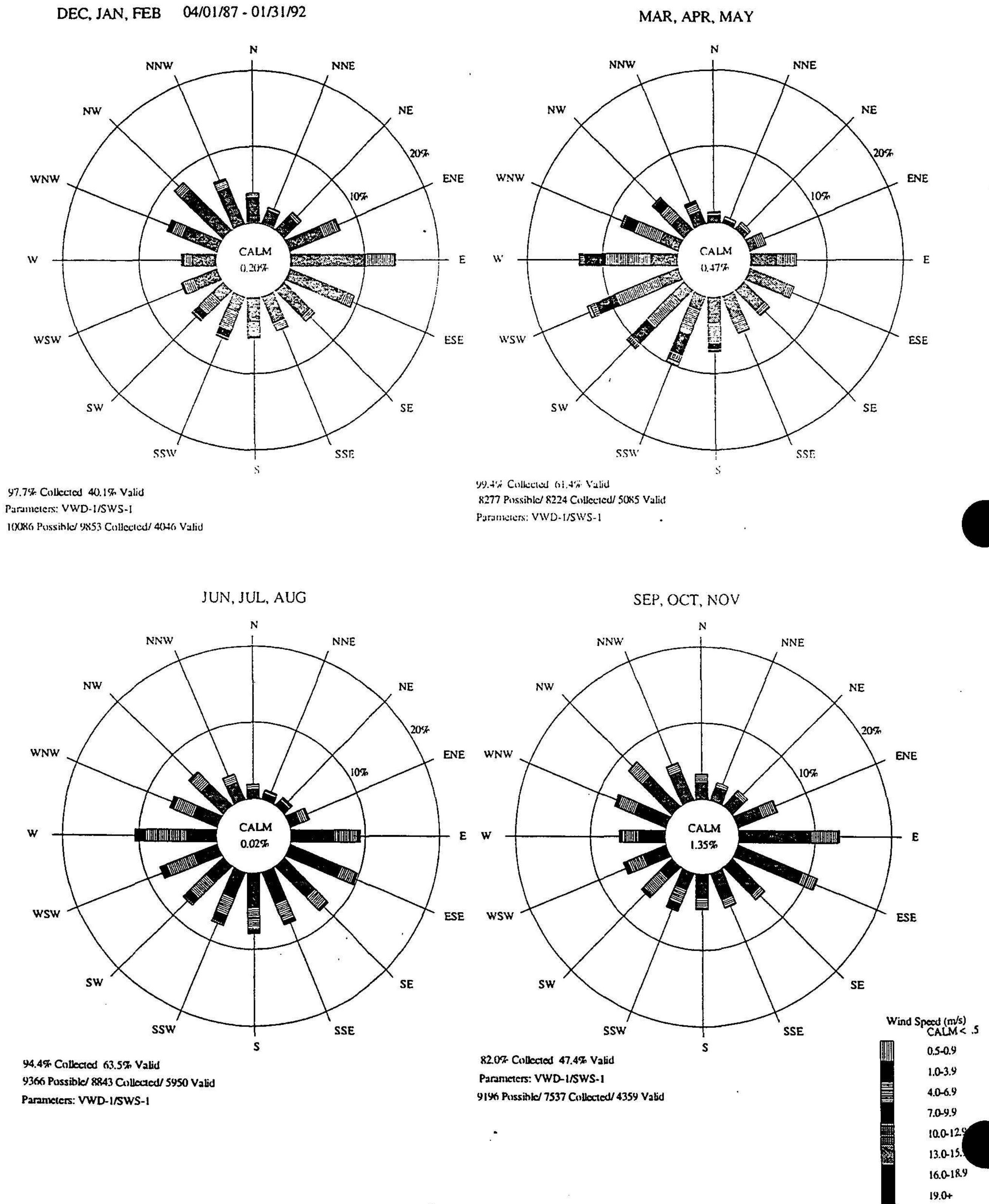
Figure 12-3. Seasonal wind roses for Petrified Forest National Park (1987-1992).
