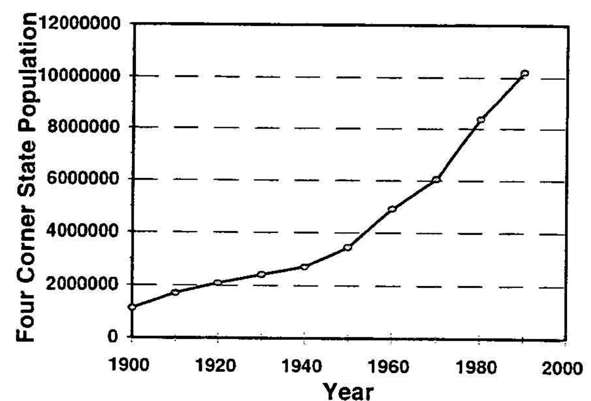
Figure 14-2. Census Bureau population for the 4-corner states (data from Hecox 1995).
