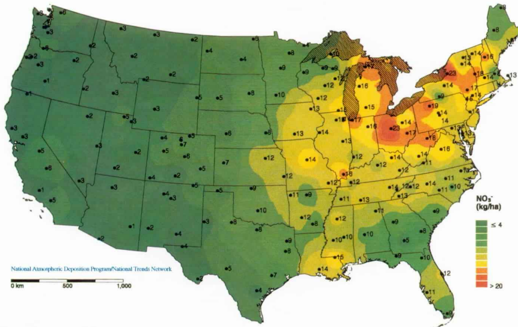
Figure 1-10. Nitrate deposition ( \text{NO}_3^- ; multiply by 0.226 for N only) for the U.S. for 1995 (map from NADP, Colorado State University).
