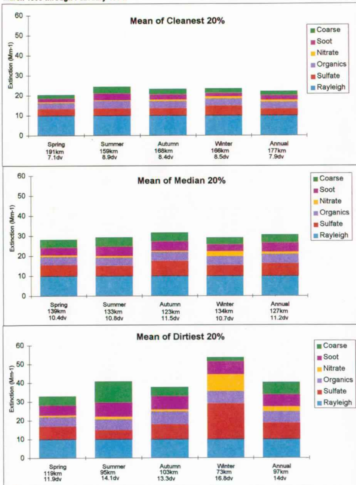
Figure 7-4. Reconstructed extinction budgets for Canyonlands NP, March 1993 through February 1994.
