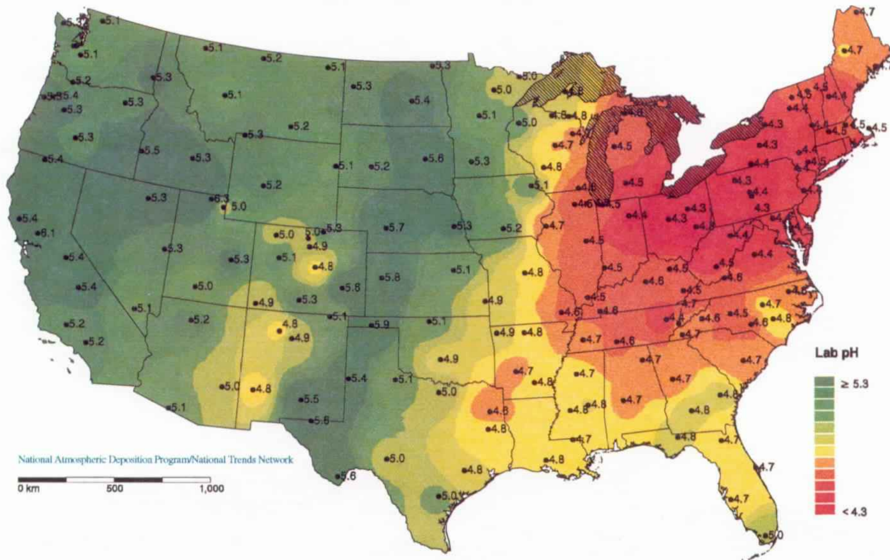
Figure 1-6. Rainfall pH (laboratory values) for the U.S. for 1995 (map from NADP, Colorado State University).
