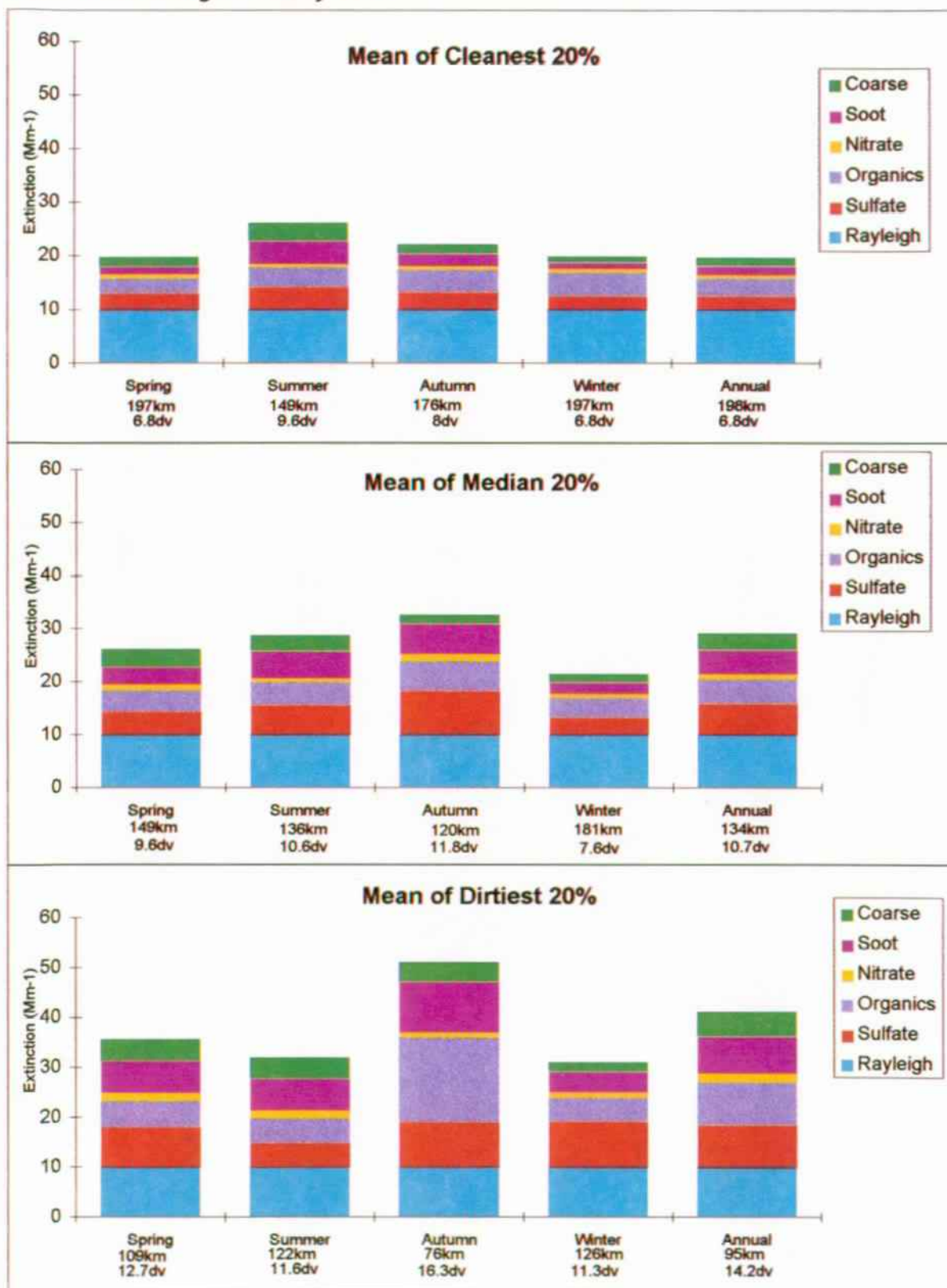
Figure 9-4. Reconstructed extinction budgets for the South Rim, March 1993 through February 1994.
