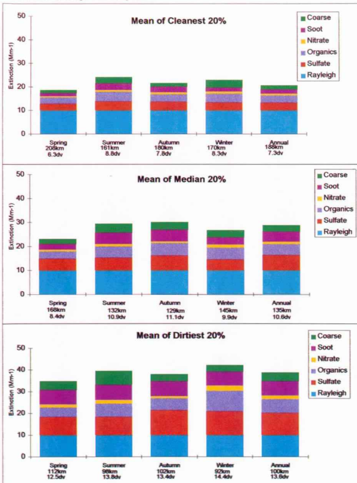
Figure 11-4. Reconstructed extinction budgets for Mesa Verde NP, March 1993 through February 1994.
