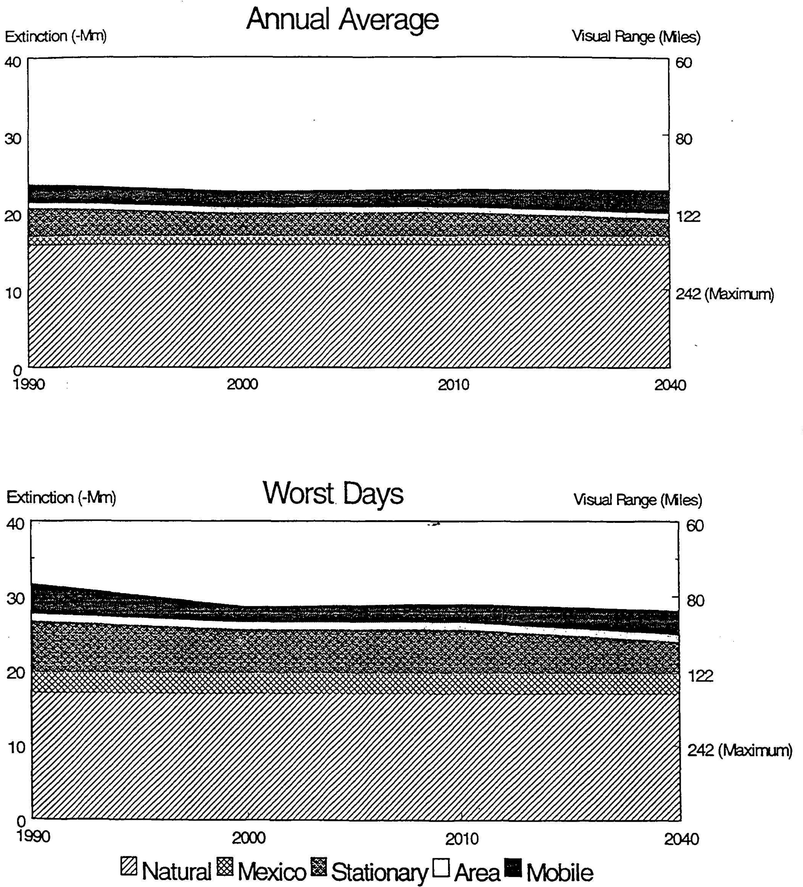
Figure 7-6. Projected "baseline" light extinction for Canyonlands National Park (GCVTC 1996).
