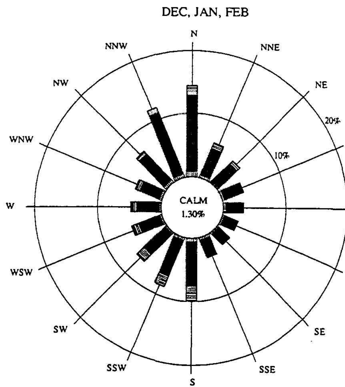
Figure 4-2. Seasonal wind roses for Bandelier National Monument (1990-1993).
