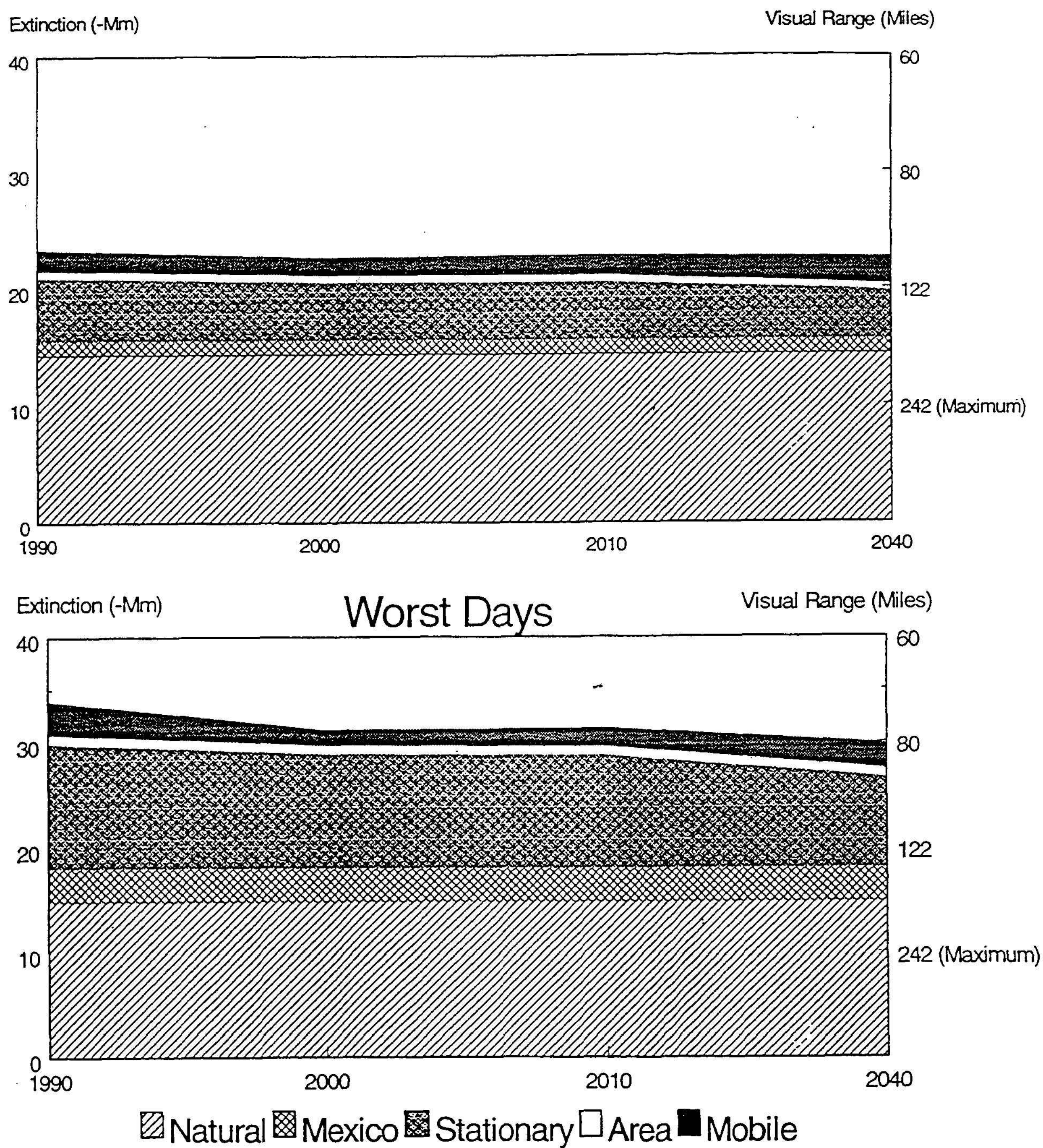
Figure 11-6. Projected "baseline" light extinction for Mesa Verde National Park (GCVTC 1996).
