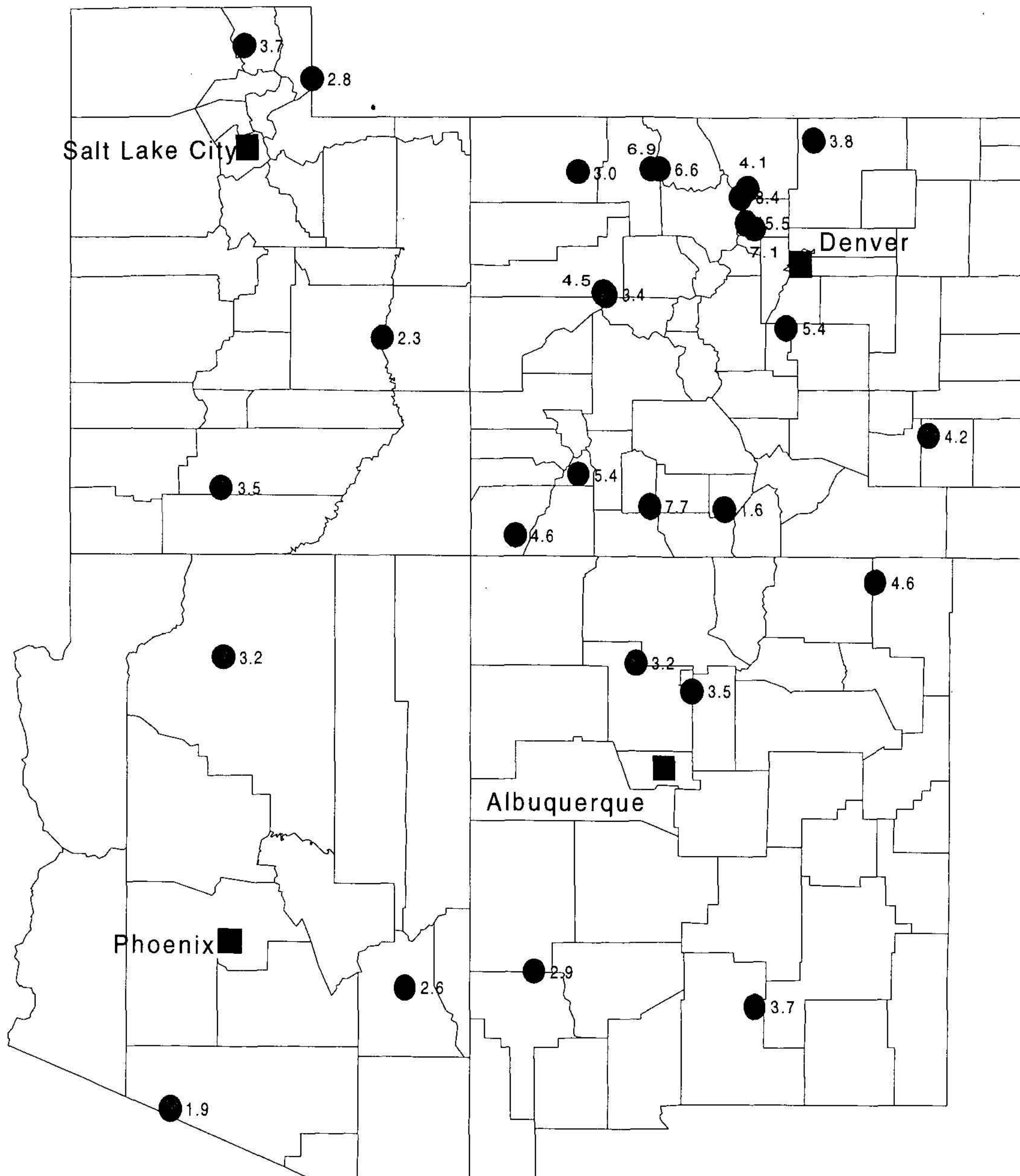
Figure 1-9. Nitrate deposition ( \text{NO}_3^- ; multiply by 0.226 for N only) for the Colorado Plateau and surrounding areas. Dots represent NADP monitoring sites, squares are major cities (data from NADP, Colorado State University).
