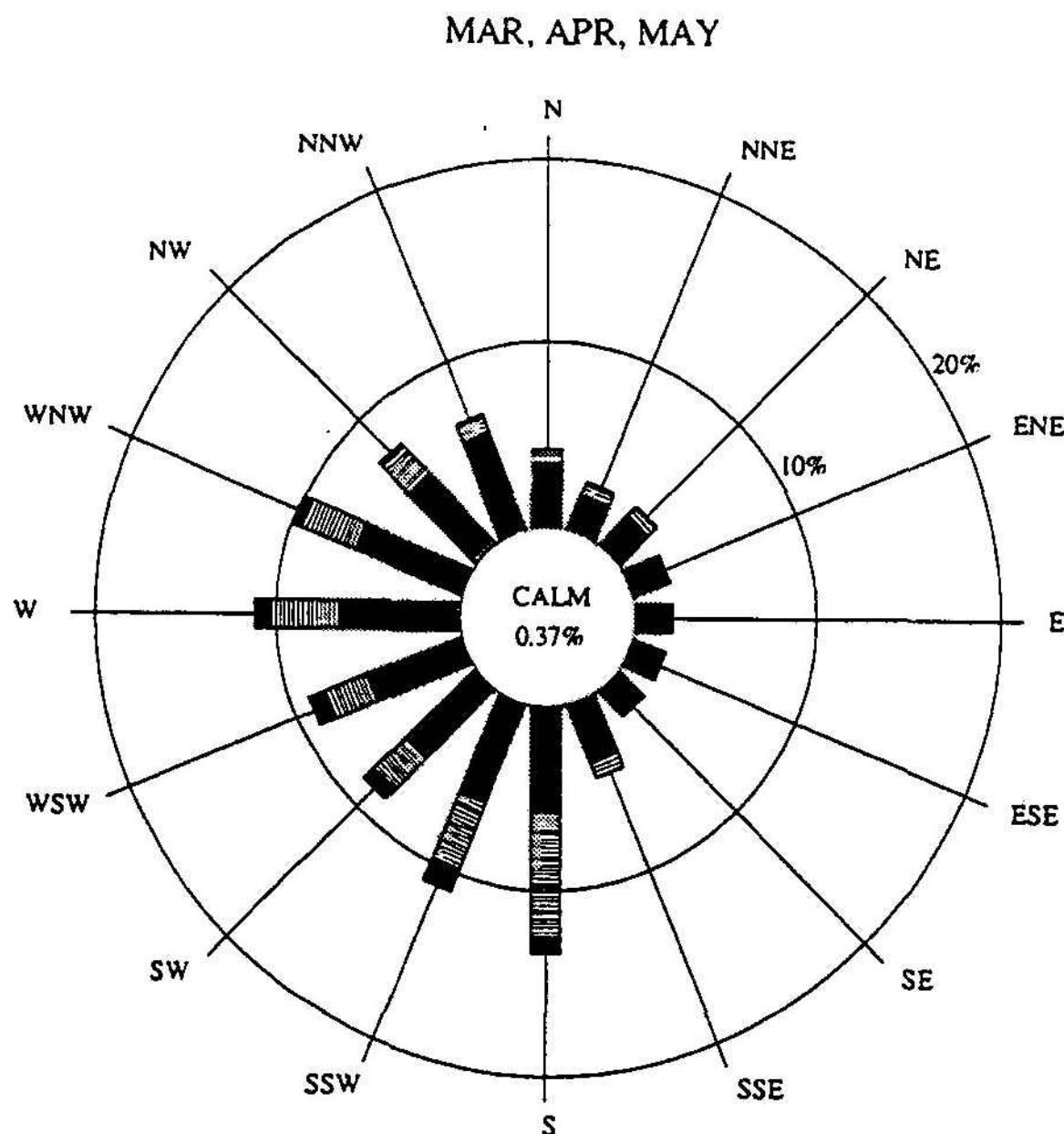
Figure 4-2. Seasonal wind roses for Bandelier National Monument (1990-1993).
