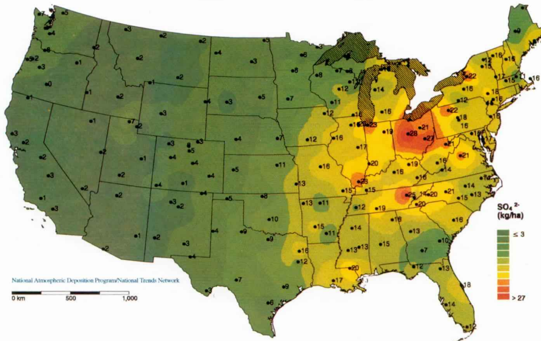
Figure 1-12. Sulfate deposition ( \text{SO}_4^{2-} ; multiply by 0.333 for S only) for the U.S. for 1995 (map from NADP, Colorado State University).
