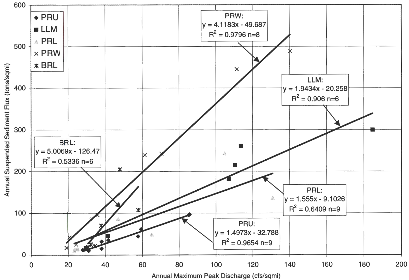
Figure 10. Prairie Creek Annual Suspended Sediment Flux vs Annual Maximum Peak Discharge
