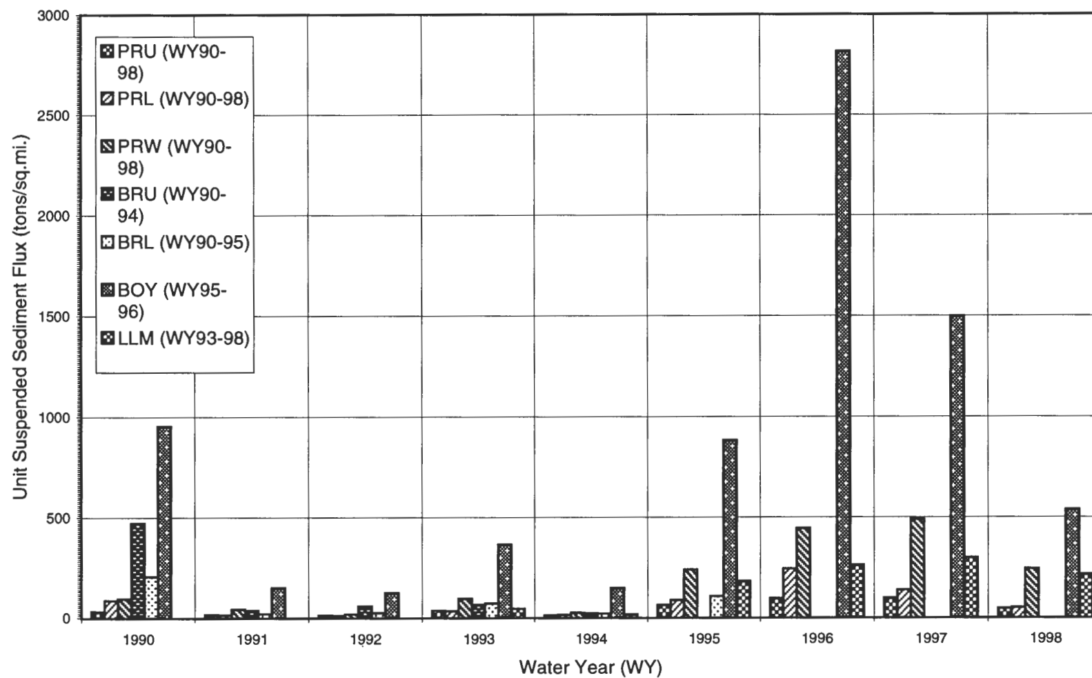
Figure 8. Unit Suspended Sediment Flux at Prairie Creek Basin Gages: WY90-98
