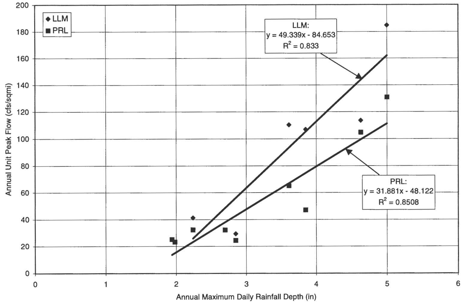
Figure 4. Annual Maximum Daily Rainfall vs Annual Peak Flow
