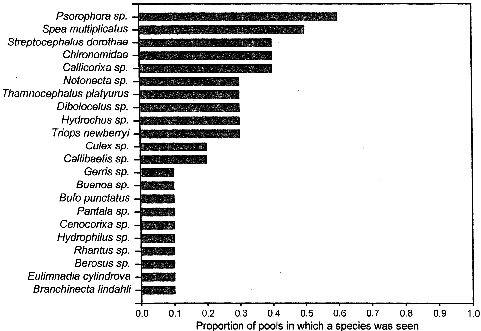
Figure 2b. Proportion of the 10 ephemeral pools surveyed in which each species was observed.
