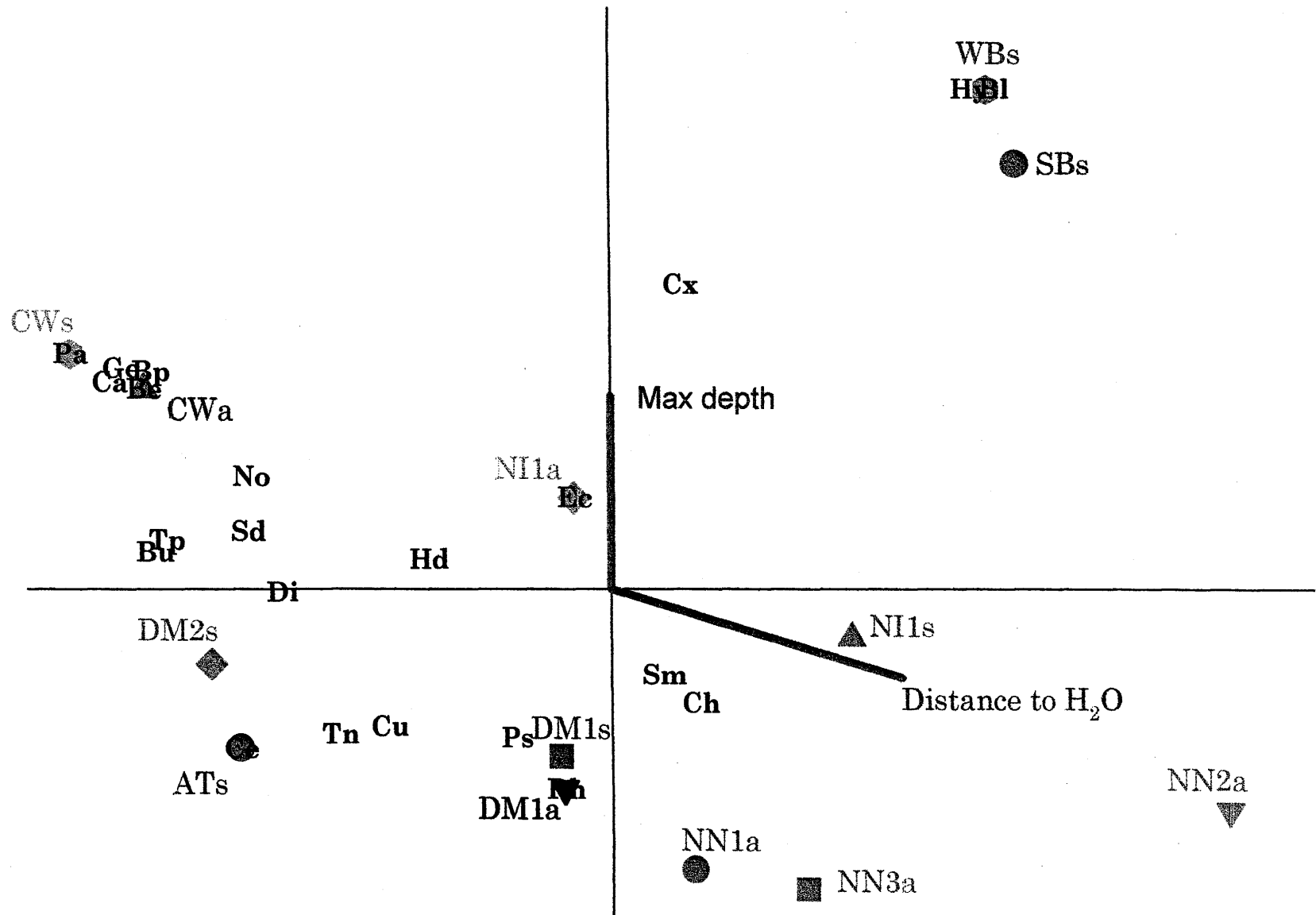
Figure 3. NMS of species (letters) and pools (symbols) from surveys at Wupatki NM. Species abbreviations are listed in Table 2.
