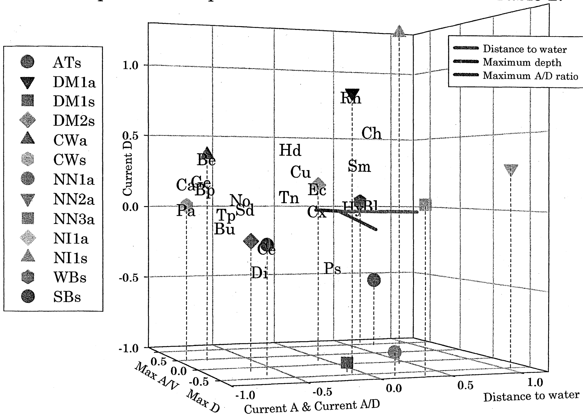
Figure 4. NMS of species (letters) and pools (symbols) from survey at Wupatki NM. Species abbreviations are listed in Table 2.
