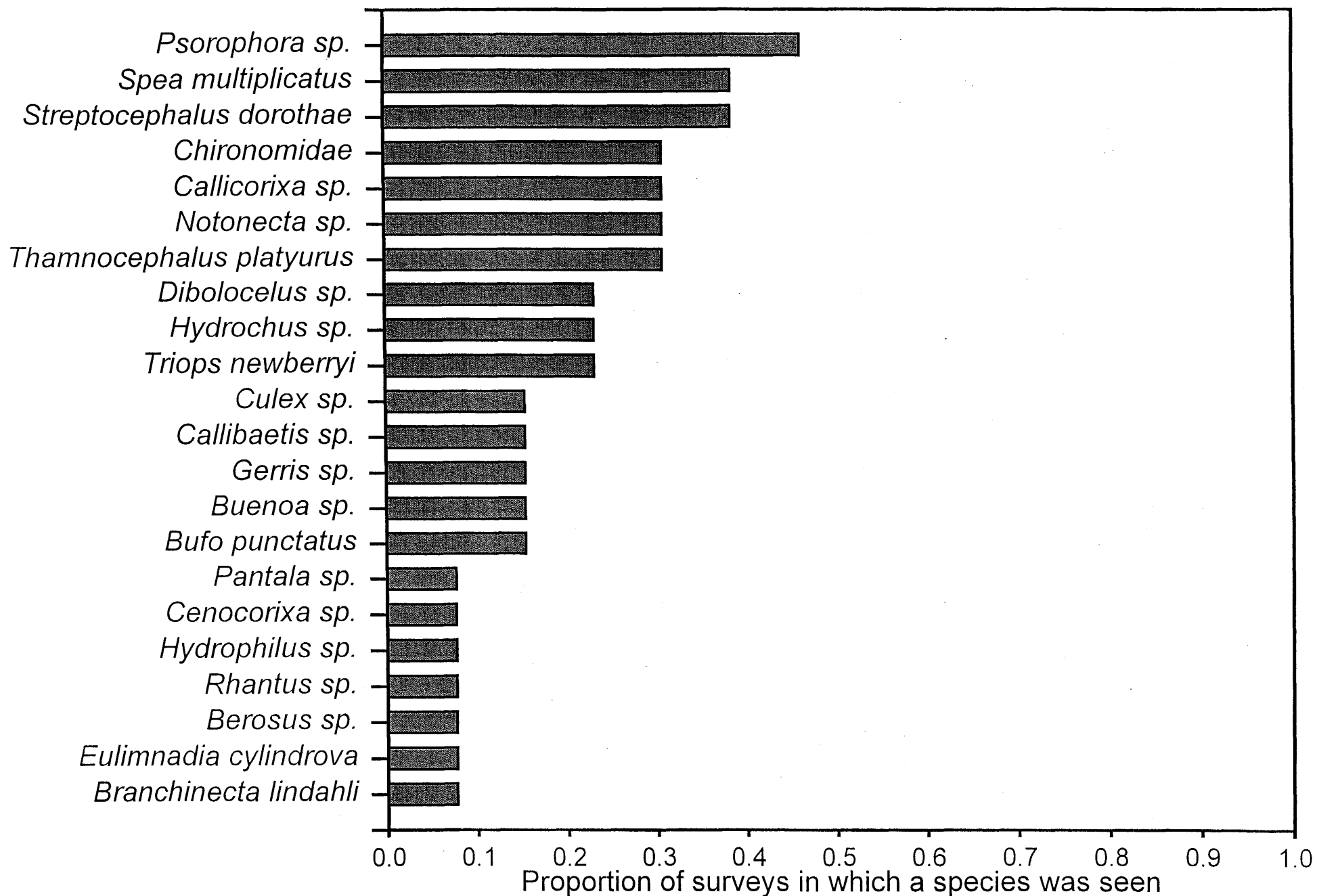
Figure 2a. Proportion of pool surveys in which each species was observed for all 13 surveys: six pools surveyed in August, seven surveyed in September; three pools surveyed on both dates.
