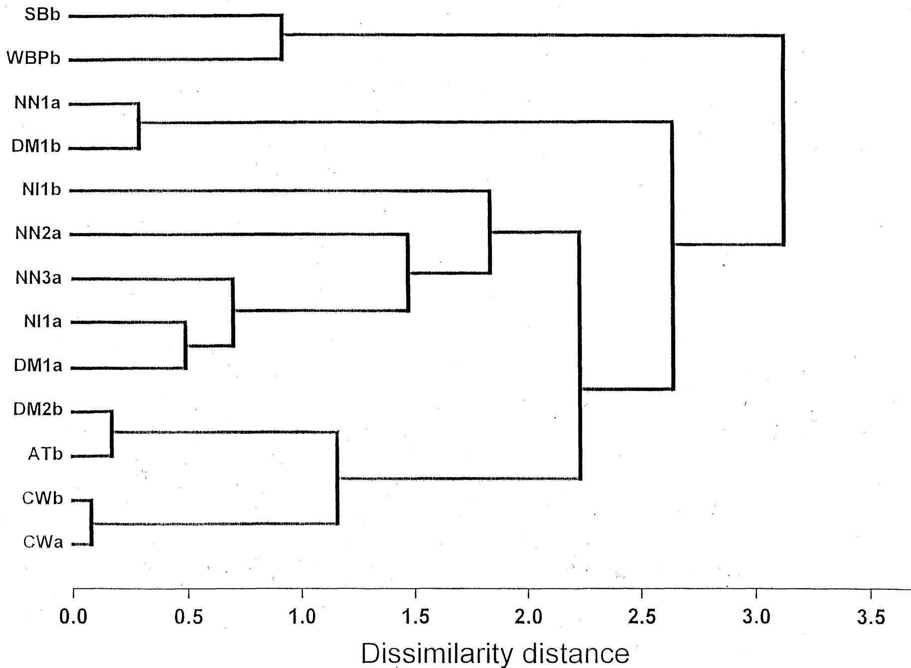
Cluster diagram of Wupatki NM pool communities using Relative Sorensen's dissimilarity index.
