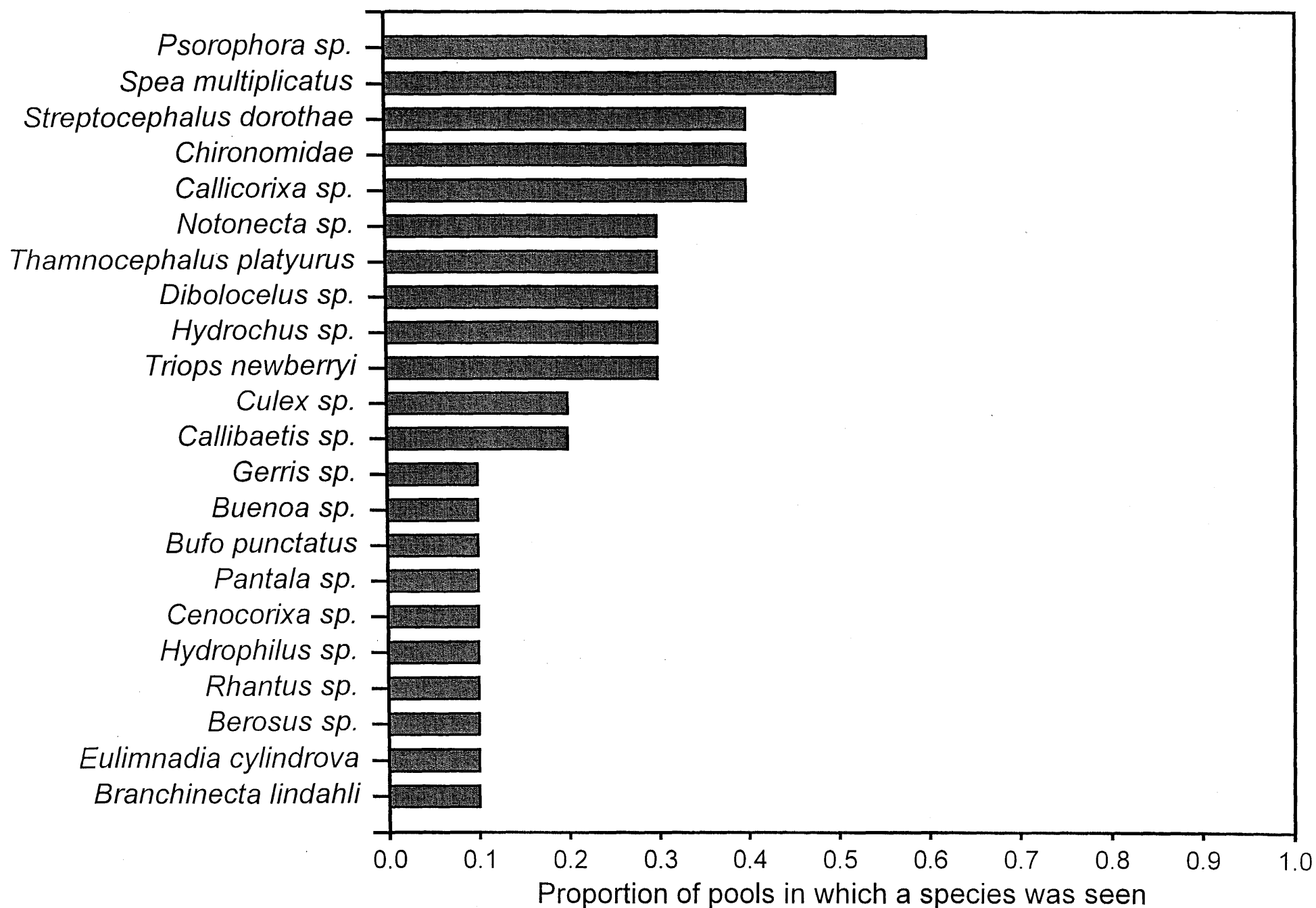
Figure 2b. Proportion of the 10 ephemeral pools surveyed in which each species was observed.
