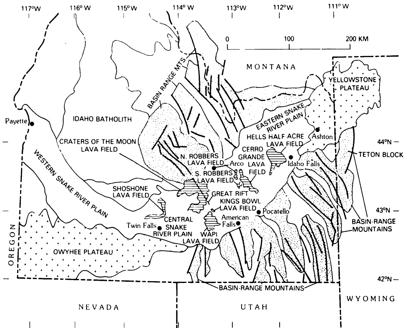
Figure 1. Index map showing generalized geology of southern Idaho and localities referred to in the text.
