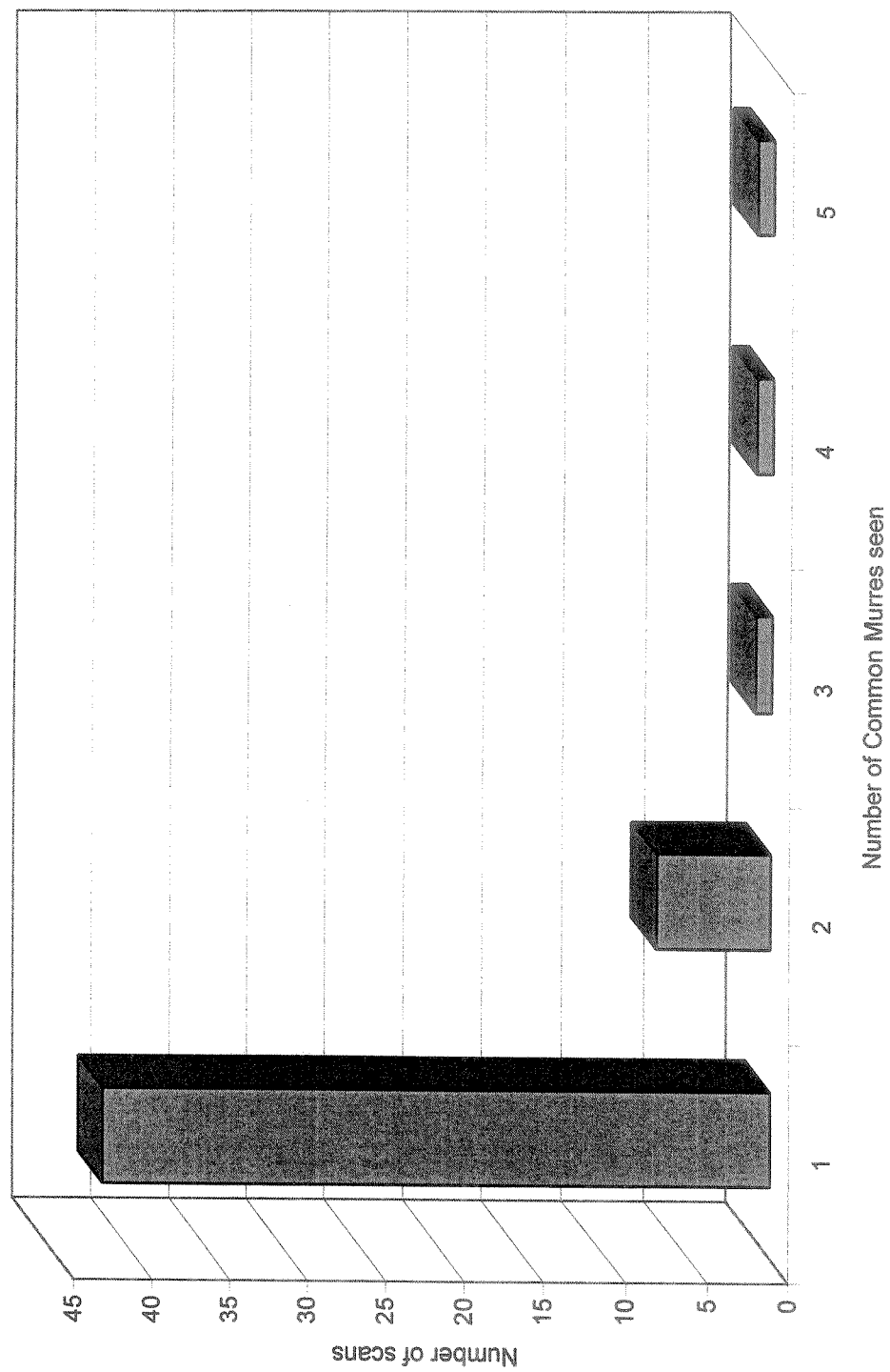
Figure 10. Number of scans resulting in Common Murre observations on San Pedro Rock, 17 April to 7 August 2003.
