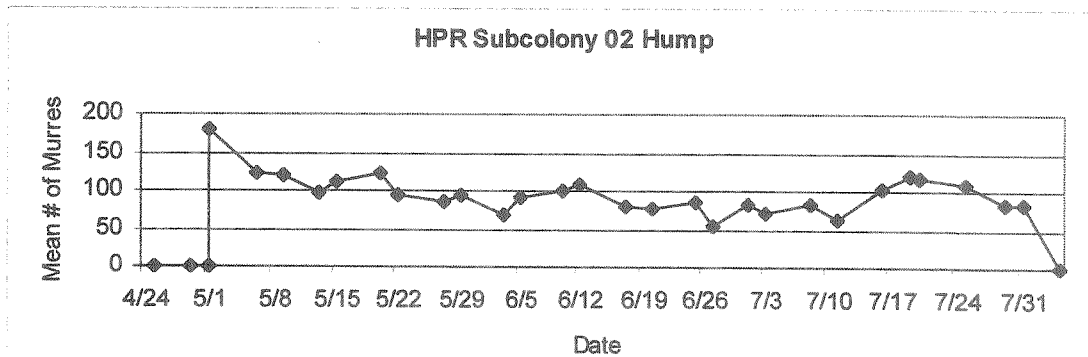
Figure 16. Seasonal attendance patterns of Common Murres at Hurricane Point Rocks subcolony 01, 02 Ledge, and 02 Hump, 17 April to 04 August 2003.
