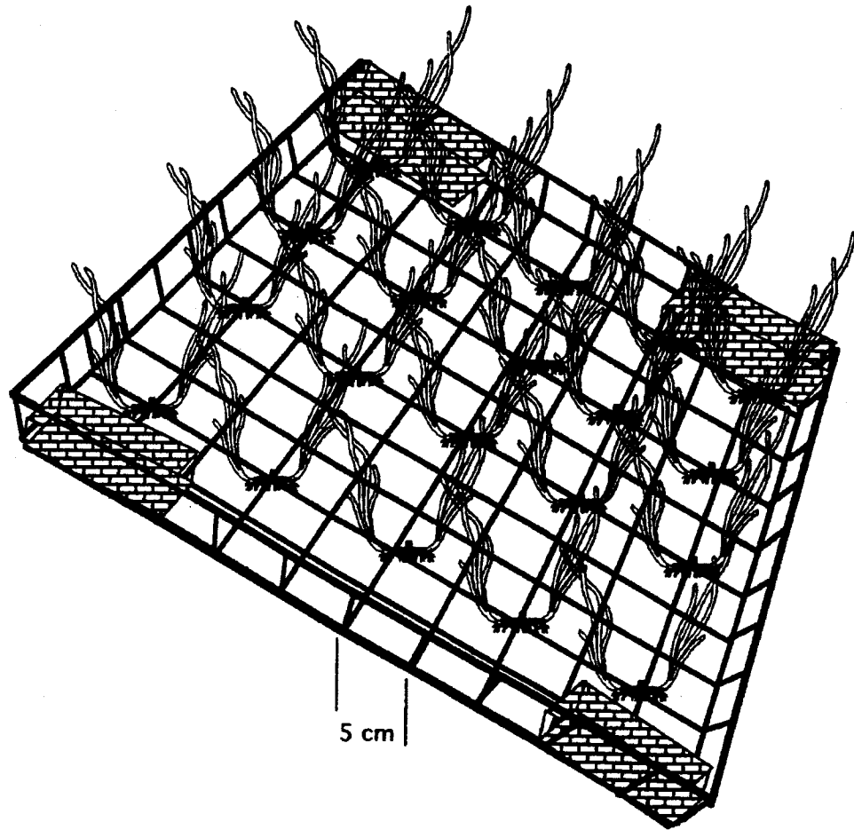
Figure 3.7. Remote planting method (TERFS: Transplanting Eelgrass Remotely with Frame Systems, developed by F. Short, Univ. New Hampshire), designed to avoid the cost of divers and for deployment in contaminated areas (e.g., PCBs) that might otherwise not affect plant growth but cause diving operations to be costly and hazardous. This method may also be applied as a bioassay tool. Plants are attached to the frame with paper ties, the frame can be retrieved after a suitable rooting time, leaving the plants in the sediment.
