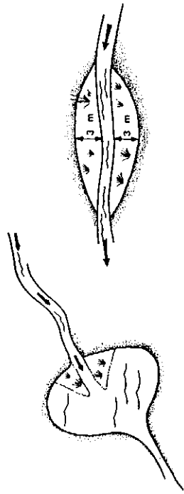
Figure 12: Rapid Predictor of Sediment Removal Relationship (from Larson, Adamus and Clairain, 1989, pp. 30-31).
