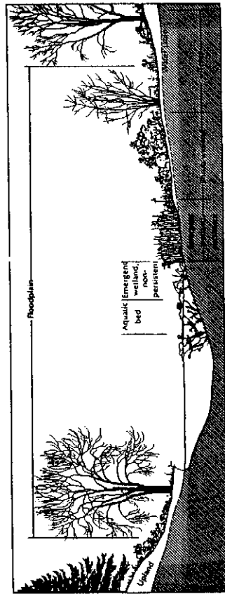
Figure 13: Riparian System Cross-Section (from Bickford and Dymon, 1990, p. 16).
