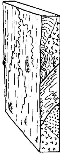
Figure 51: Continued Evolution of the Southern New England Landscape. The same area is shown after a long period of erosion, as the streams have gradually reduced the land to a peneplain (from Jorgensen, 1977, p. 22).
