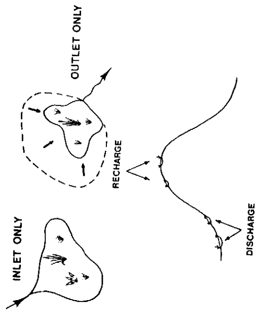
Figure 11: Rapid Predictors of Ground Water Relationships (from Larson, Adamus and Clairain, 1989, pp. 15-17).
