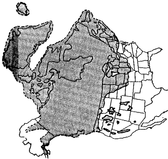
Figure 53: Map of North America Showing the Extent of the Pleistocene Ice Age Approximately 2,000 Years Ago (from Jorgensen, 1977, p. 83).
