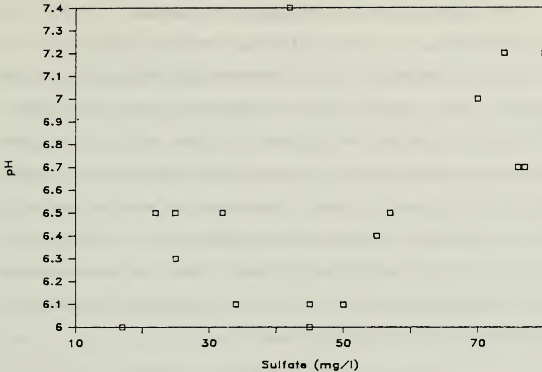
Figure 29. Plot of pH vs. sulfate for Site R0-1 in Rock Creek ( r = 0.56 , n = 17 ).
