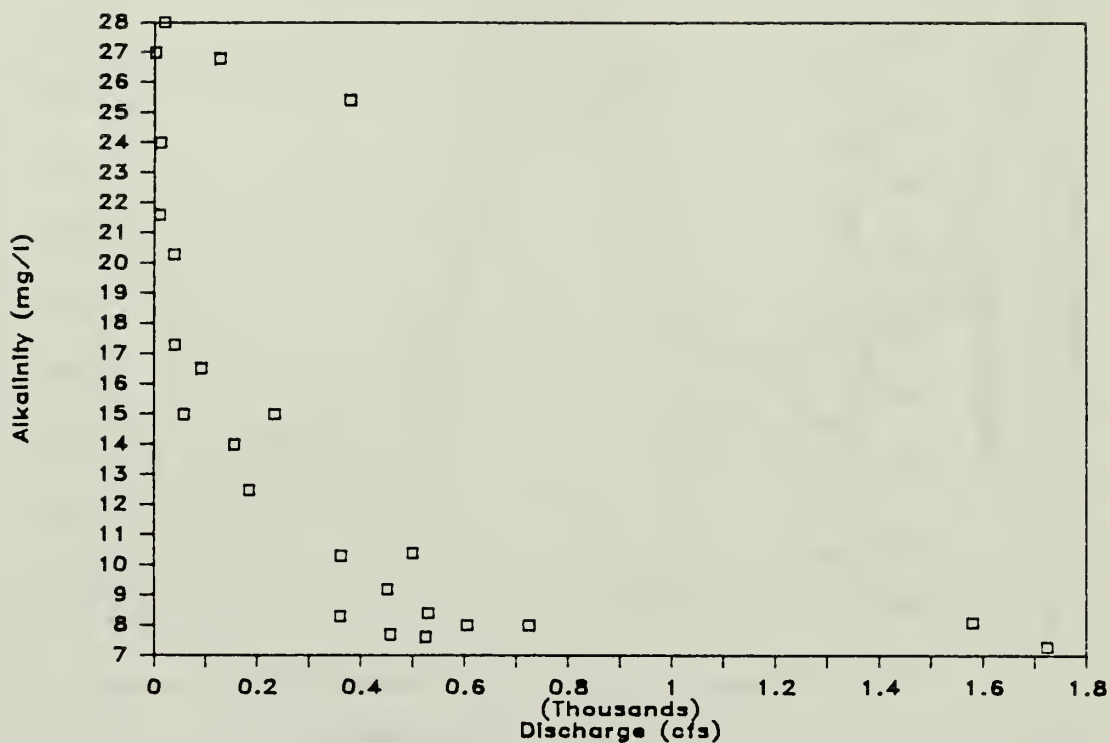
Figure 23. Plot of alkalinity vs. stream discharge for site CL-2 in Clear Fork.
