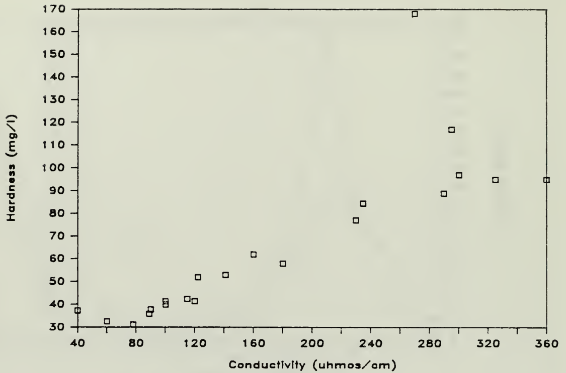
Figure 25. Plot of hardness vs. conductivity for site PI-3 in Pine Creek ( r = 0.84 , n = 21 ).
