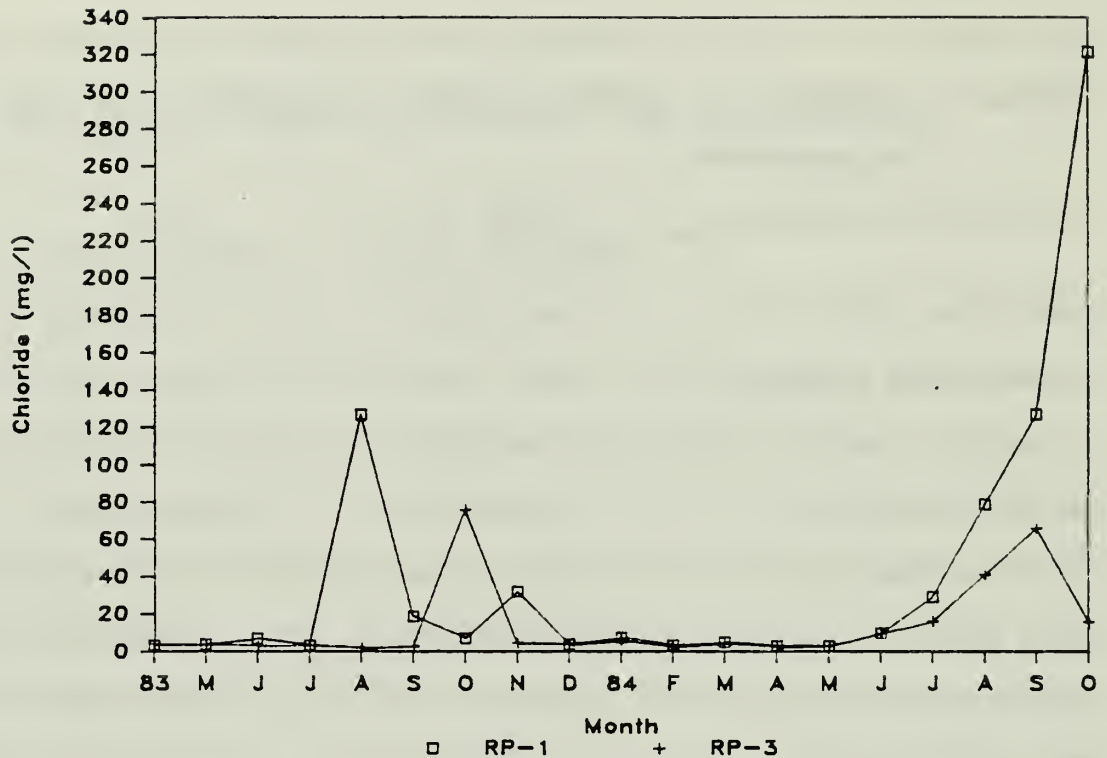
Figure 16. Seasonal fluctuations in chloride levels for sites RP-1 and RP-3 in Roaring Paunch Creek, a severely polluted stream.
