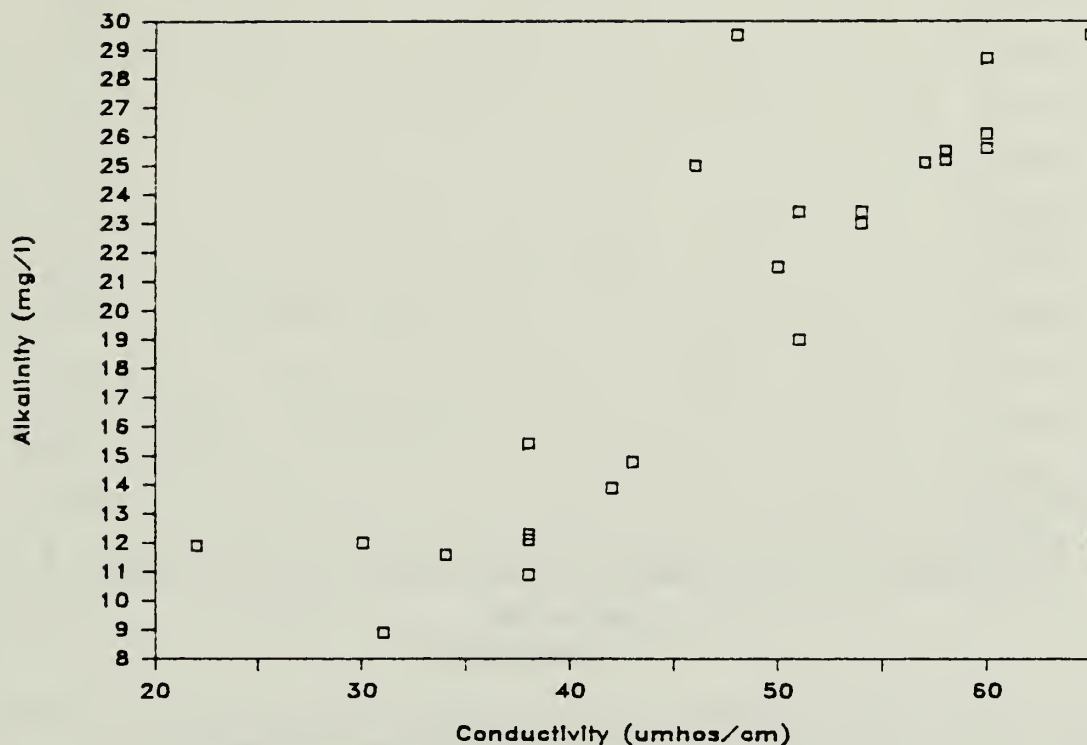
Figure 27. Plot of alkalinity vs. conductivity for site SC-3 in Station Camp Creek ( r = 0.88 , n = 24 ).
