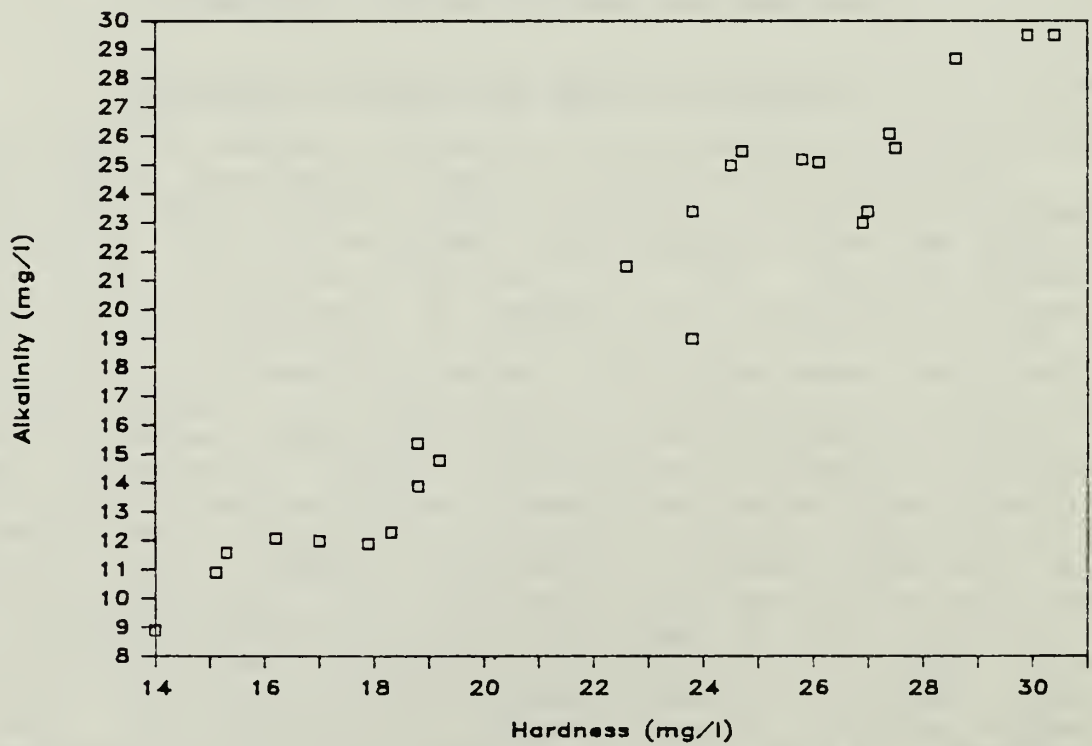
Figure 26. Plot of alkalinity vs. hardness for site SC-3 in Station Camp Creek ( r = 0.97 , n = 24 ).
