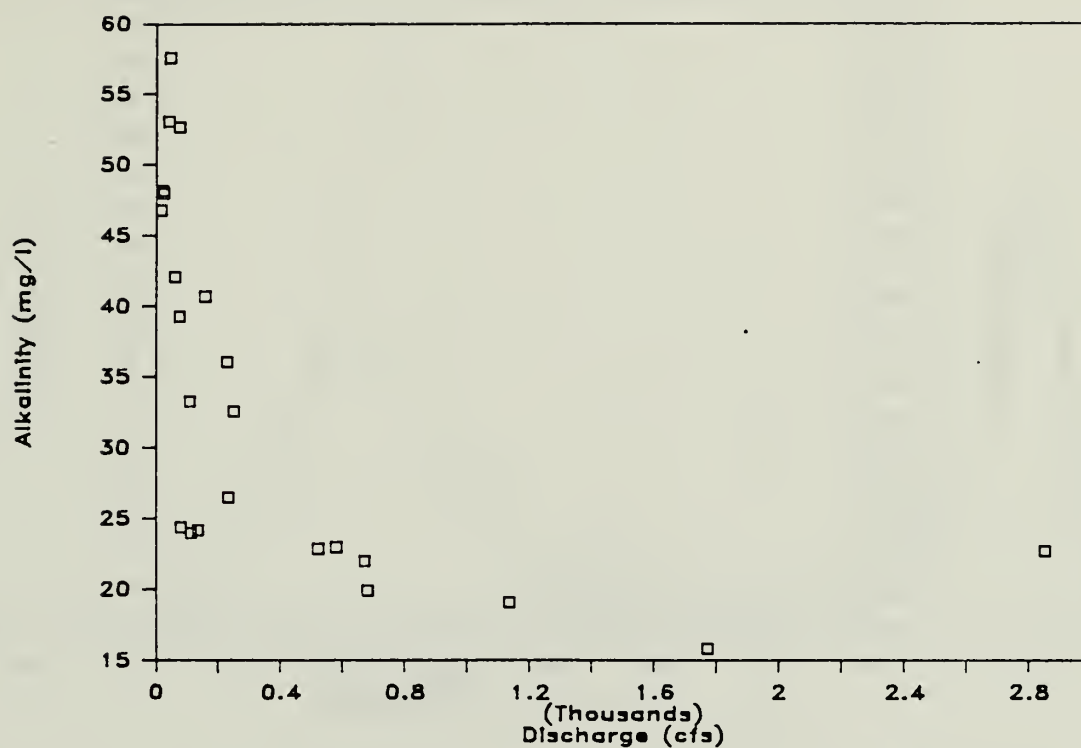
Figure 21. Plot of alkalinity vs. stream discharge for site NR-3 in New River.
