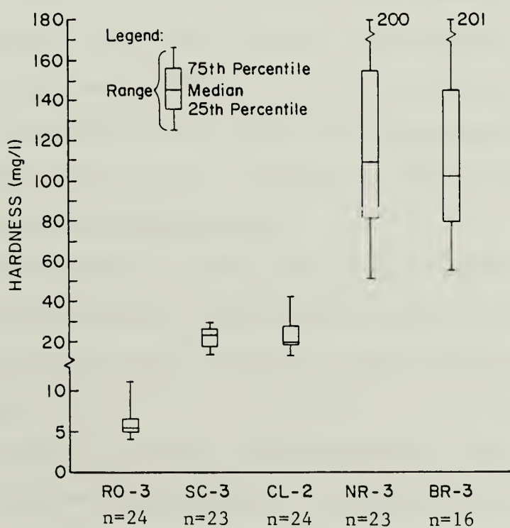
Figure 14. Medians and ranges of hardness values for the five example stream sites.
