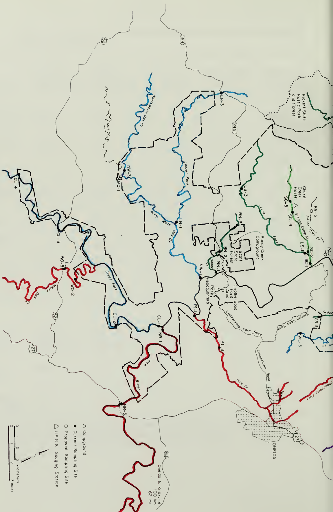
Figure 10. Stream category designations for tributaries monitored in the Big South Fork National River and Recreation Area.
