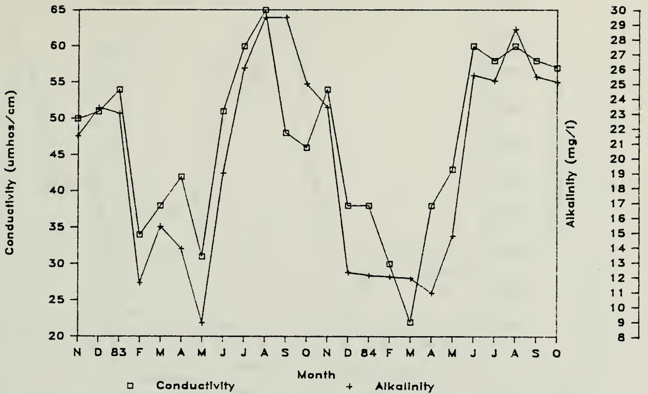
Figure 17. Seasonal fluctuations in conductivity and alkalinity levels for site SC-3 in Station Camp Creek, a clean/limestone-influenced stream.
