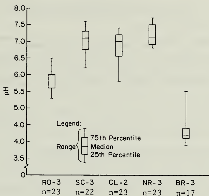
Figure 13. Medians and ranges of pH values for the five example stream sites.
