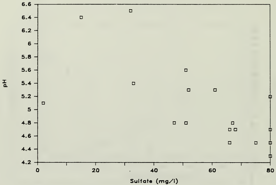
Figure 28. Plot of pH vs. sulfate for site BR-1 in Bear Creek ( r = 0.69 , n = 18 ).
