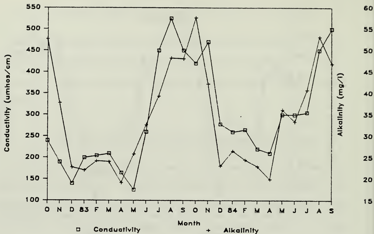
Figure 19. Seasonal fluctuations in conductivity and alkalinity levels for site NR-3 in New River, a moderately polluted stream.
