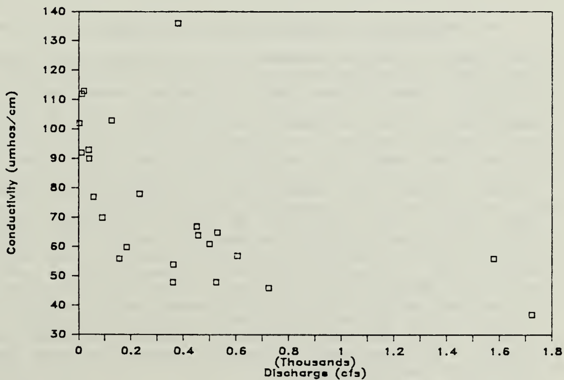
Figure 22. Plot of conductivity vs. stream discharge for site CL-2 in Clear Fork.
