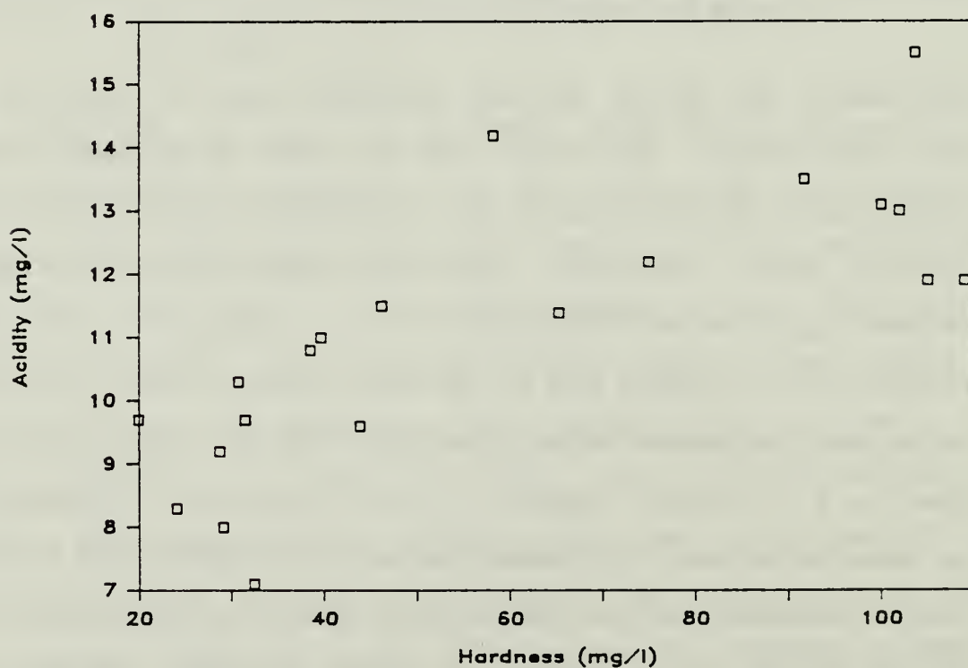
Figure 30. Plot of acidity vs. hardness for site RO-1 in Rock Creek ( r = 0.78 , n = 20 ).
