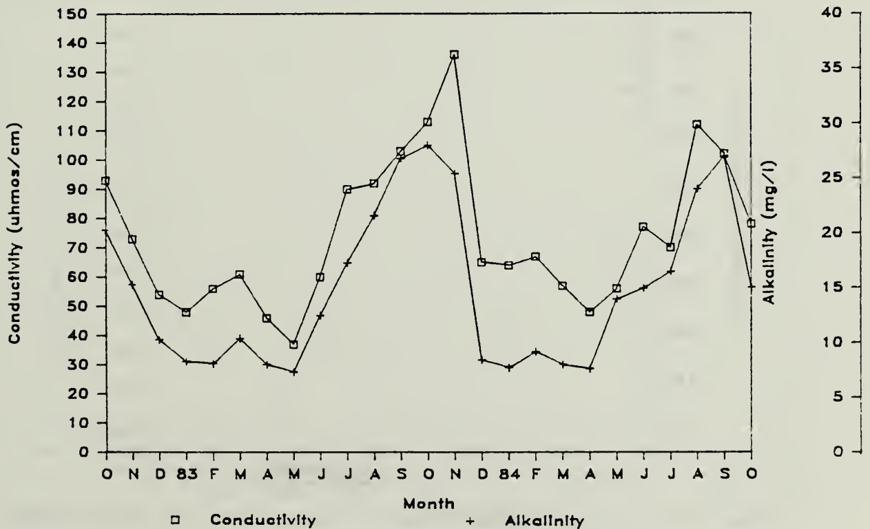
Figure 18. Seasonal fluctuations in conductivity and alkalinity levels for site CL-2 in Clear Fork, a slightly polluted stream.
