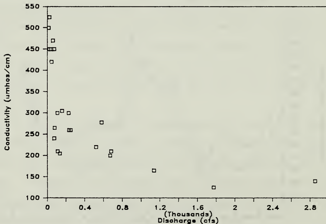
Figure 20. Plot of conductivity vs. stream discharge for site NR-3 in New River.
