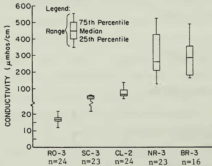
Figure 12. Medians and ranges of conductivity values for the five example stream sites.
