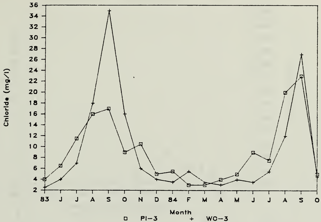
Figure 24. Seasonal fluctuations in chloride levels for site PI-3 in Pine Creek and site WO-3 in White Oak Creek.
