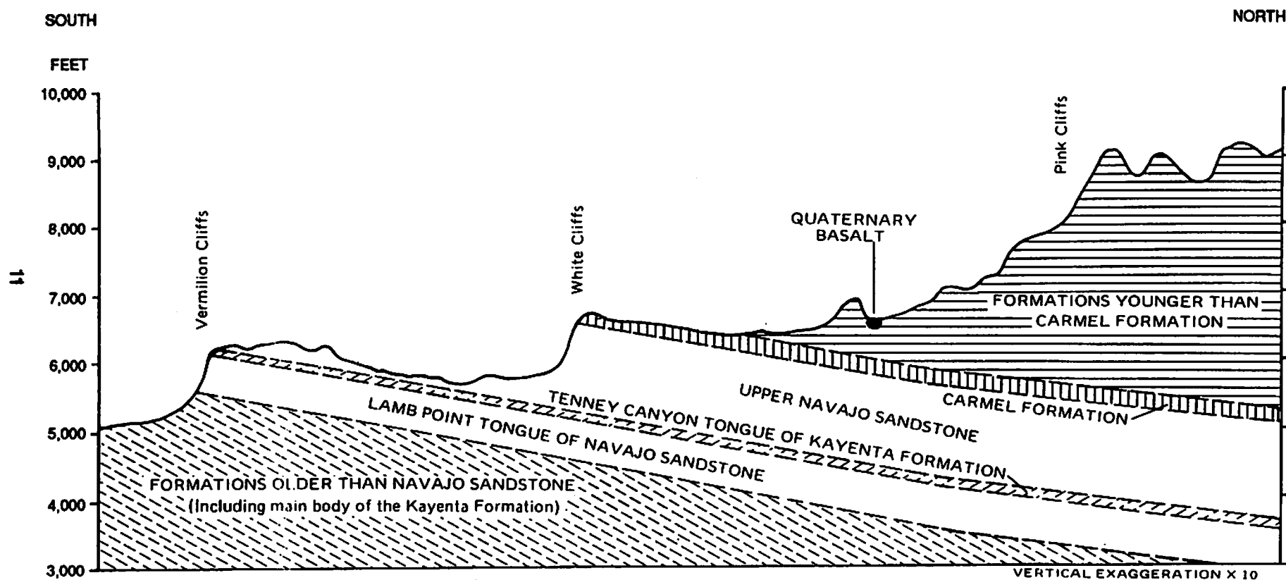
Figure 6.--Schematic section across the Kanab block indicating assumed thickness, attitude, and stratigraphic relation of younger and older formations with the two members of the Navajo Sandstone, in Kane County, Utah.
