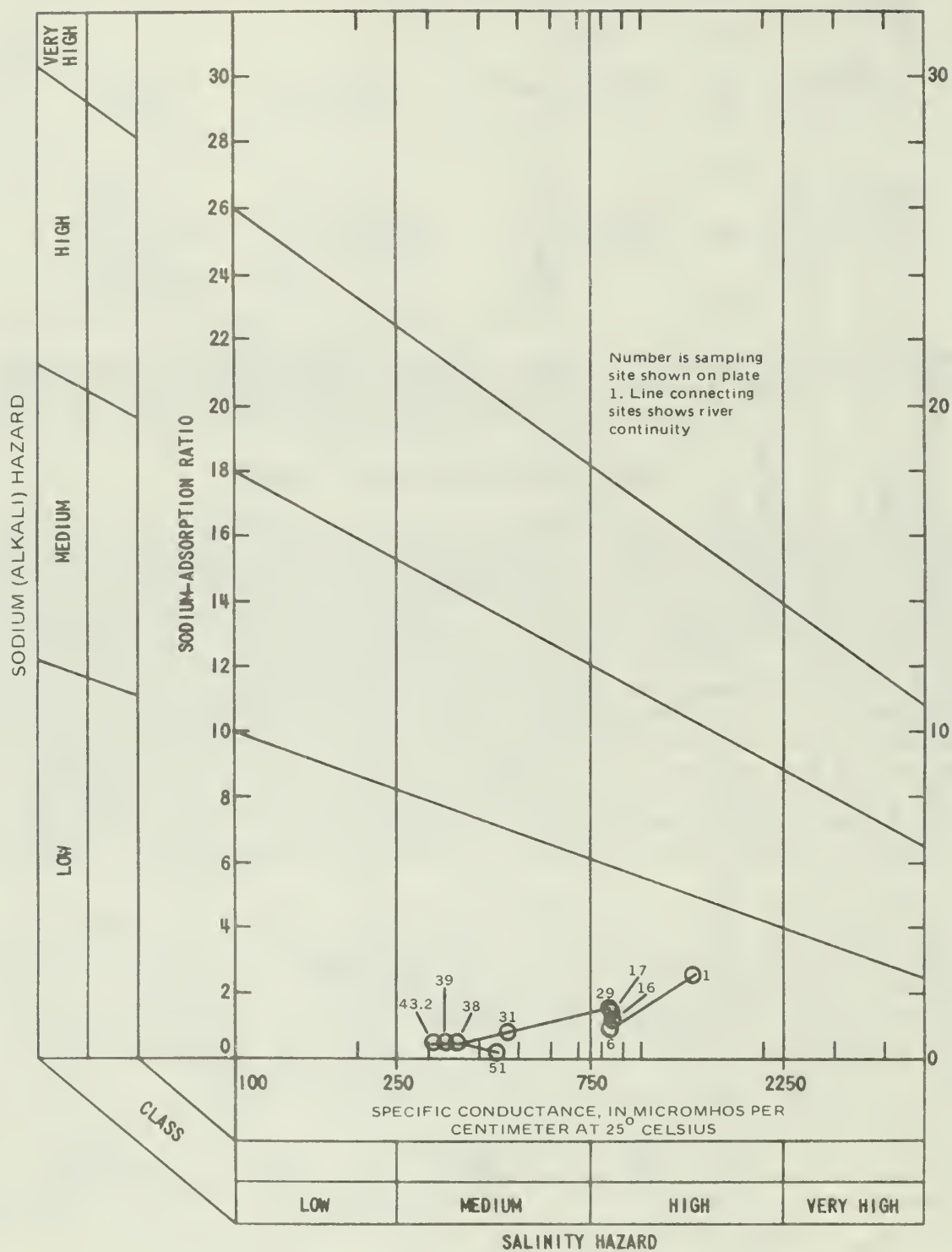
Figure 3.—Diagram showing classification of water for irrigation at selected sites on the Virgin River during high flow, May 3-11, 1982.
