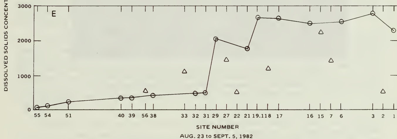
Figure 4.—Concentration of dissolved solids at selected sites—Continued.
