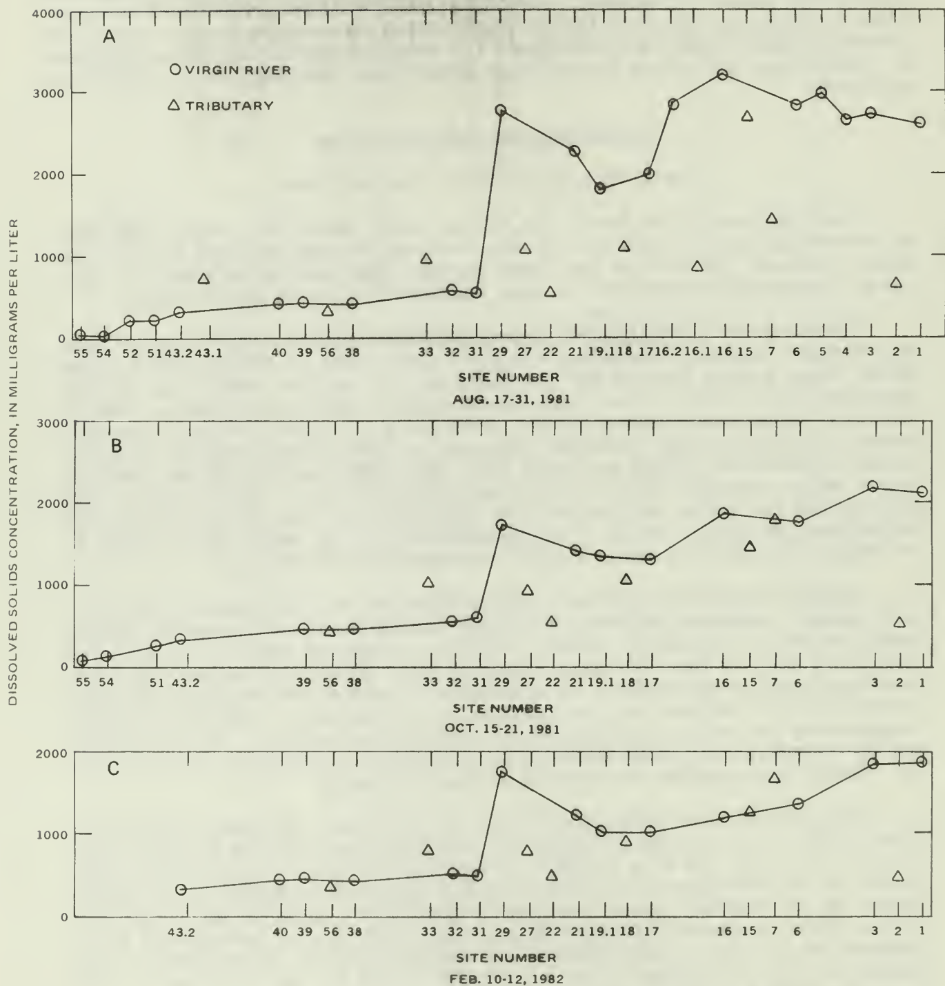
Figure 4.—Concentration of dissolved solids at selected sites.
