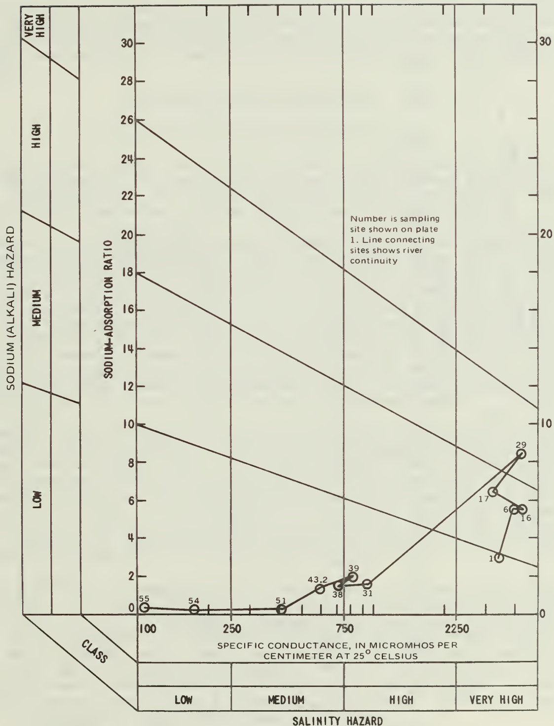
Figure 2.—Diagram showing classification of water for irrigation at selected sites on the Virgin River during low flow, August 17-31, 1981.
