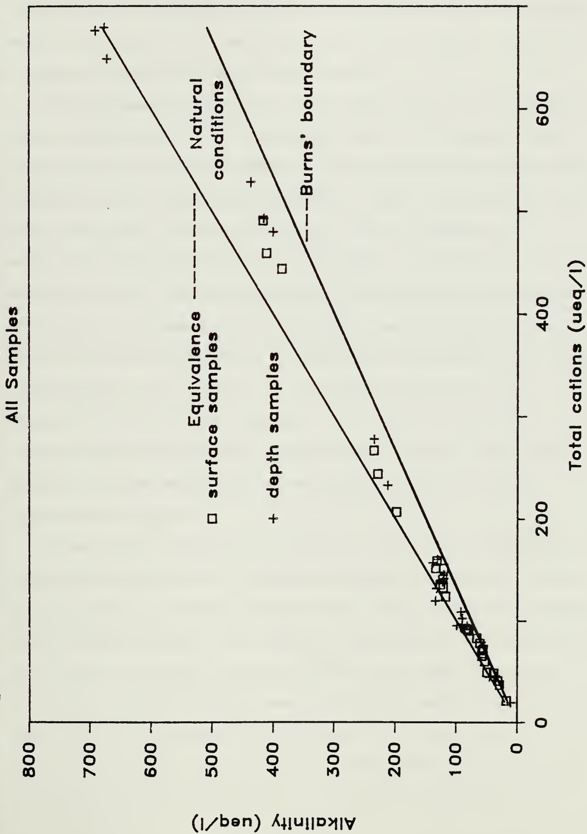
Figure 11. Alkalinity vs. Total Cations
