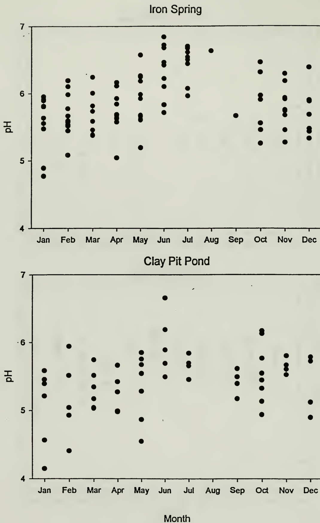
Figure 19. Monthly pH of Iron Spring and Clay Pit Pond, FOCL.
