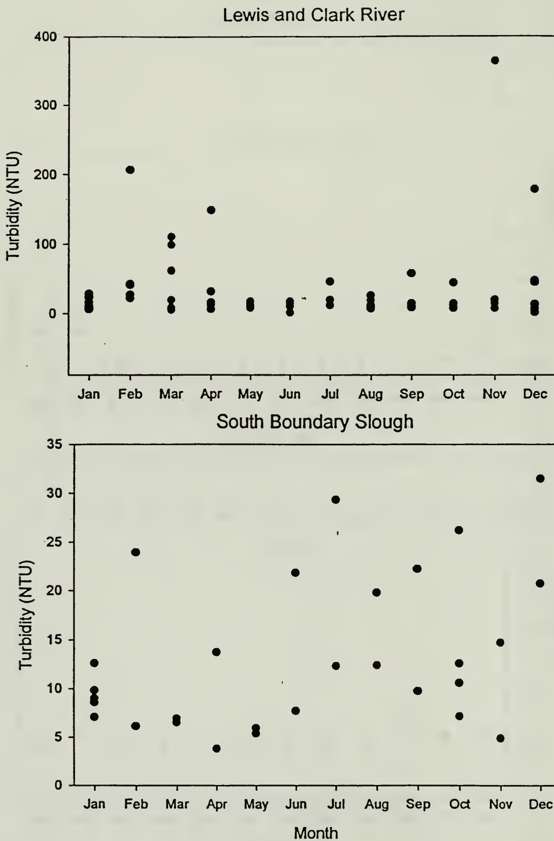
Figure 6. Monthly turbidities of the Lewis and Clark River and South Boundary Slough, FOCL.
