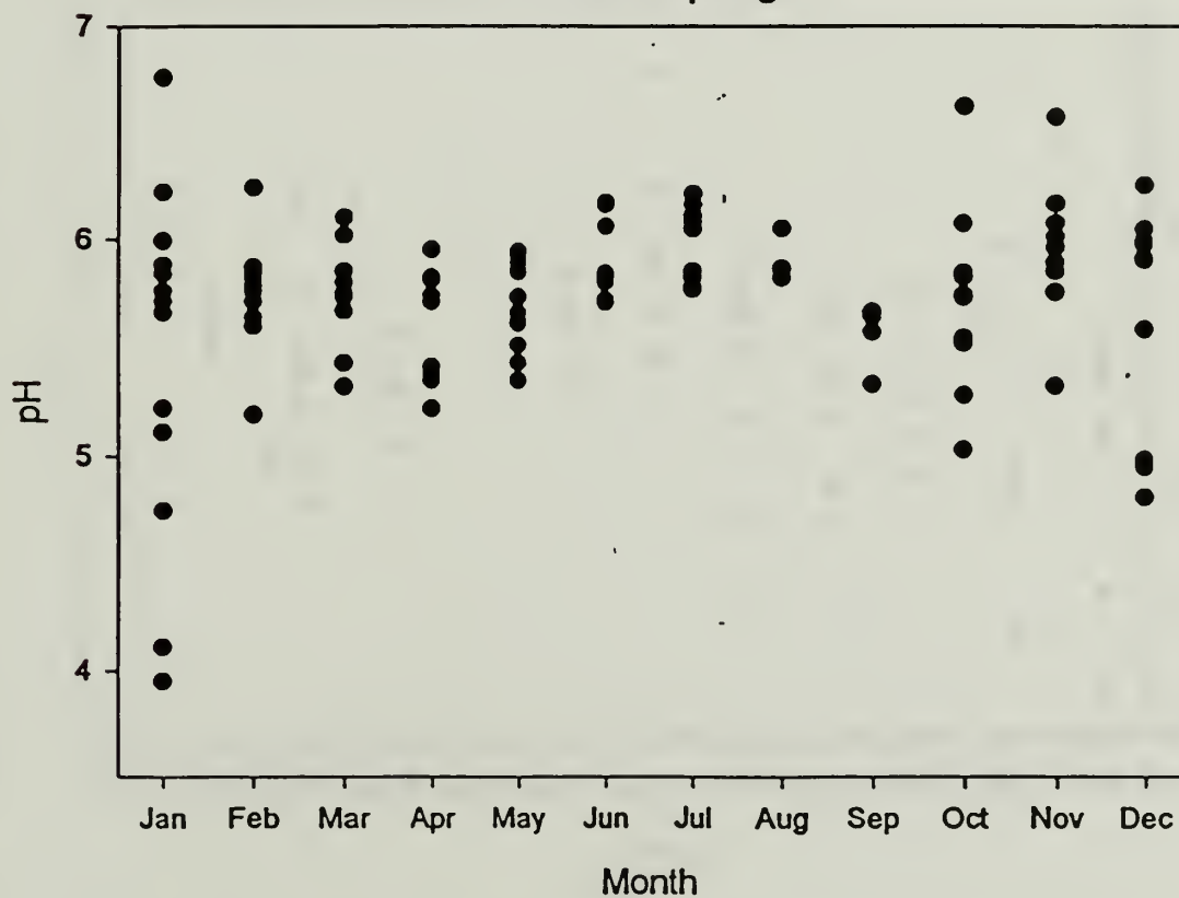
Figure 18. Monthly pH of Salamander Creek and Historic Spring, FOCL.
