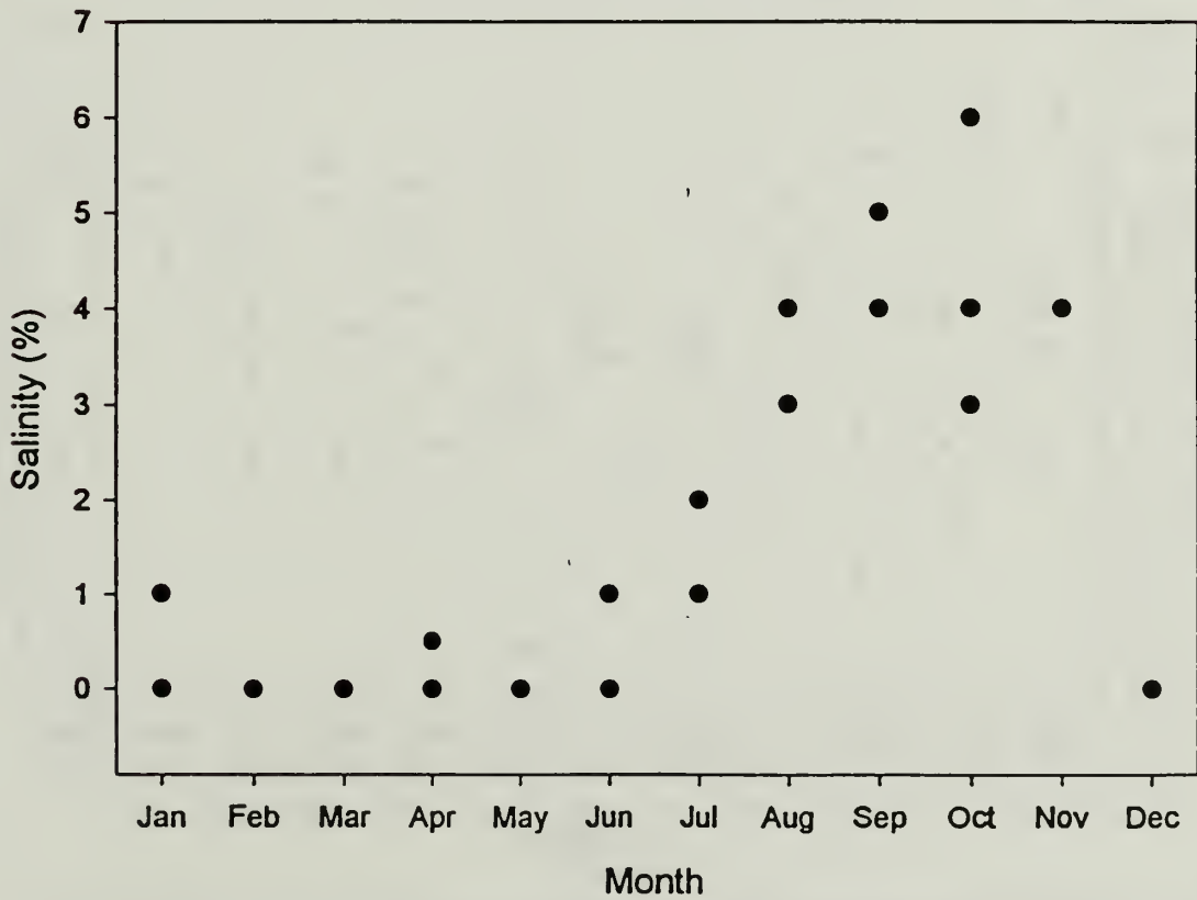
Figure 31. Monthly salinities of the Lewis and Clark River and South Boundary Slough, FOCL.
