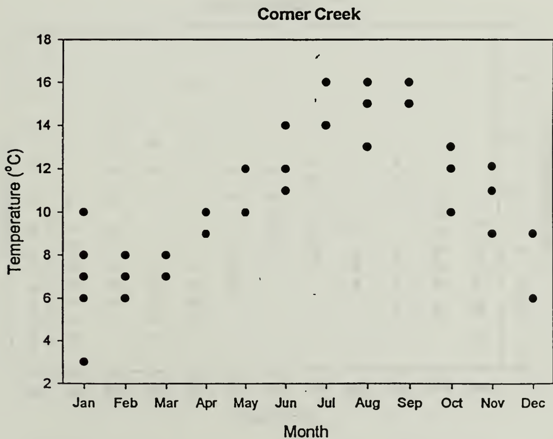
Figure 12. Monthly water temperatures of Alder Creek and Comer Creek, FOCL.
