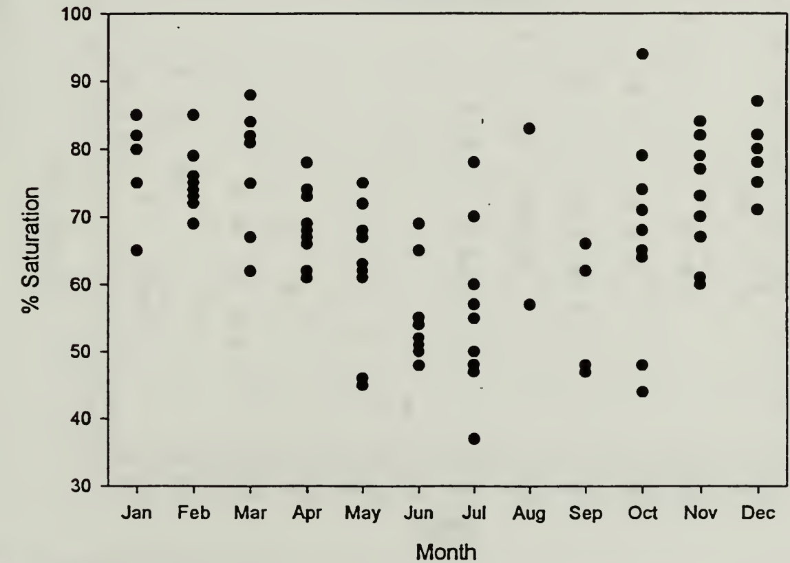
Figure 39. Monthly percent saturation of dissolved oxygen of Salamander Creek and Historic Spring, FOCL.
