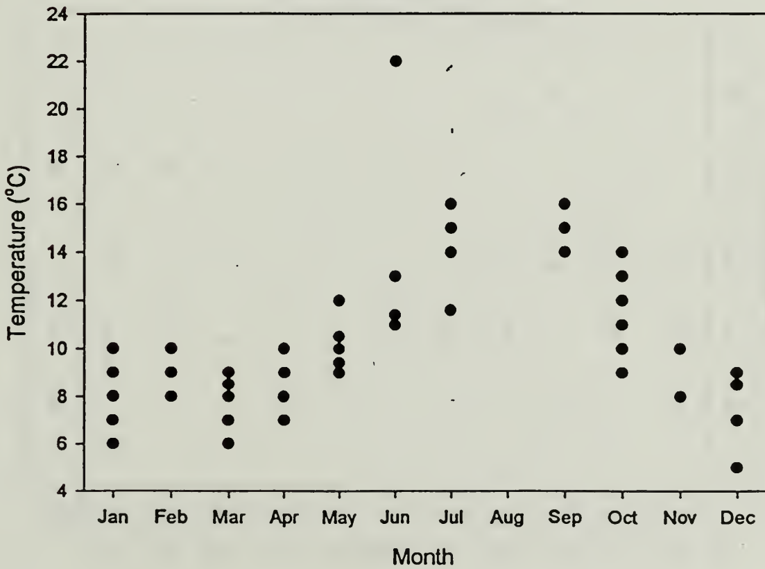
Figure 14. Monthly water temperatures of Iron Spring and Clay Pit Pond, FOCL.
