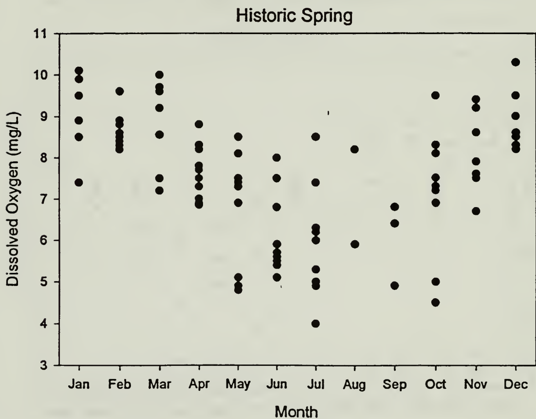
Figure 34. Monthly concentrations of dissolved oxygen of Salamander Creek and Historic Spring, FOCL.
