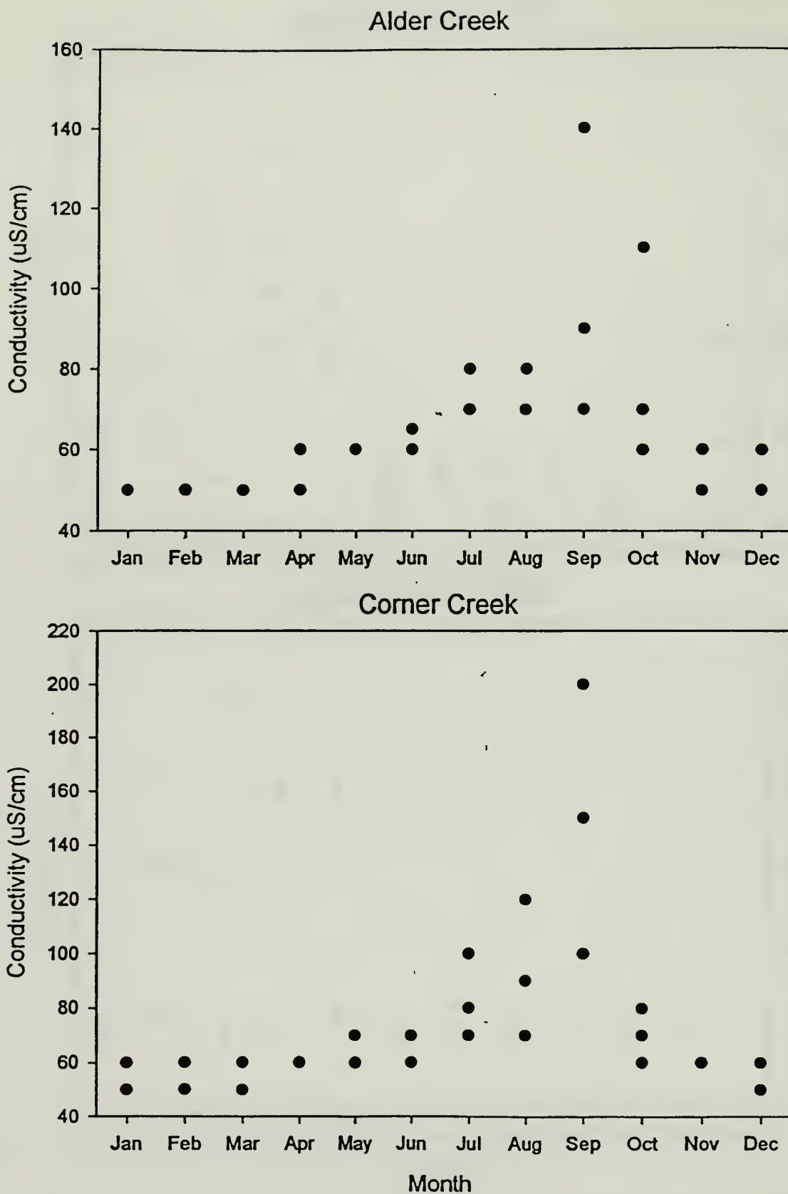
Figure 27. Monthly conductivities of Alder Creek and Corner Creek, FOCL.
