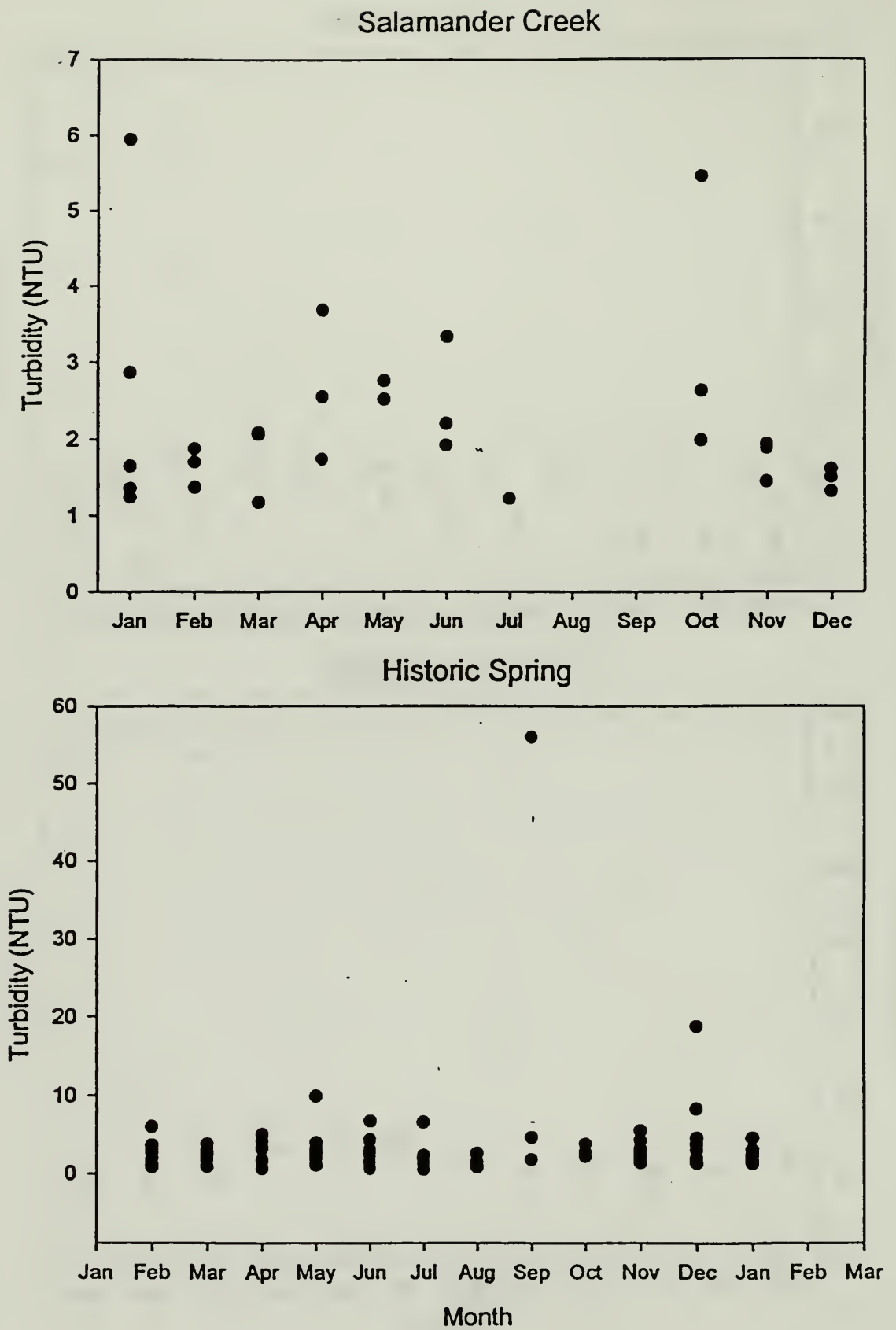
Figure 8. Monthly turbidities of Salamander Creek and Historic Spring, FOCL.
