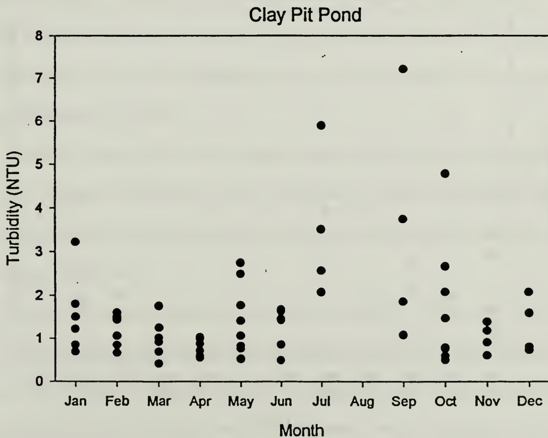
Figure 9. Monthly turbidities of Iron Spring and Clay Pit Pond, FOCL.
