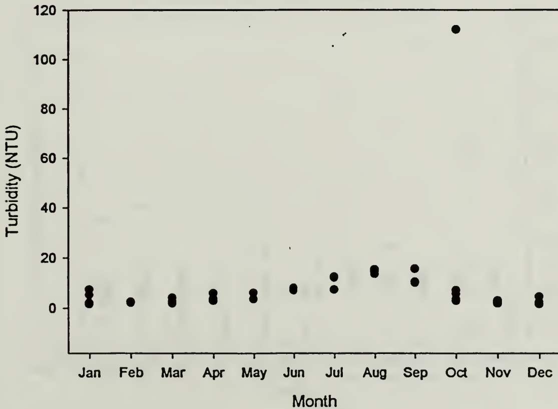
Figure 7. Monthly turbidities of Alder Creek and Comer Creek, FOCL.
