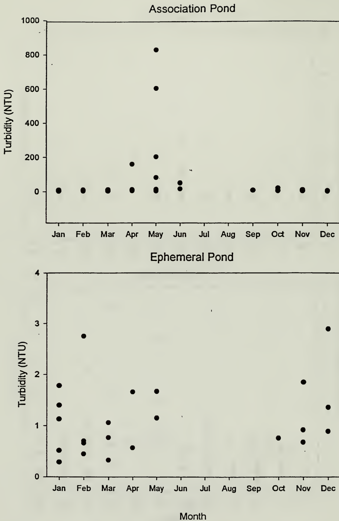
Figure 10. Monthly turbidities of Association Pond and Ephemeral Pond, FOCL.
