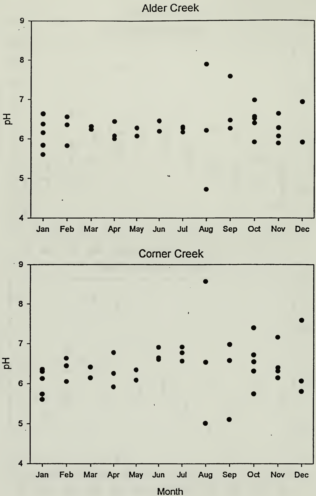
Figure 17. Monthly pH of Alder Creek and Corner Creek, FOCL.
