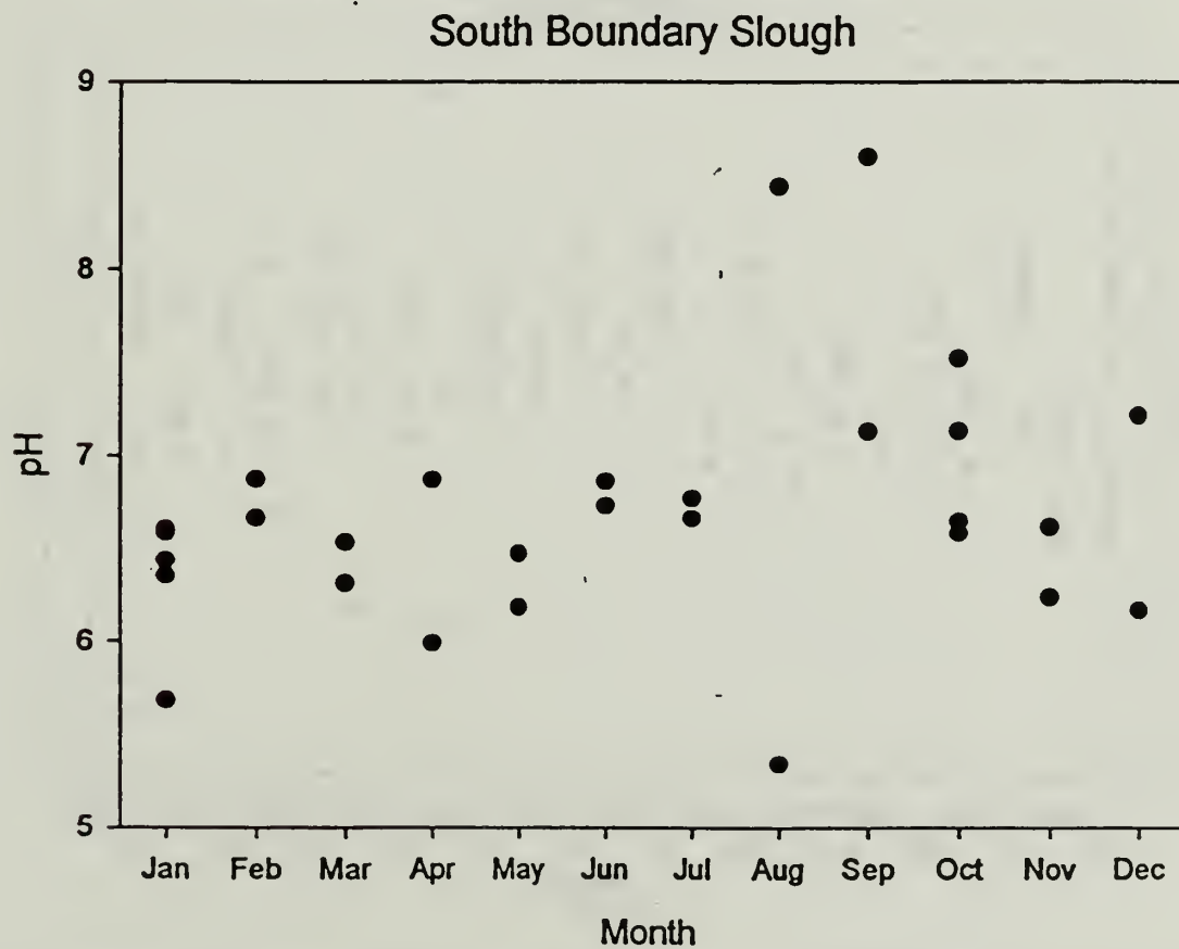
Figure 16. Monthly pH of the Lewis and Clark River and South Boundary Slough, FOCL.
