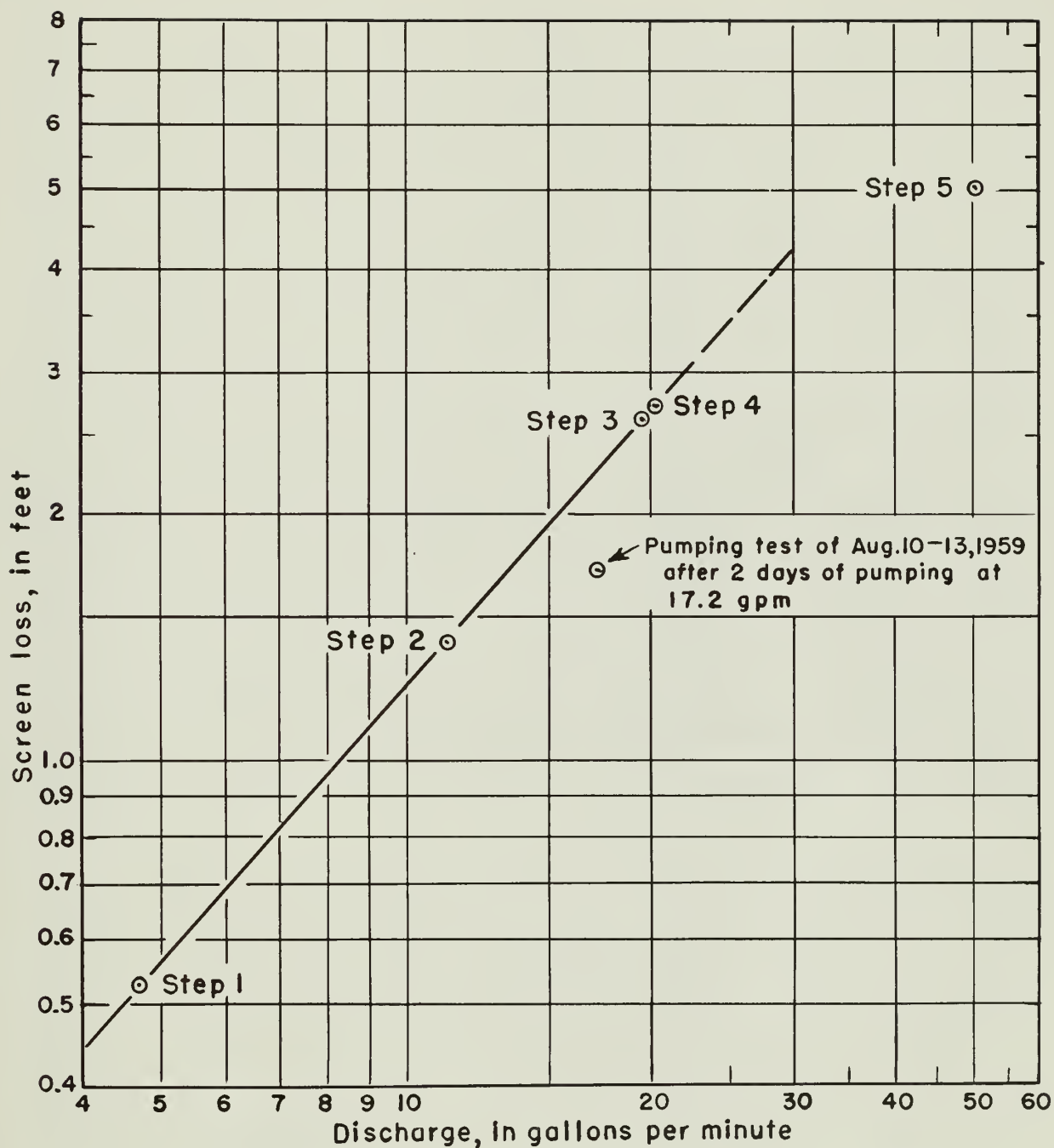
Figure III-17.--Log plot of screen loss versus discharge during the step-drawdown test of April 29, 1960.
