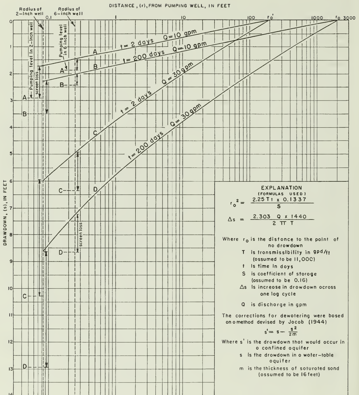
Figure 111-18.--Graphs of the predicted drawdowns that would be produced by a well drawing from the sand deposit in Saratoga National Historical Park and vicinity. (The drawdowns have been corrected for dewatering of the aquifer.)
