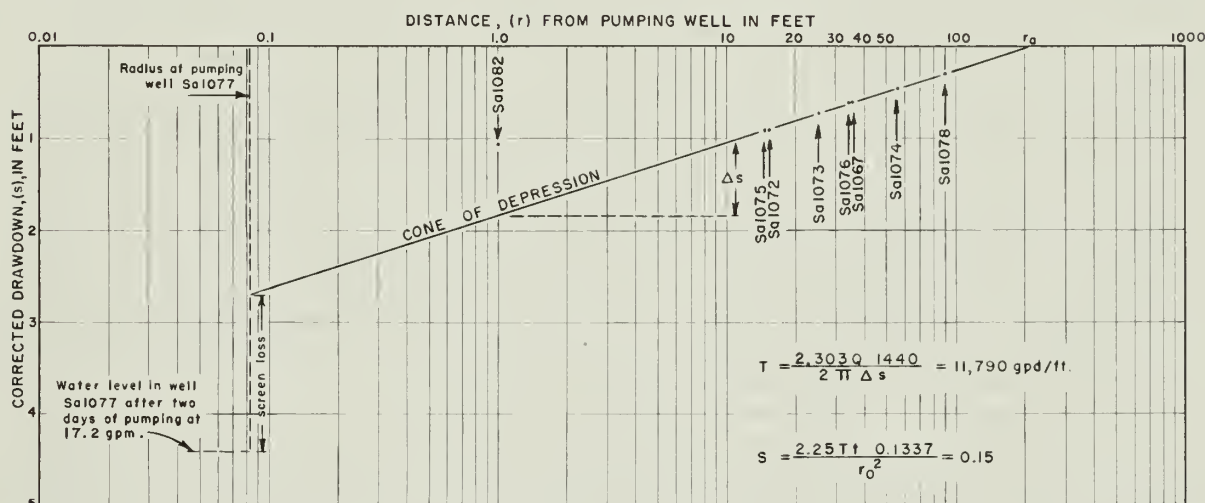
Figure III-15.--Graph of drawdowns versus log of distance from pumping well. (Measurements of drawdowns were made after 2 days of pumping at 17.2 gpm. The drawdowns are corrected for seasonal decline and dewatering of the aquifer.)
