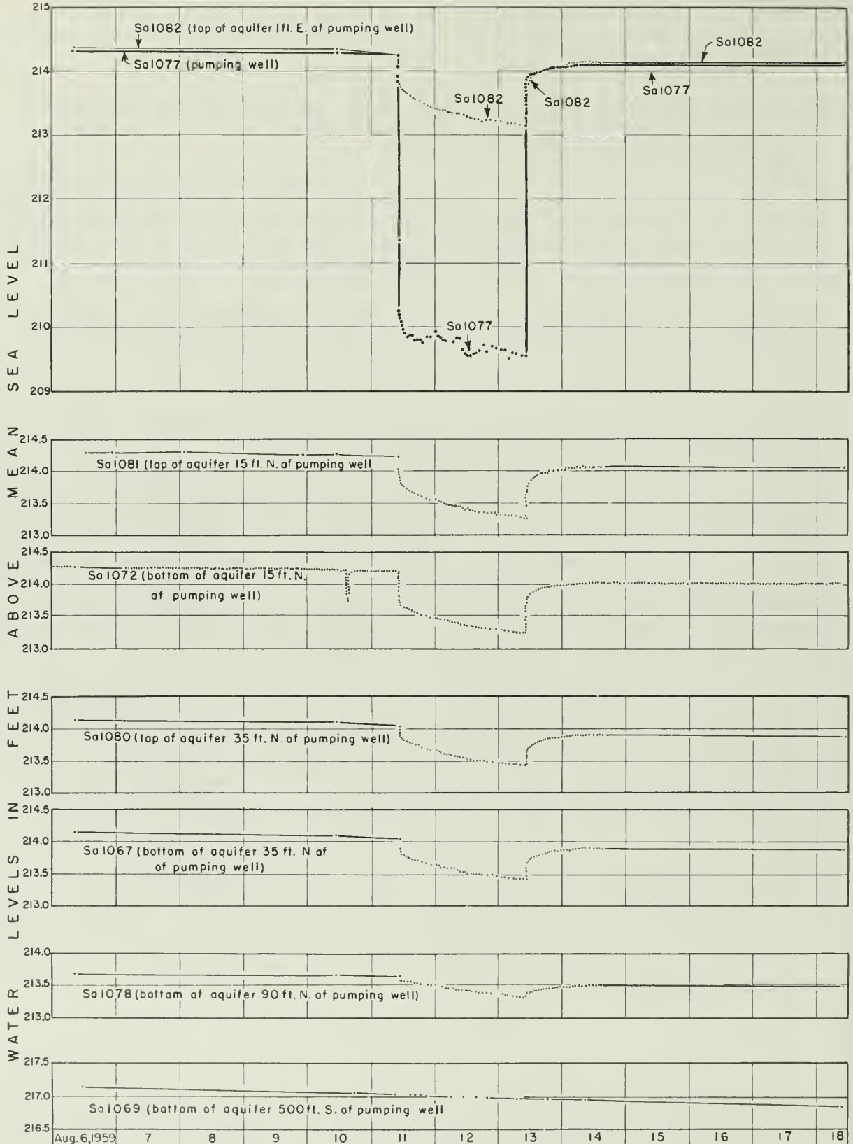
Figure III-13.--Hydrographs of the pumping well and selected observation wells in the vicinity of the Wilbur Spring ravine showing response of the water level during the pumping test of August 11-13, 1959. (Well Sa 1077 was pumped at a rate of 17.2 gpm from 10:47 a. m., August 11 to 10:25 a. m., August 13.)
