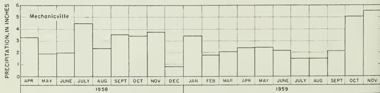
Figure III-8.--Graphs of the flow from the springs at the head of Wilbur Spring ravine, water levels in observation wells, and monthly precipitation at Mechanicville.
