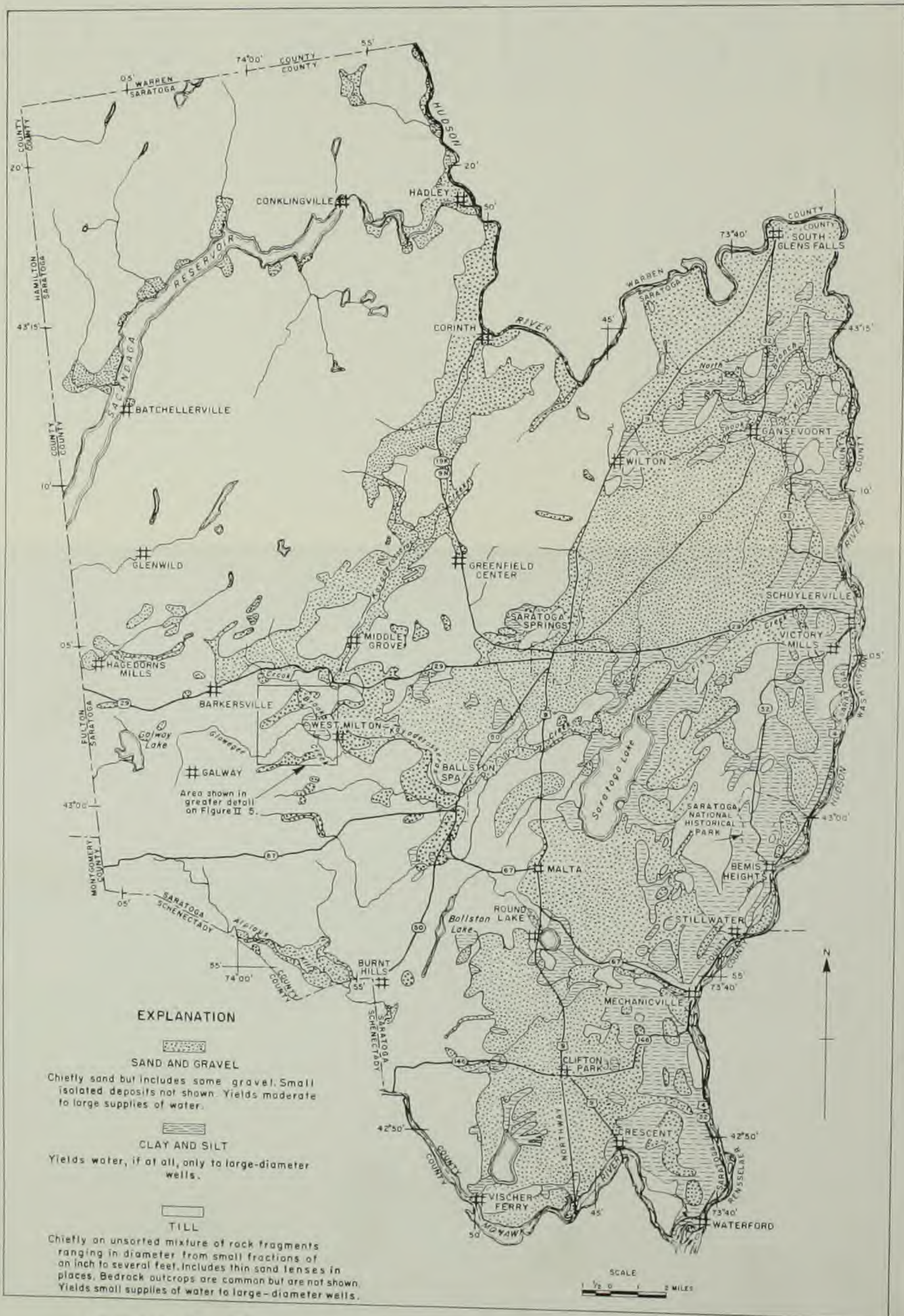
Figure 1-3.--Map of Saratoga County showing principal types of unconsolidated deposits.
