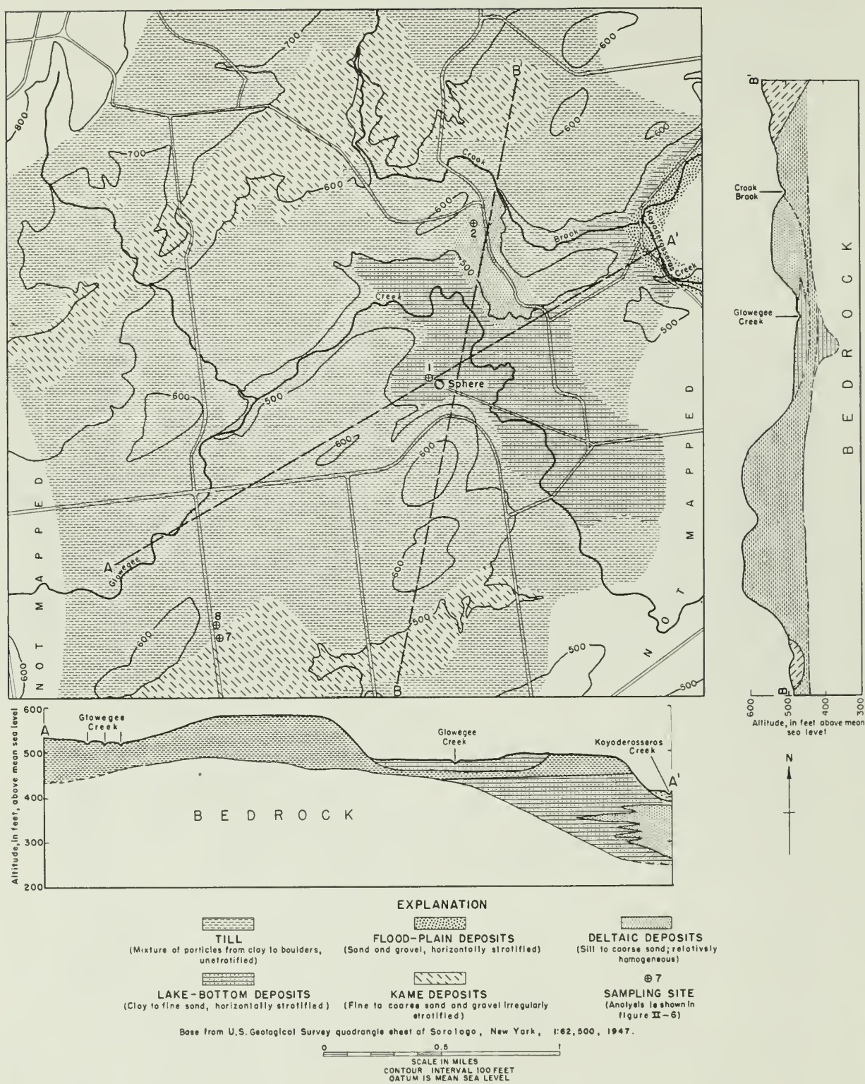
Figure 11-5.--Map and geologic sections showing unconsolidated deposits in a part of the West Milton area. (after Mack and others, fig. 6)
