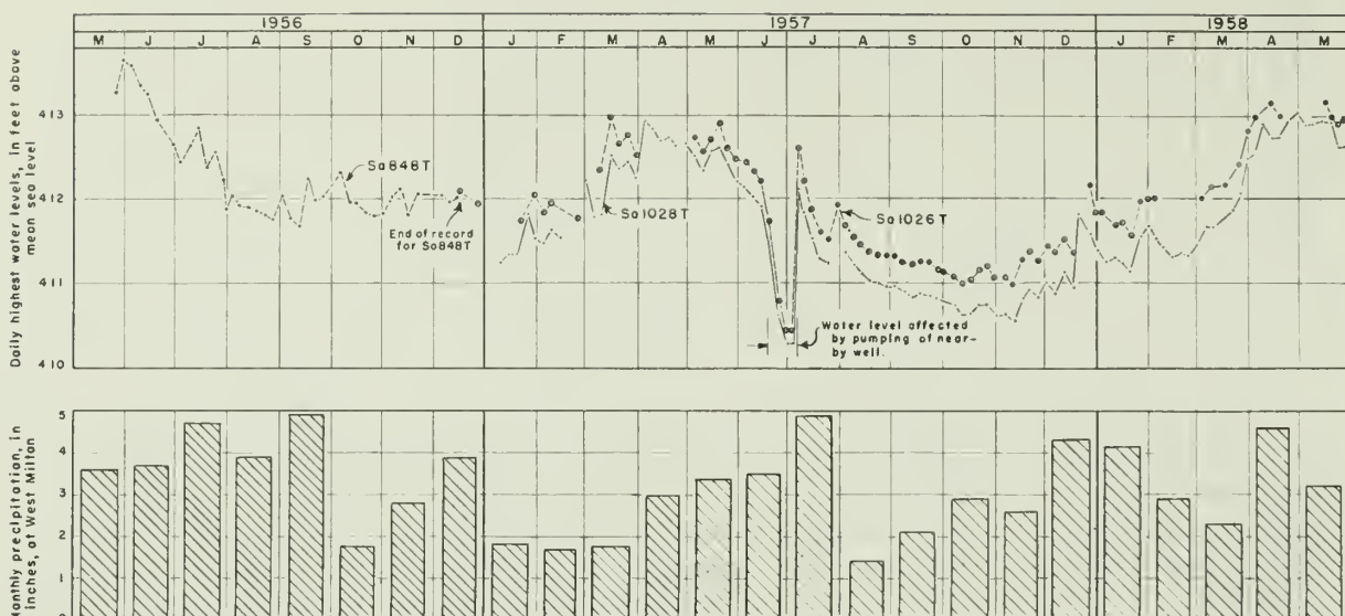
Figure 11-14.--Graphs showing fluctuations of the water levels in wells penetrating the artesian aquifer in the vicinity of Kayaderosseras Creek and monthly precipitation at West Milton.
