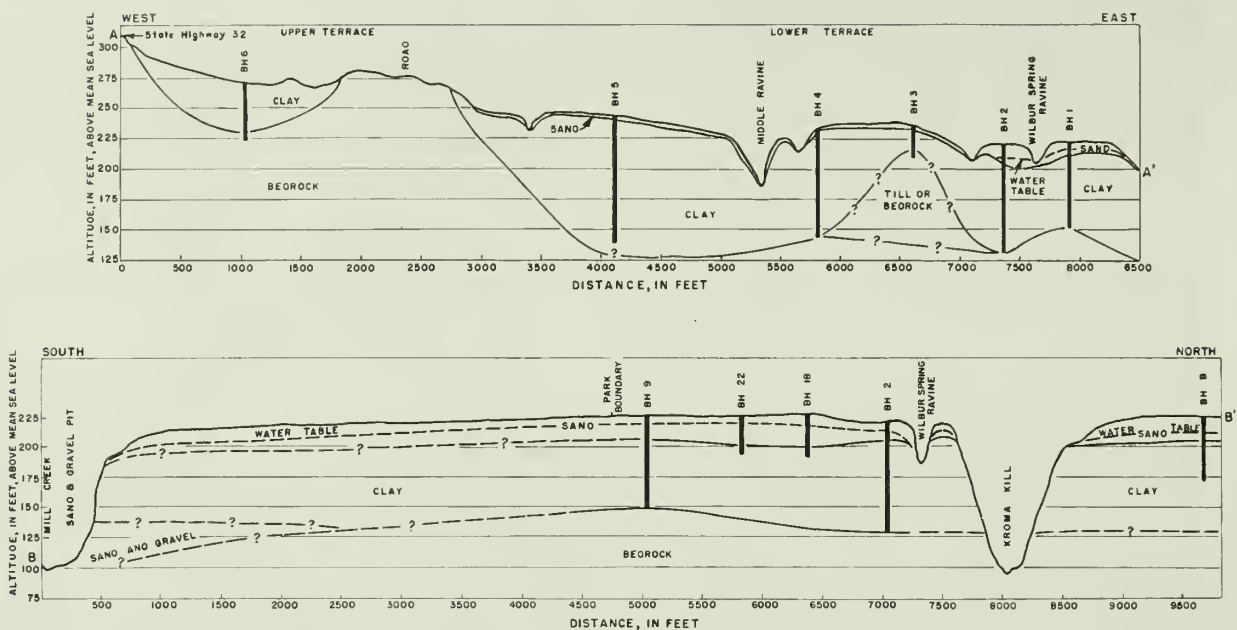
Figure 111-6.--Geologic sections in Saratoga National Historical Park along lines A-A' and B-B' in figure 111-1.
