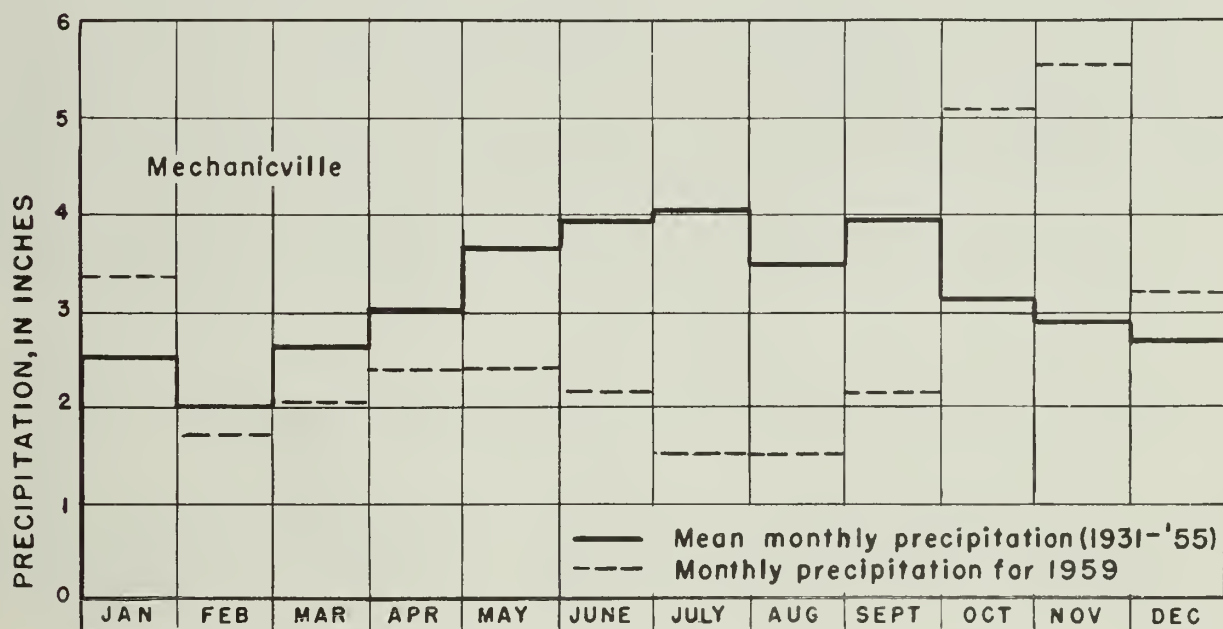
Figure III-2.--Normal monthly temperature at Saratoga Springs and monthly precipitation at Mechanicville.
