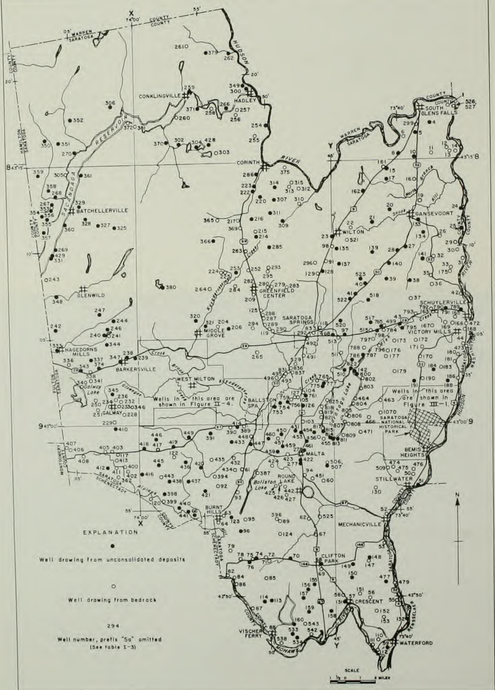
Figure 1-5.--Map of Saratoga County showing the location of selected wells and test holes.
