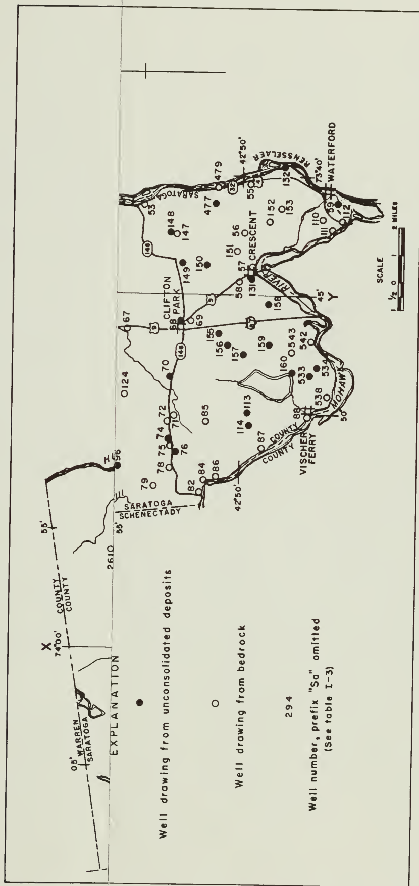
Figure 1-5.--Map of Saratoga County showing the location of selected wells and test holes.
