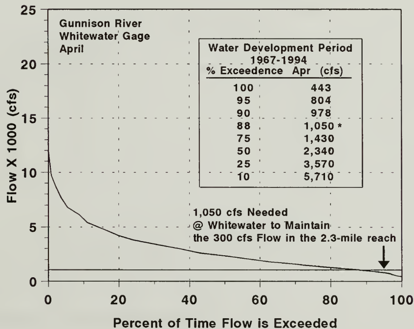
Figure H.2. Mean daily flow exceedences for March (top) and April (bottom) for the Gunnison River at the Whitewater USGS stream gage during the post-water development period, 1967-1994. The horizontal line at 1,050 represents the minimum amount of water (cfs) needed at the USGS stream gage at Whitewater to provide a minimum of 300 cfs in the 2.3-mile reach of the lower Gunnison River immediately downstream of Redlands Diversion Dam. This assumes that Redlands Canal withdraws at least 750 cfs from the river, thus 750+300=1,050 .
