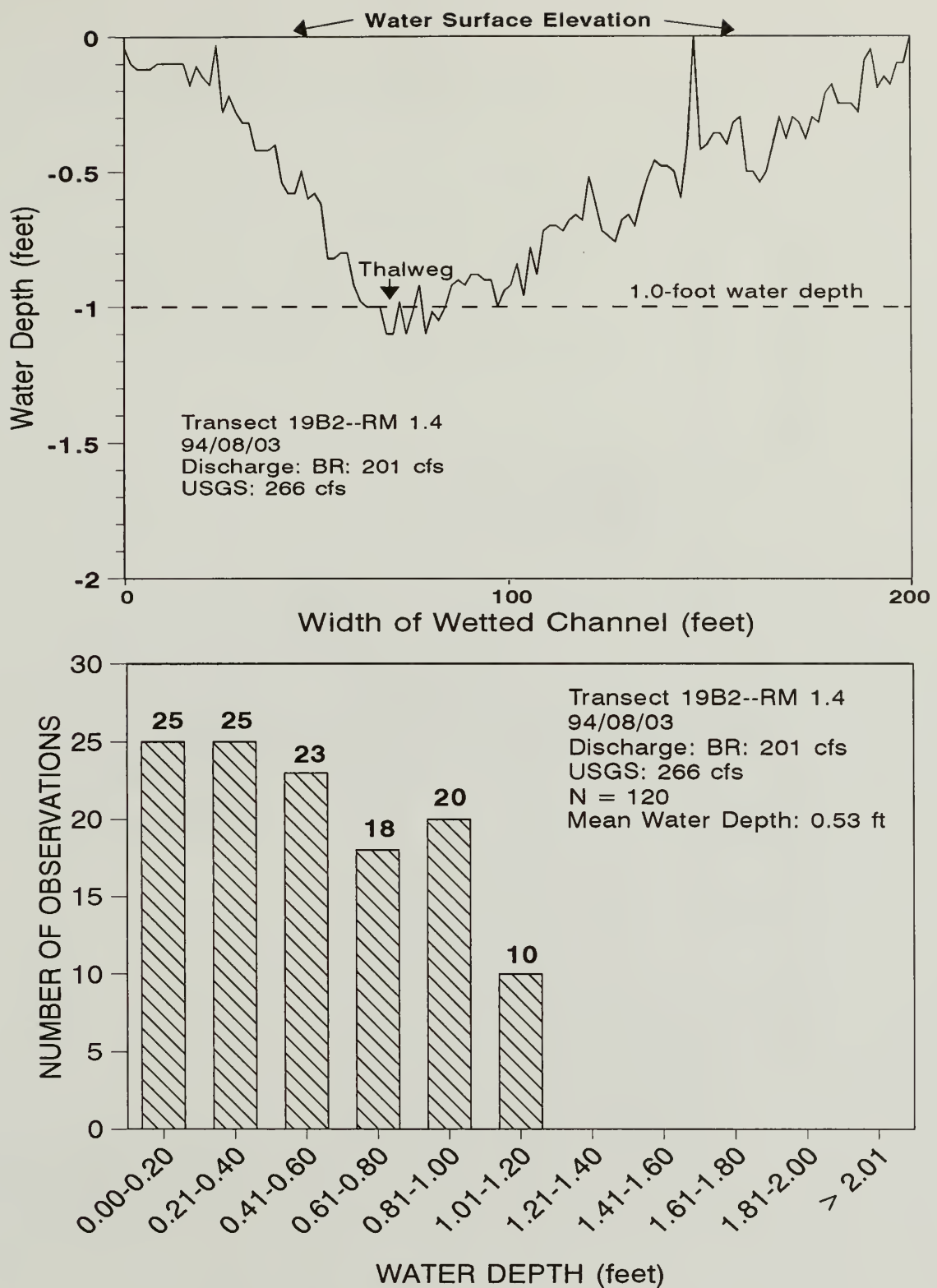
Figure G.12. River profile (top) and the distribution of water depths (feet) observed by 0.2-foot increments (bottom) for transect 19B2, river mile 1.4, Gunnison River, Colorado, 3 August 1994.
