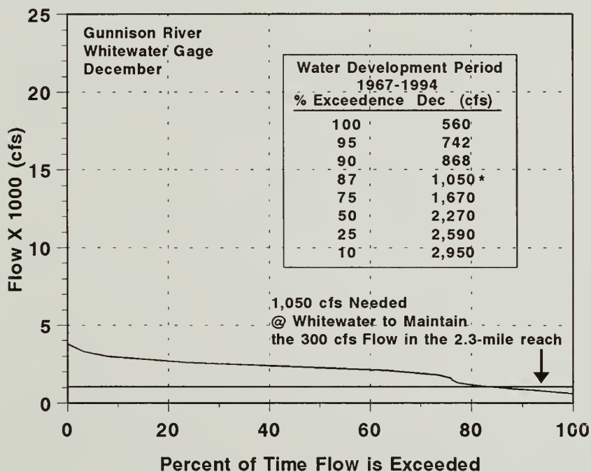
Figure H.6. Mean daily flow exceedences for November (top) and December (bottom) for the Gunnison River at the Whitewater USGS stream gage during the post-water development period, 1967-1994. The horizontal line at 1,050 represents the minimum amount of water (cfs) needed at the USGS stream gage at Whitewater to provide a minimum of 300 cfs in the 2.3-mile reach of the lower Gunnison River immediately downstream of Redlands Diversion Dam. This assumes that Redlands Canal withdraws at least 750 cfs from the river, thus 750+300=1,050 .
