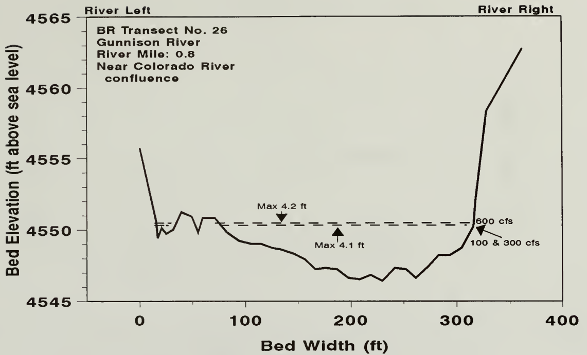
Figure G.6. River profile and variation in stage and maximum depth at various flow levels (100, 300, and 600 cfs) at Transect 26. Transect conducted by BR personnel.
