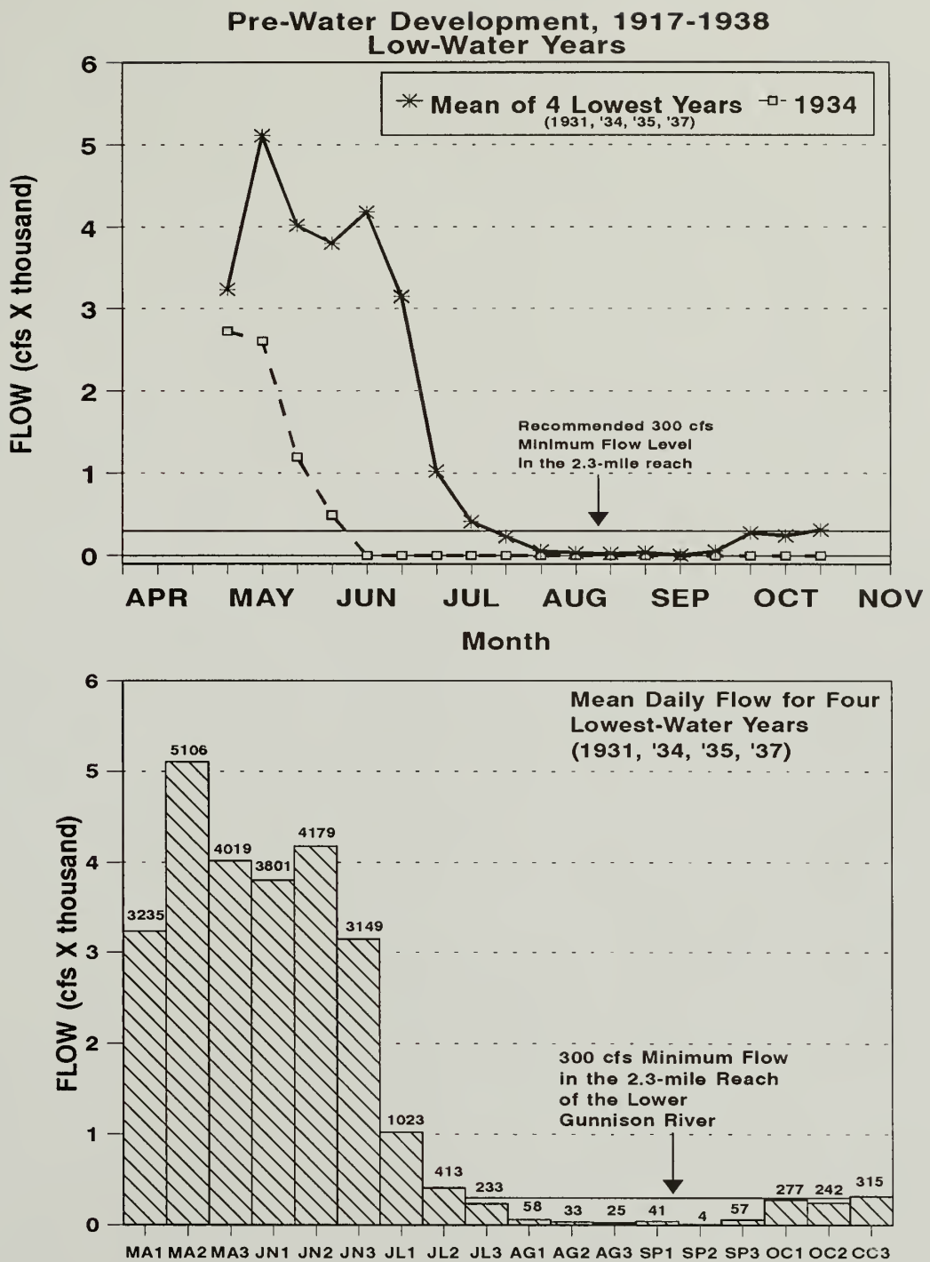
Figure I.1. Mean daily flow (cfs) and shape of the hydrograph for four lowest-water years (1931, 1934, 1935, and 1937) compared to 1934, a low, low-water year from 1 May to 31 October in the 2.3-mile reach of the lower Gunnison River between the Redlands Diversion Dam and the confluence with the Colorado River. The bottom figure represents the mean daily flow for 1 May through 31 October for the 2.3-mile reach by 10- and 11-day step increments, e.g., May 1-10, May 11-20, May 21-31, etc.
