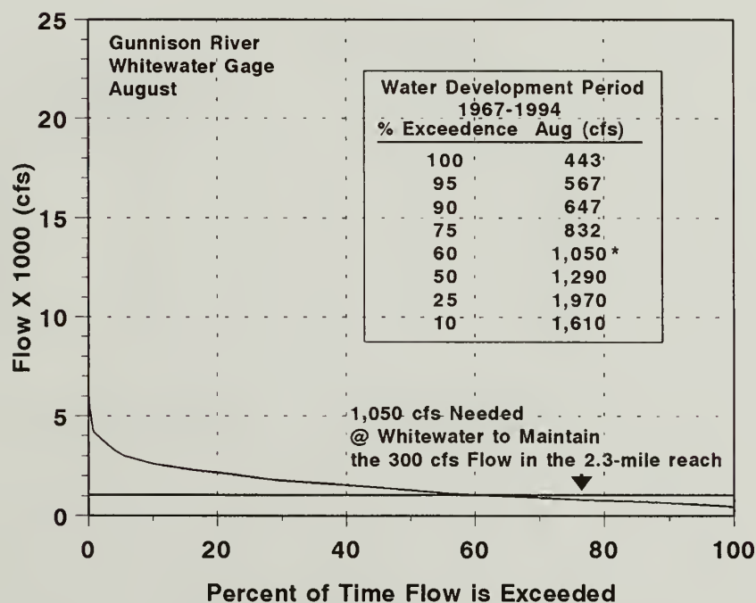
Figure H.4. Mean daily flow exceedences for July (top) and August (bottom) for the Gunnison River at the Whitewater USGS stream gage during the post-water development period, 1967-1994. The horizontal line at 1,050 represents the minimum amount of water (cfs) needed at the USGS stream gage at Whitewater to provide a minimum of 300 cfs in the 2.3-mile reach of the lower Gunnison River immediately downstream of Redlands Diversion Dam. This assumes that Redlands Canal withdraws at least 750 cfs from the river, thus 750+300=1,050 .
