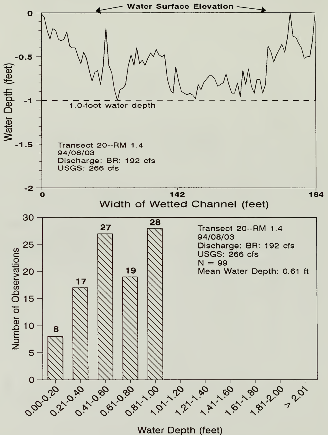
Figure G.13. River profile (top) and the distribution of water depths (feet) observed by 0.2-foot increments (bottom) for transect 20, river mile 1.4, Gunnison River, Colorado, 3 August 1994.
