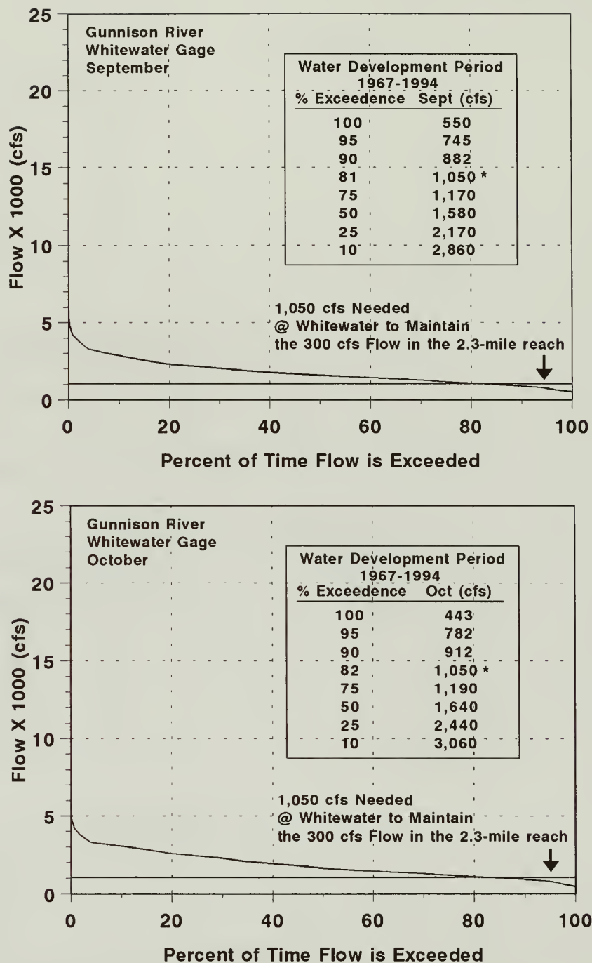
Figure H.5. Mean daily flow exceedences for September (top) and October (bottom) for the Gunnison River at the Whitewater USGS stream gage during the post-water development period, 1967-1994. The horizontal line at 1,050 represents the minimum amount of water (cfs) needed at the USGS stream gage at Whitewater to provide a minimum of 300 cfs in the 2.3-mile reach of the lower Gunnison River immediately downstream of Redlands Diversion Dam. This assumes that Redlands Canal withdraws at least 750 cfs from the river, thus 750+300=1,050 .
