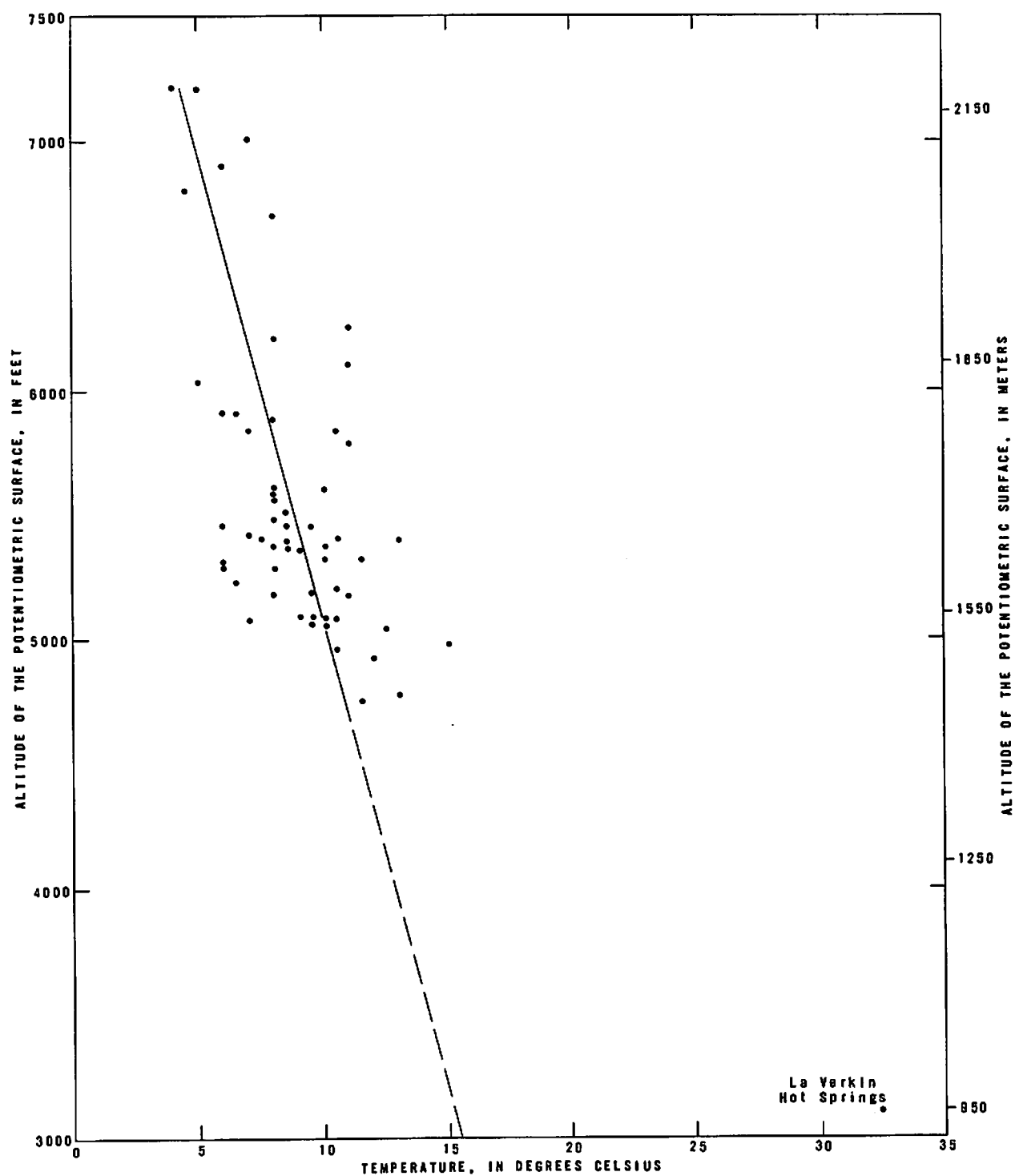
Figure 16.— Relation of ground-water temperature to the altitude of the potentiometric surface.
