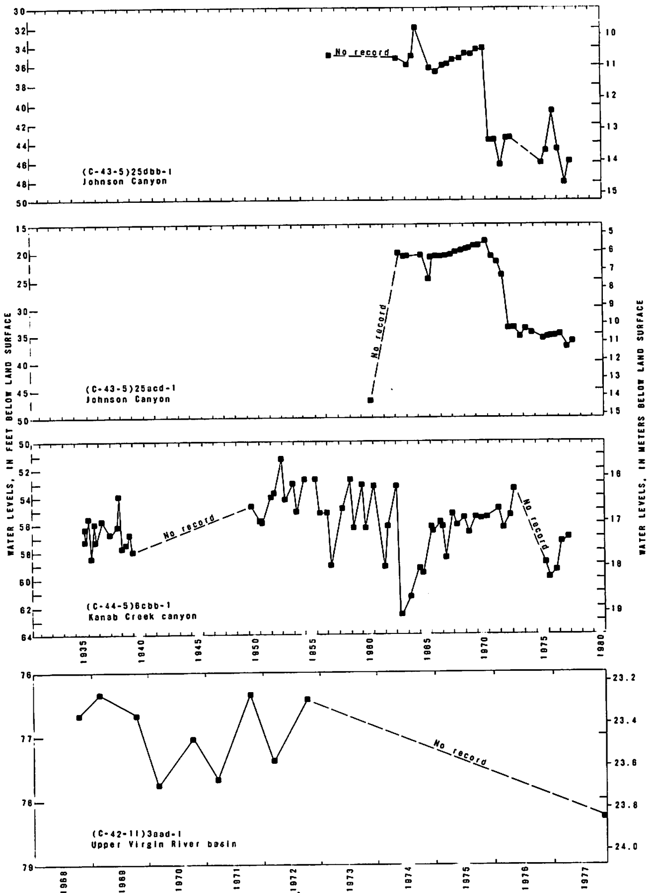
Figure 10.— Water-level fluctuations in selected wells in the study area.
