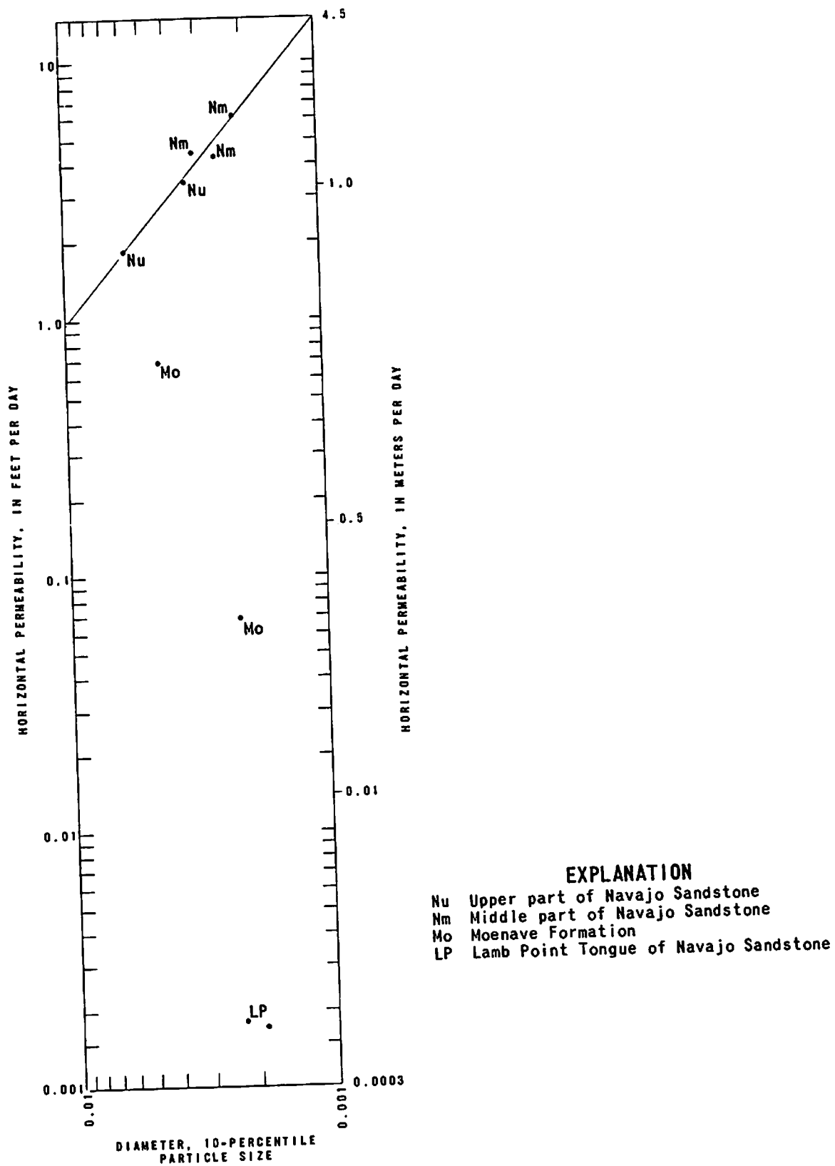
Figure 8.—Relation of horizontal permeability to the 10-percentile particle-size diameter of selected rock samples.
