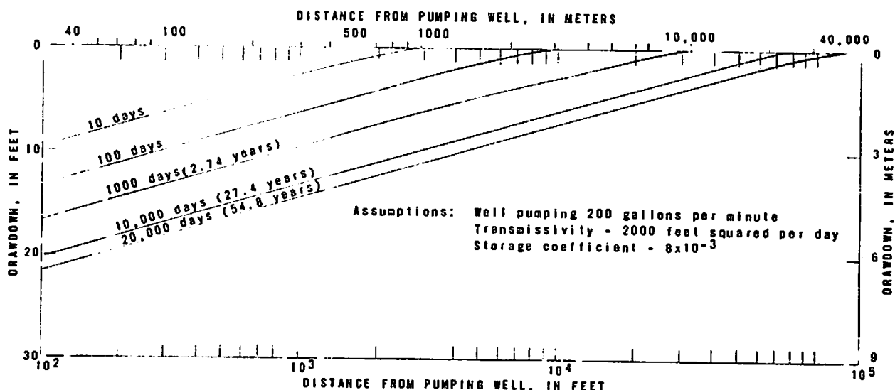
Figure 18.—Theoretical relation between drawdown and distance from a pumping well tapping mainly the Shinarump Member of the Chinle Formation for selected pumping durations.
