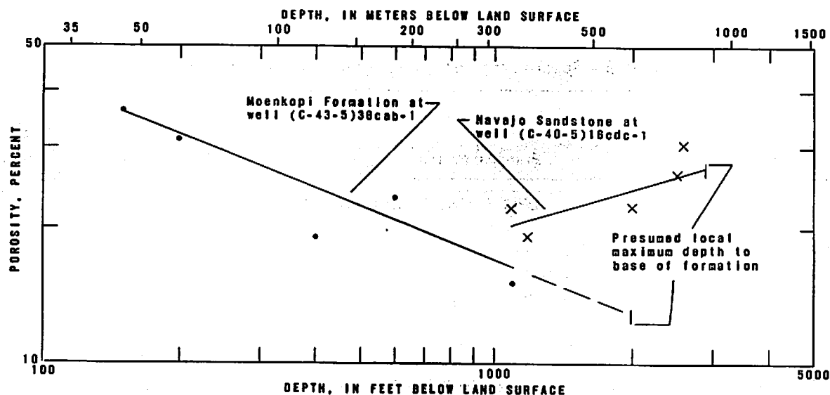
Figure 7.—Relation between porosity and depth for two aquifers in the upper Kanab Creek basin.
