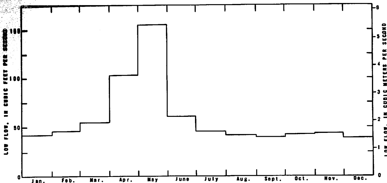
Figure 5.— Average monthly low flow (1937-76) of the North Fork Virgin River at site (C-41-10)22bc.
