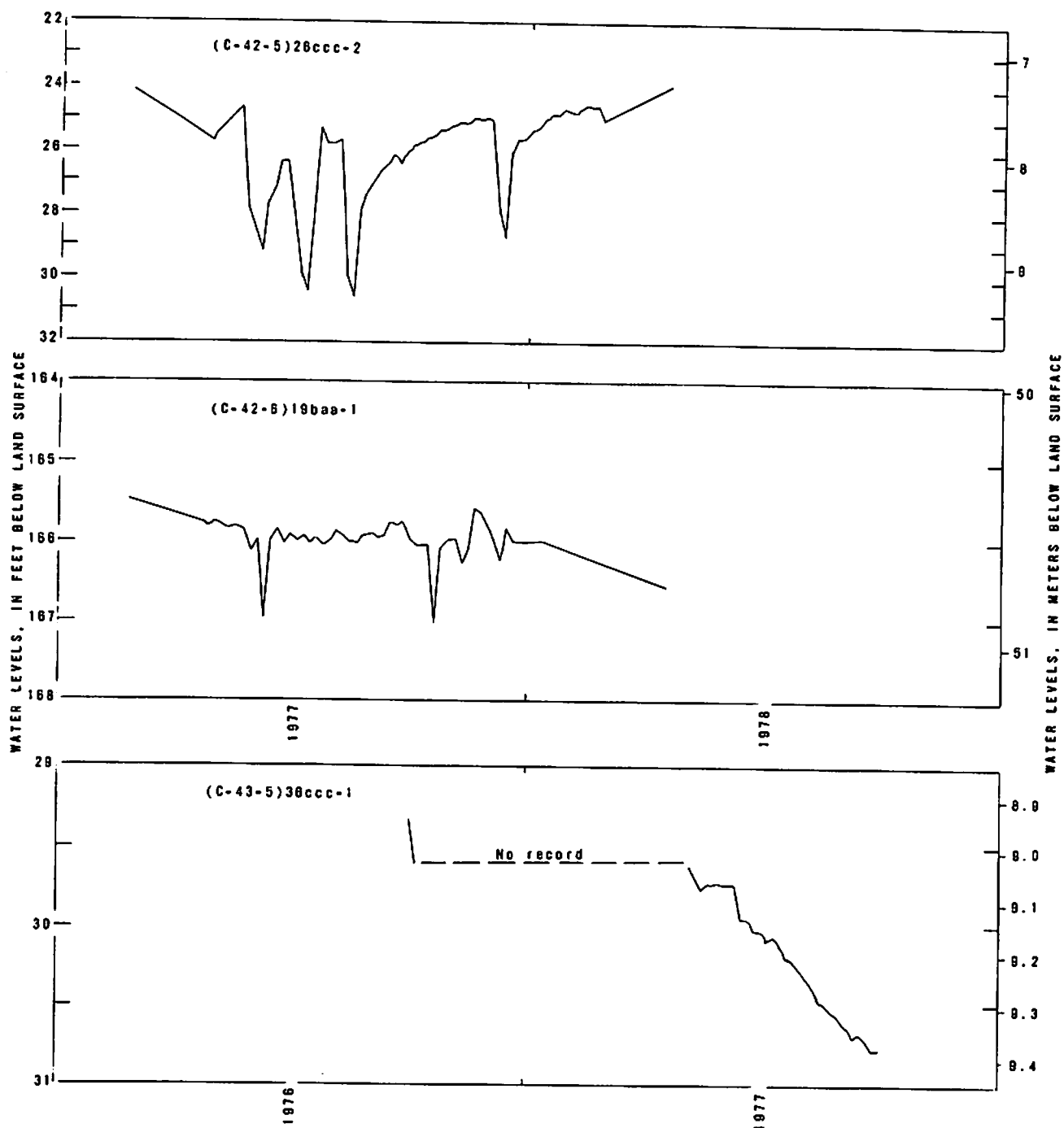
Figure 11.— Water-level fluctuations (1976-78) in selected wells in the upper Kanab Creek basin.
