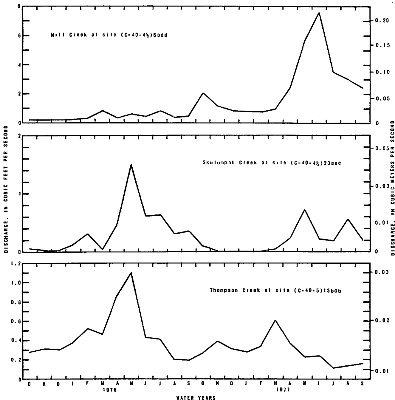
Figure 4.— Streamflow hydrographs of Mill, Skutumpah, and Thompson Creeks, 1976 and 1977 water years.
