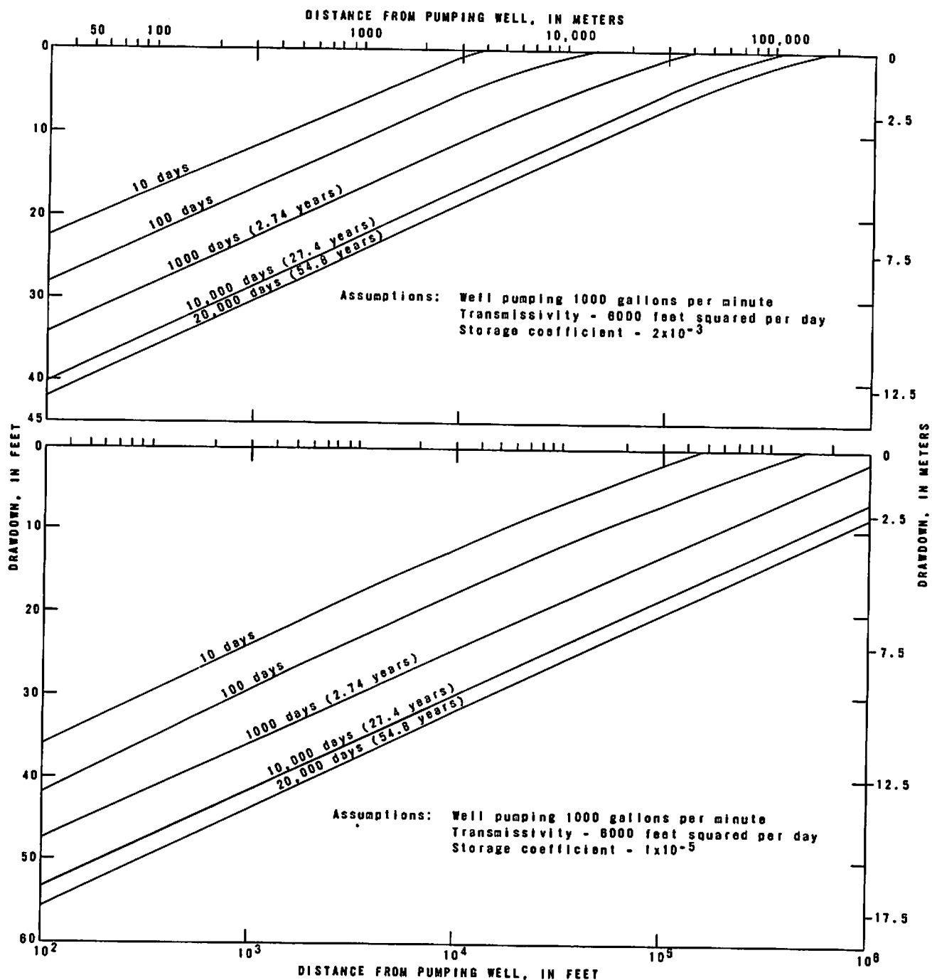
Figure 17.—Theoretical relation between drawdown and distance from a pumping well in the Navajo Sandstone for selected pumping durations.
