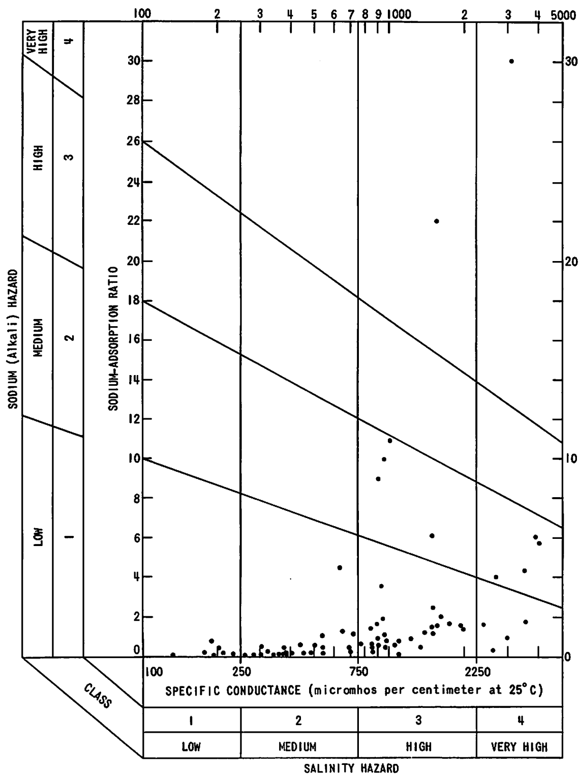
Figure 15.— Classification for irrigation of selected ground-water samples from the study area. (Classification after a method of the U.S. Salinity Laboratory Staff, 1954.)
