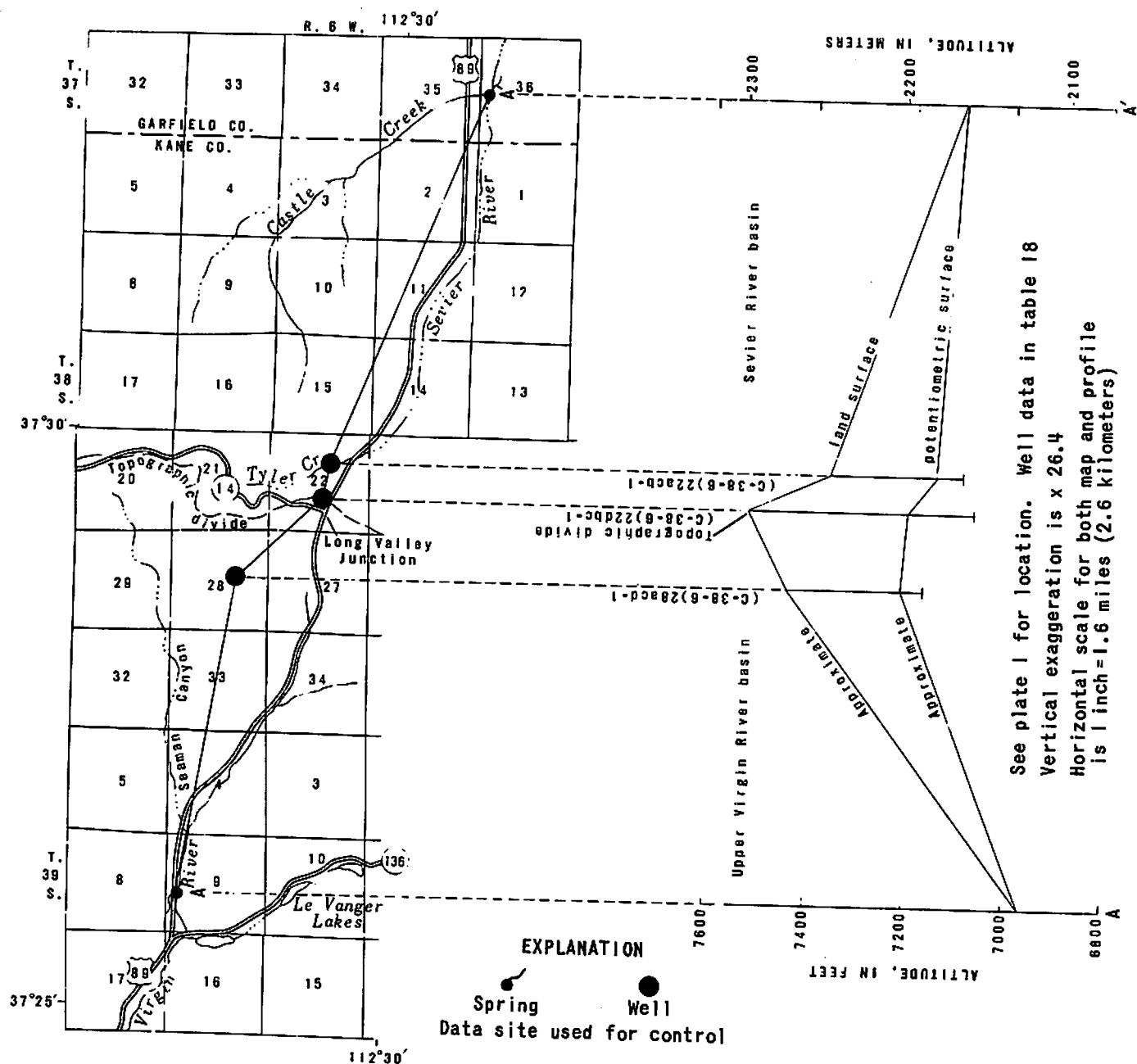
Figure 9.—Profile of the potentiometric surface at the divide between the upper Virgin River and Sevier River basins.
