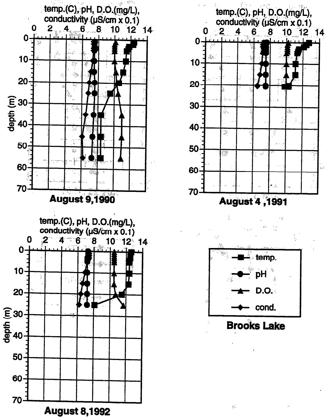
Figure 7. Depth profiles of water quality characteristics, Brooks Lake.
