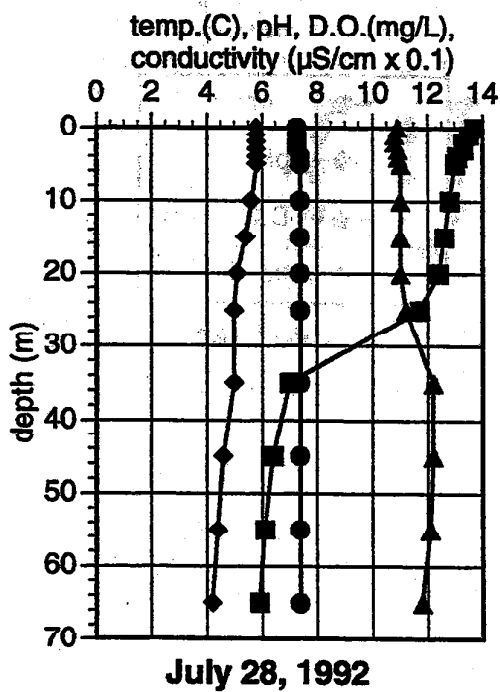
Figure 9. Depth profiles of water quality characteristics, Grosvenor Lake.
