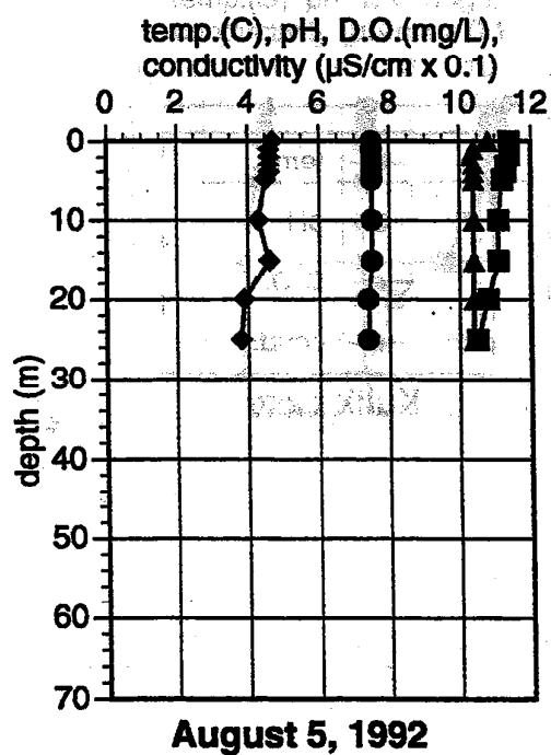
Figure 12. Depth profiles of water quality characteristics, Kukaklek Lake.
