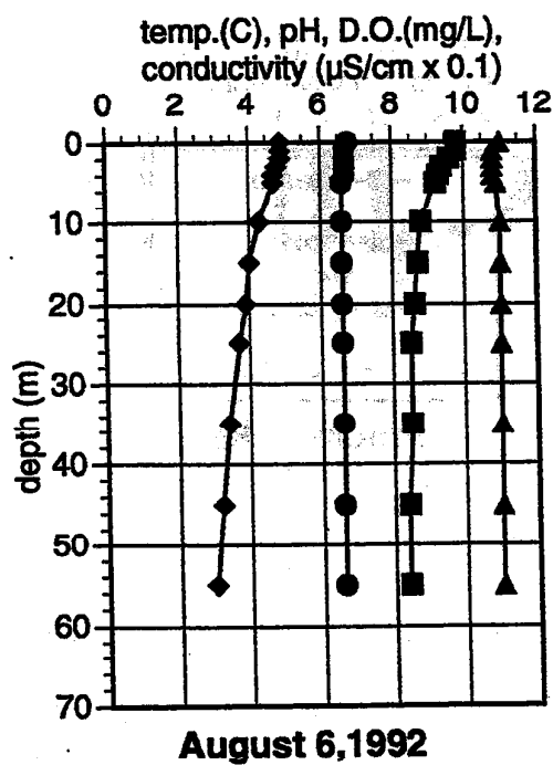
Figure 6. Depth profiles of water quality characteristics, Battle Lake.
