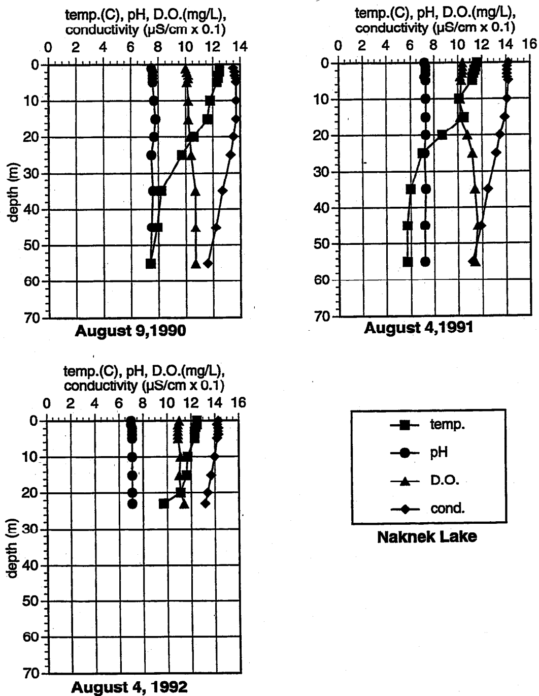
Figure 15. Depth profiles of water quality characteristics, Naknek Lake.
