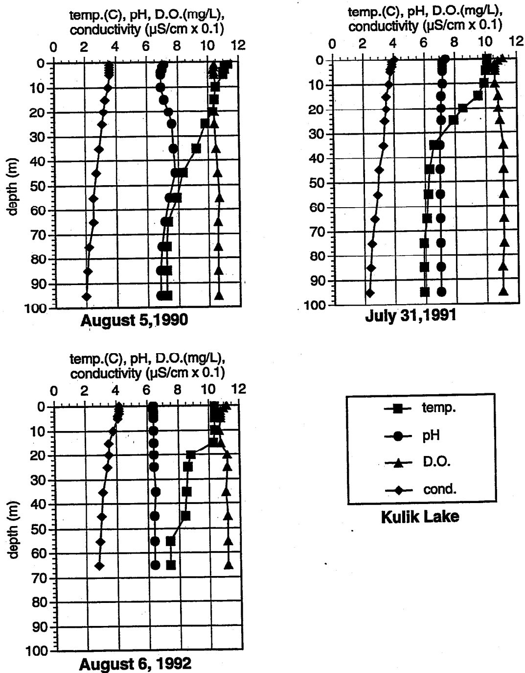
Figure 13. Depth profiles of water quality characteristics, Kulik Lake.
