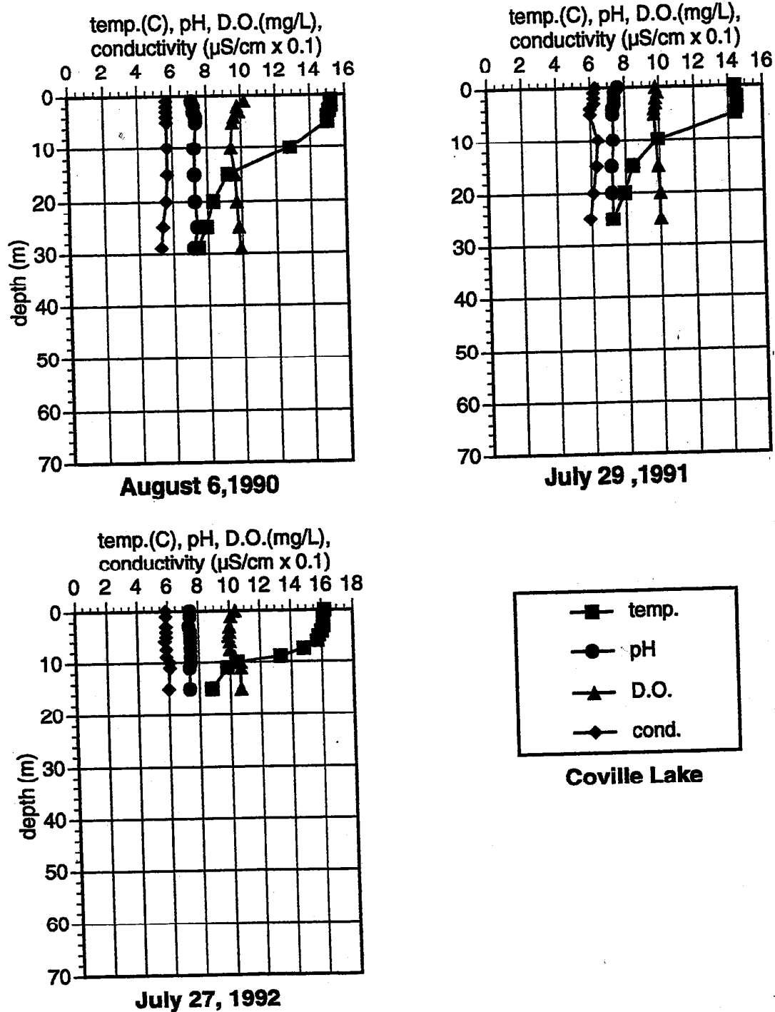
Figure 8. Depth profiles of water quality characteristics, Coville Lake.
