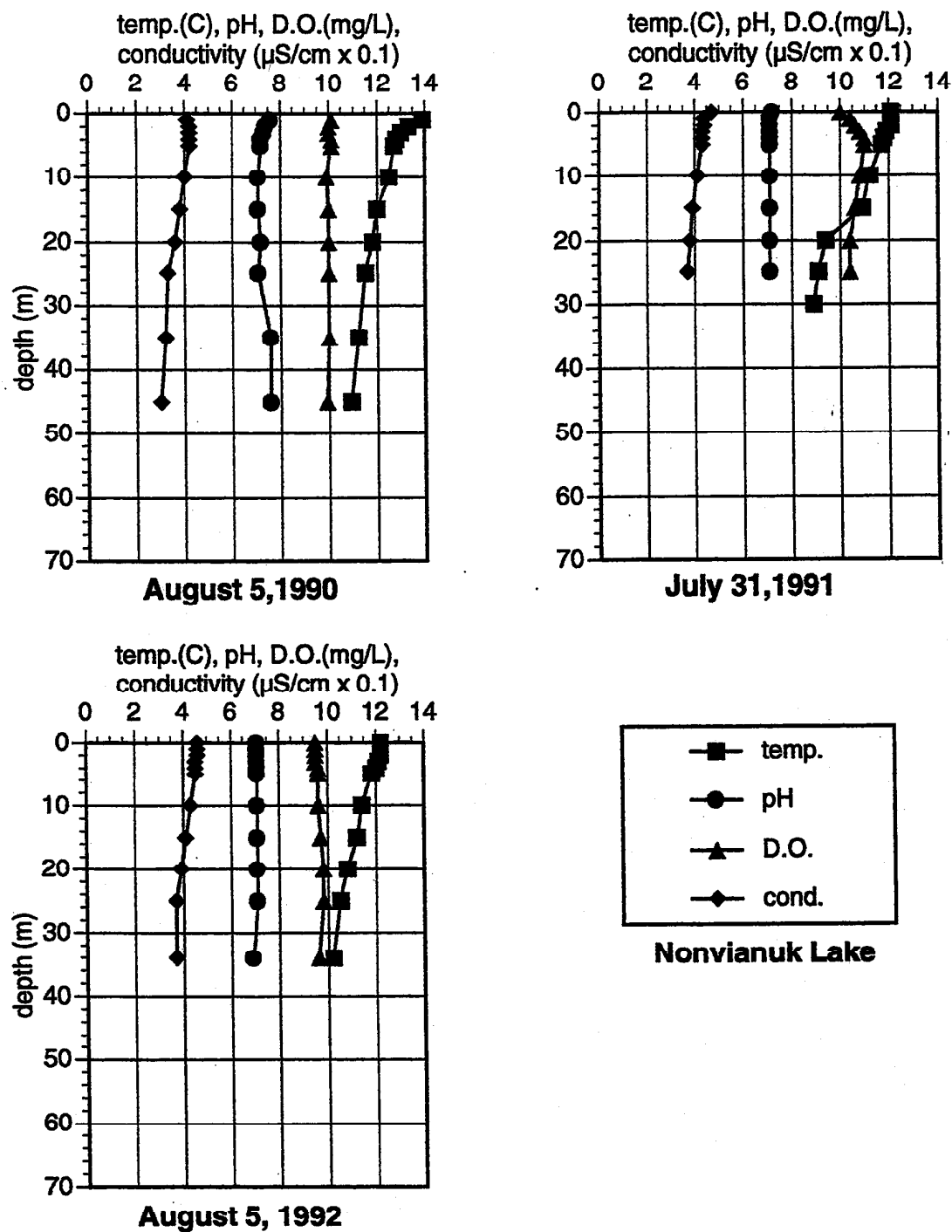
Figure 16. Depth profiles of water quality characteristics, Nonvianuk Lake.
