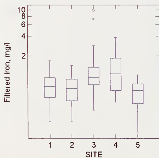
Figure 27. Box Plot for Filtered Iron
