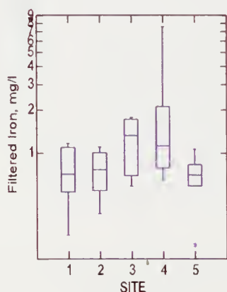
Figure 67. Box Plot of Wet Weather Filtered Iron.
