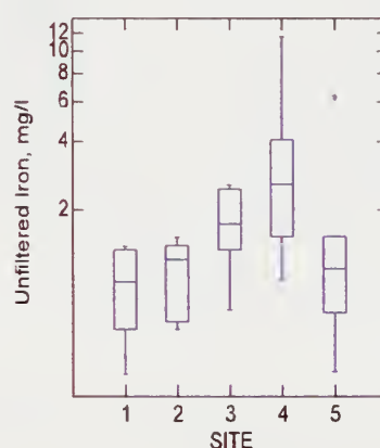
Figure 69. Box Plot of Wet Weather Unfiltered Iron.
