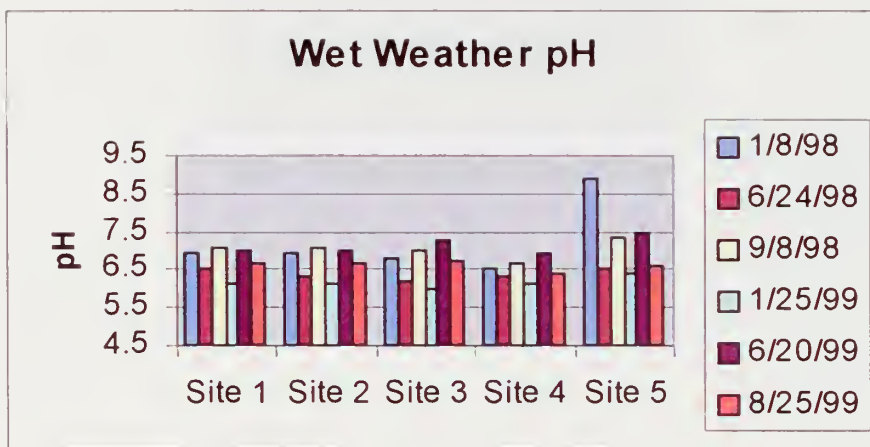
Figure 44. Wet Weather pH
