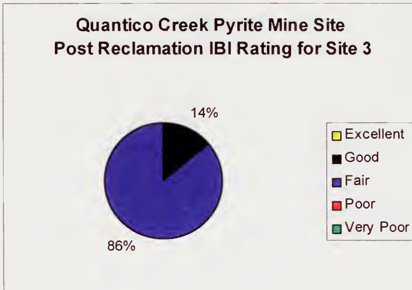
Figure 86. Post Reclamation IBI Ratings For Impacted Site 3
