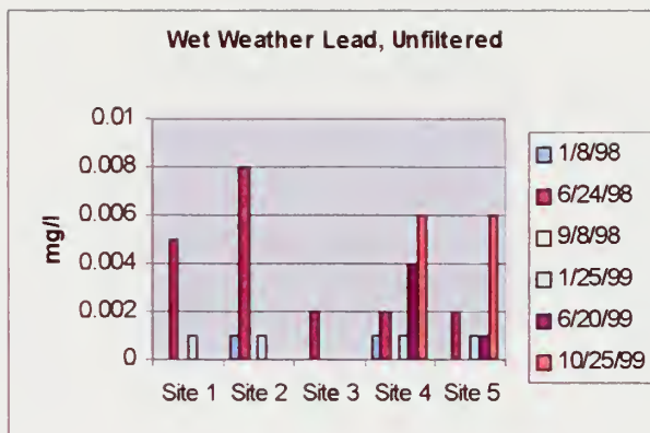
Figure 72. Wet Weather Unfiltered Lead
