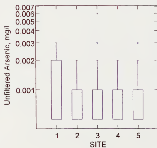
Figure 37. Box Plot for Unfiltered Arsenic
