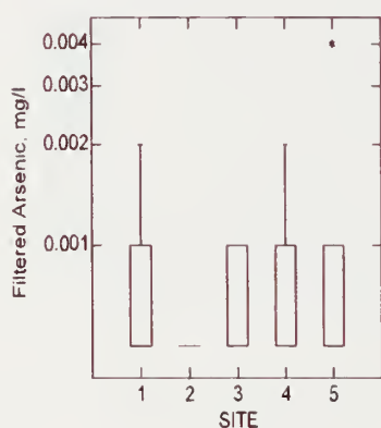
Figure 63. Box Plot of Wet Weather Filtered Arsenic
