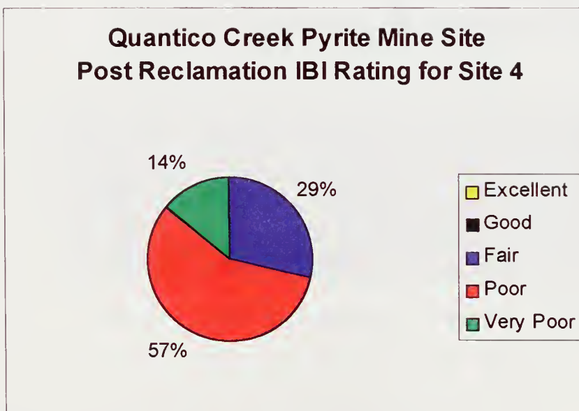
Figure 87. Post Reclamation IBI Ratings For Impacted Site 4
