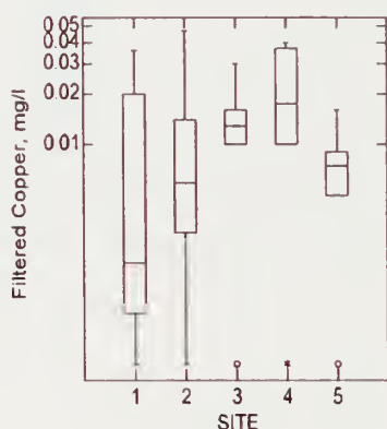
Figure 55. Box Plot Wet Weather Filtered Copper
