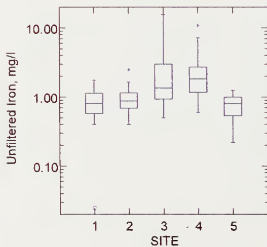
Figure 39. Box Plot for Unfiltered Iron
