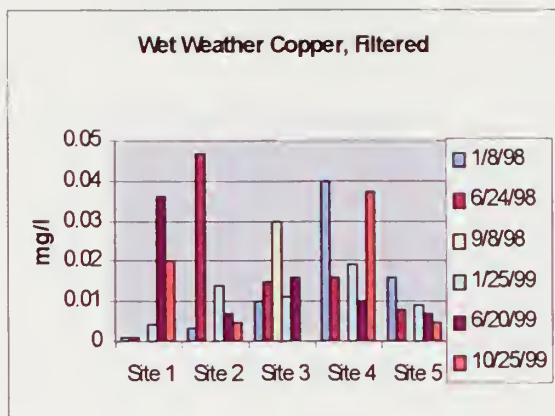
Figure 54. Wet Weather Filtered Copper
