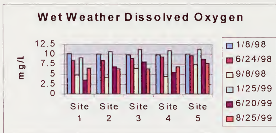
Figure 46. Wet Weather Dissolved Oxygen
