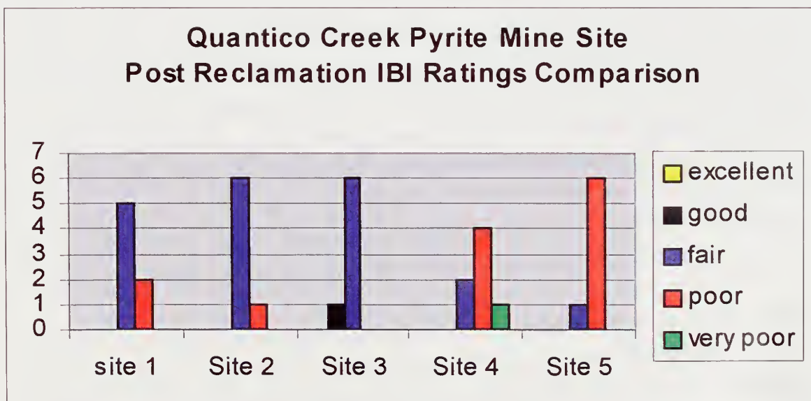
Figure 89. Comparison of IBI Ratings Among Sites
