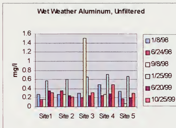
Figure 60. Wet Weather Unfiltered Aluminum
