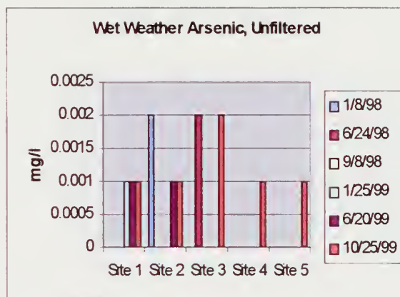
Figure 64. Wet Weather Unfiltered Arsenic
