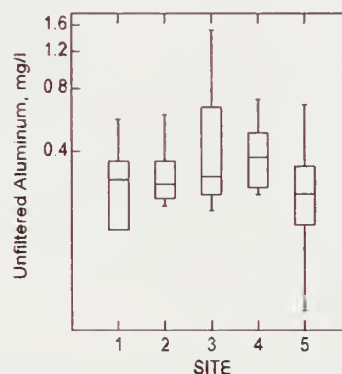
Figure 61. Box Plot of Wet Weather Unfiltered Aluminum
