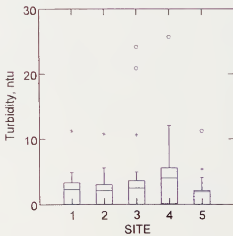
Figure 17. Box Plot of Turbidity
