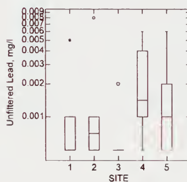
Figure 73. Box Plot of Wet Weather Unfiltered Lead
