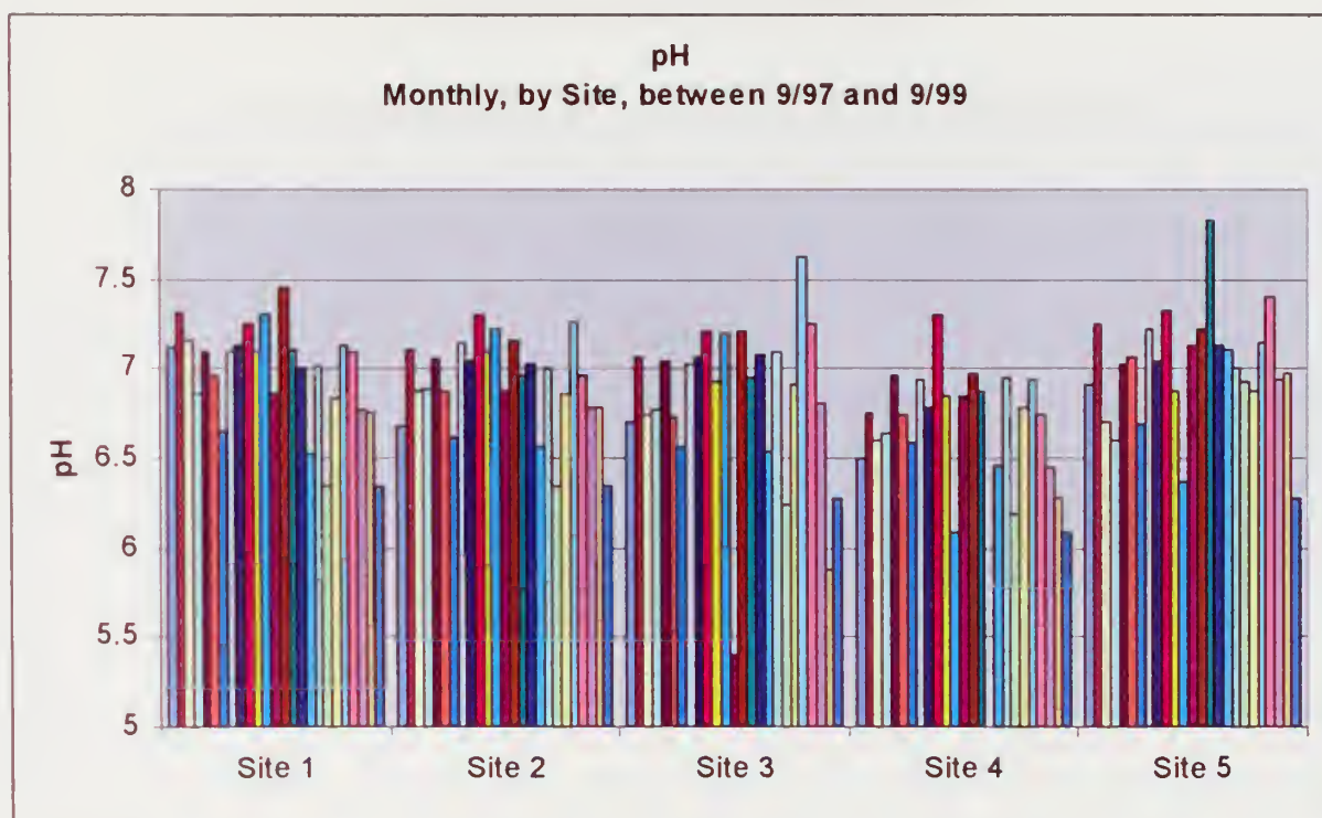
Figure 4. pH by Site
