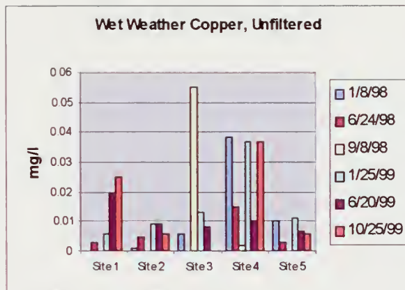
Figure 56. Wet Weather Unfiltered Copper
