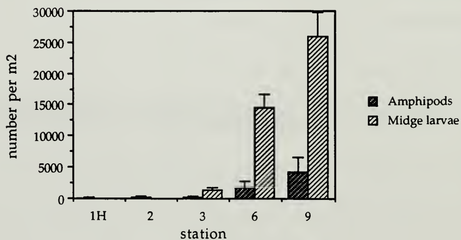
Fig. 35. Abundances of six benthic faunal groups vs station, averaged over 1991-92 sampling dates. \pm standard error. Please note that scale is different in top graph.
