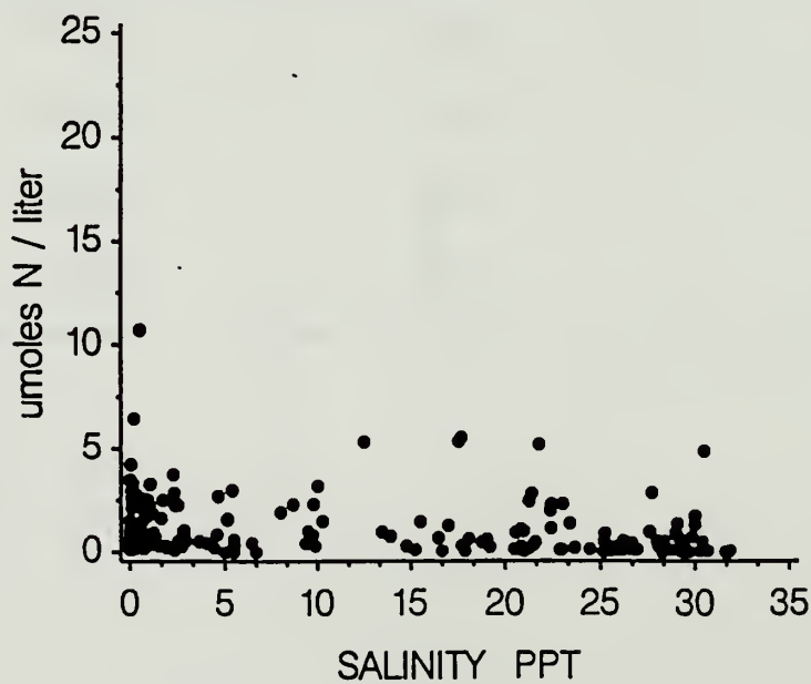
Fig. 16. Salinity vs property plots (a-j)
