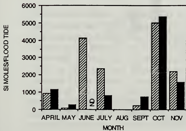
DISSOLVED SILICON LOADING
