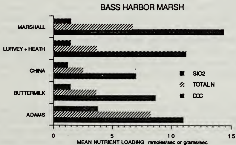
Fig. 12. Average nutrient loading (concentration x discharge) for the five freshwater brooks. Units are all mmol/sec except DOC which is grams/sec. n=7 in all cases except for total N and P where n=6.
