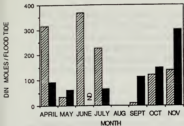
DISSOLVED INORGANIC NITROGEN LOADING
