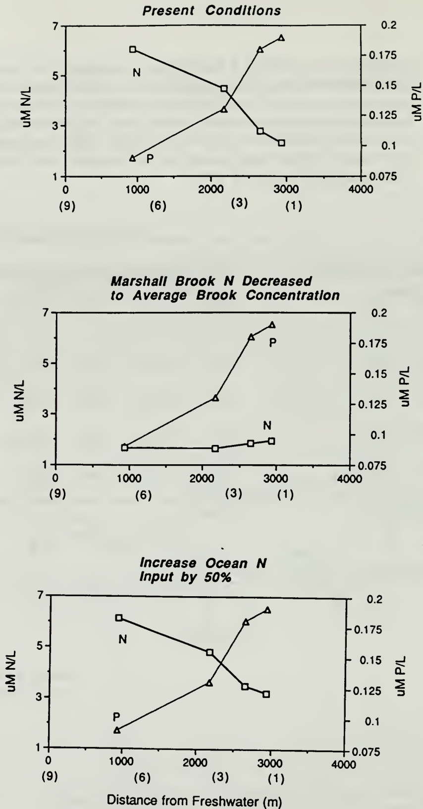
Fig. 18. Predicted DIN and DIP concentrations throughout the estuary from STELLA modelling. Model runs are for present conditions, decreasing DIN input from Marshall Brook, and increasing DIN from the ocean. A ratio of 16:1 is at the intersection of the plots. With distance from the freshwater end, station number is indicated in parentheses.
