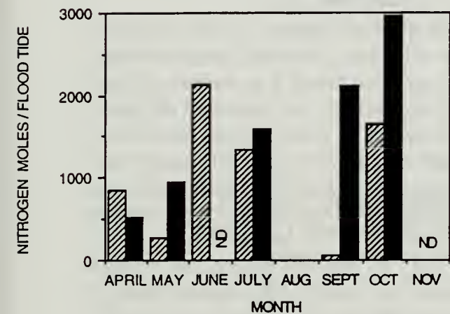
TOTAL NITROGEN LOADING
