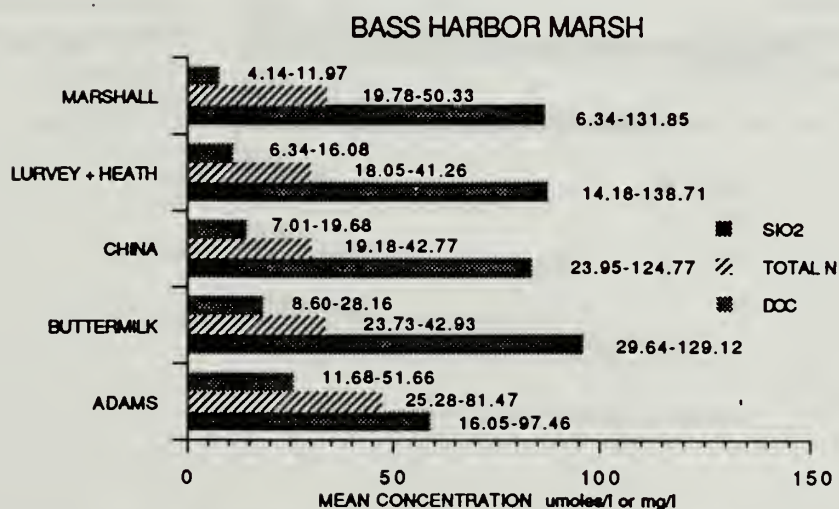
Fig. 11. Mean concentration of nutrients measured in the five fresh-water brooks. n=7 in all cases excepting total N and P where n=6 . Numbers above bars represent the range of concentrations measured. Units are all in \mu\text{moles/l} , except for DOC ( \text{mgC/l} ).
