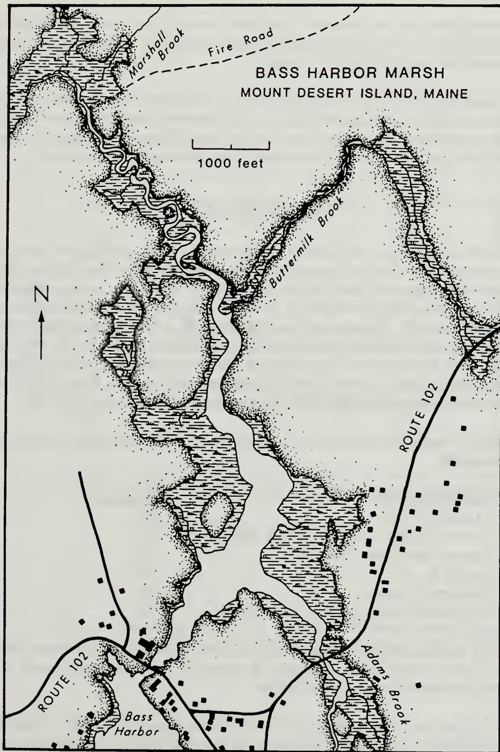
Fig. 2. Bass Harbor Marsh study site. Note freshwater drainages.
