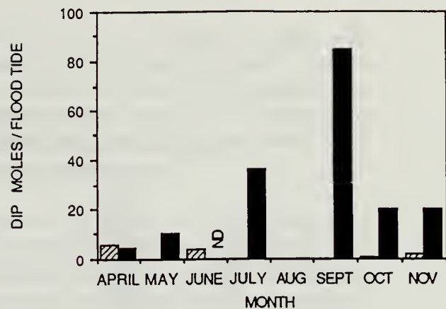
DISSOLVED INORGANIC PHOSPHORUS LOADING
