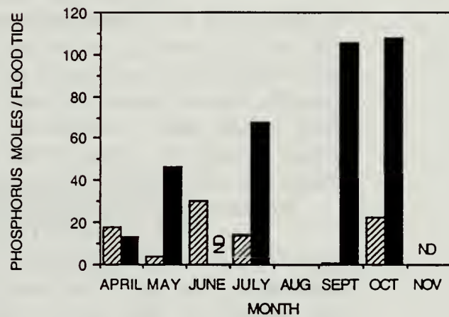
TOTAL PHOSPHORUS LOADING
