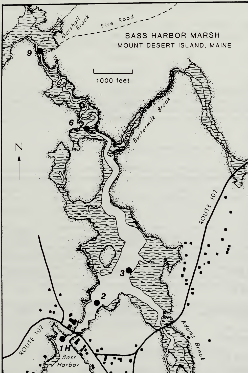
Fig. 32. Benthic macrofauna sample stations.
