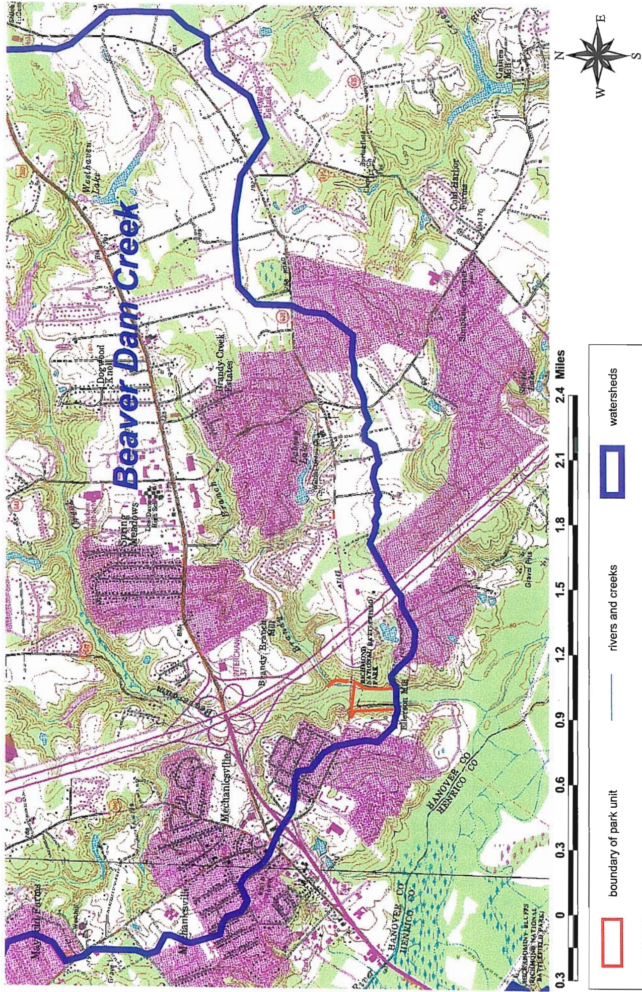
Figure 13. Map showing watershed contributing to the Beaver Dam Creek unit.
