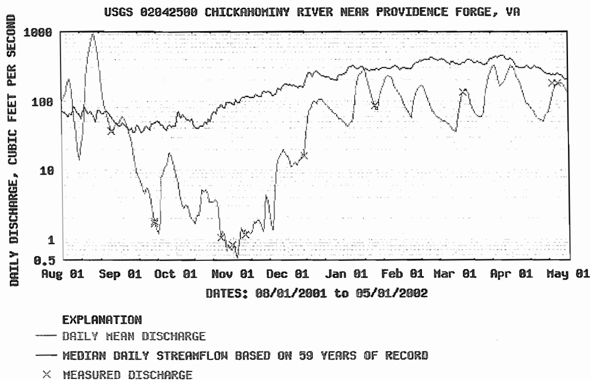
Figure 8. Indicator gage
