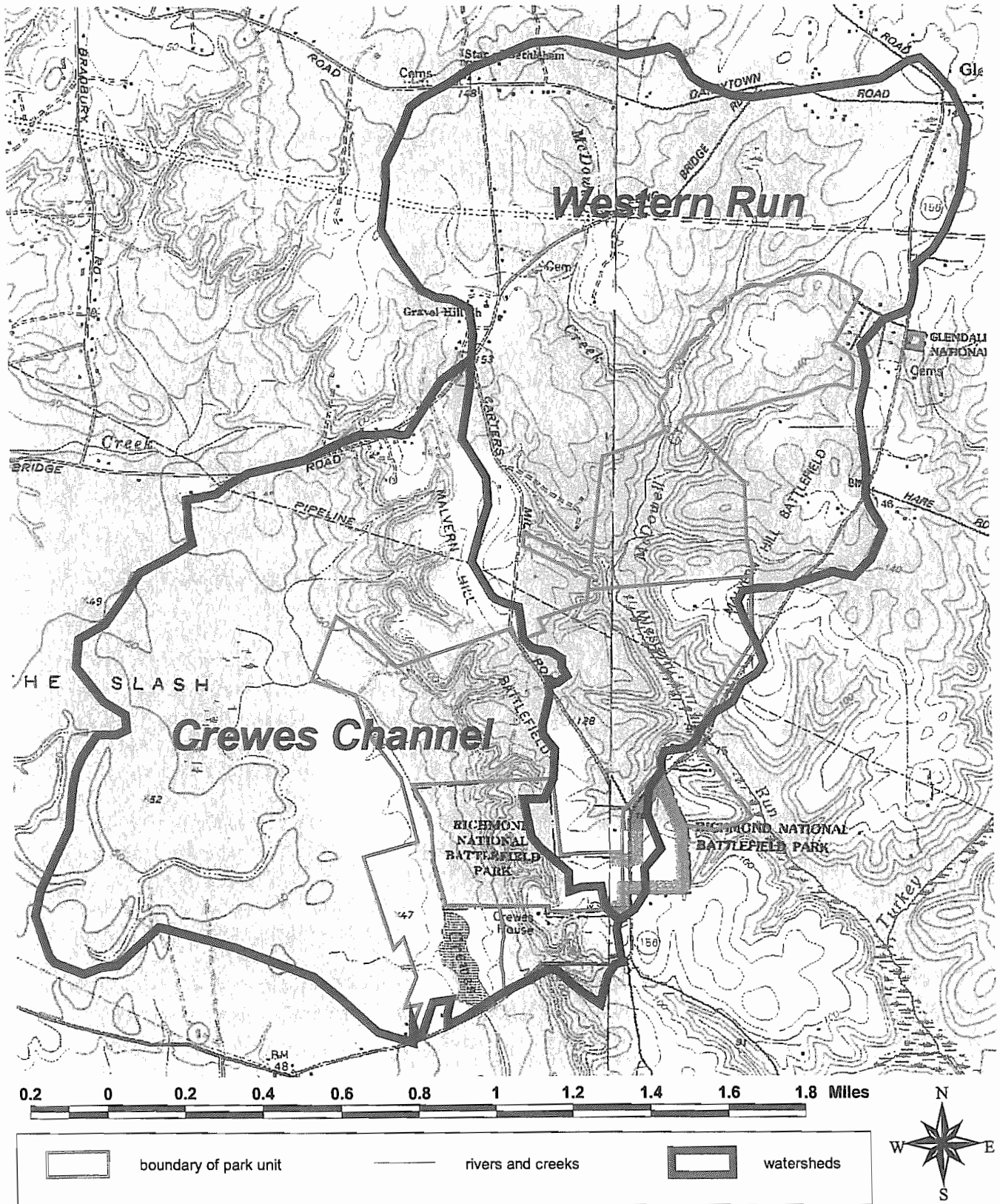
Figure 20. Map showing watershed contributing to the Malvern Hill/Glendale units.
