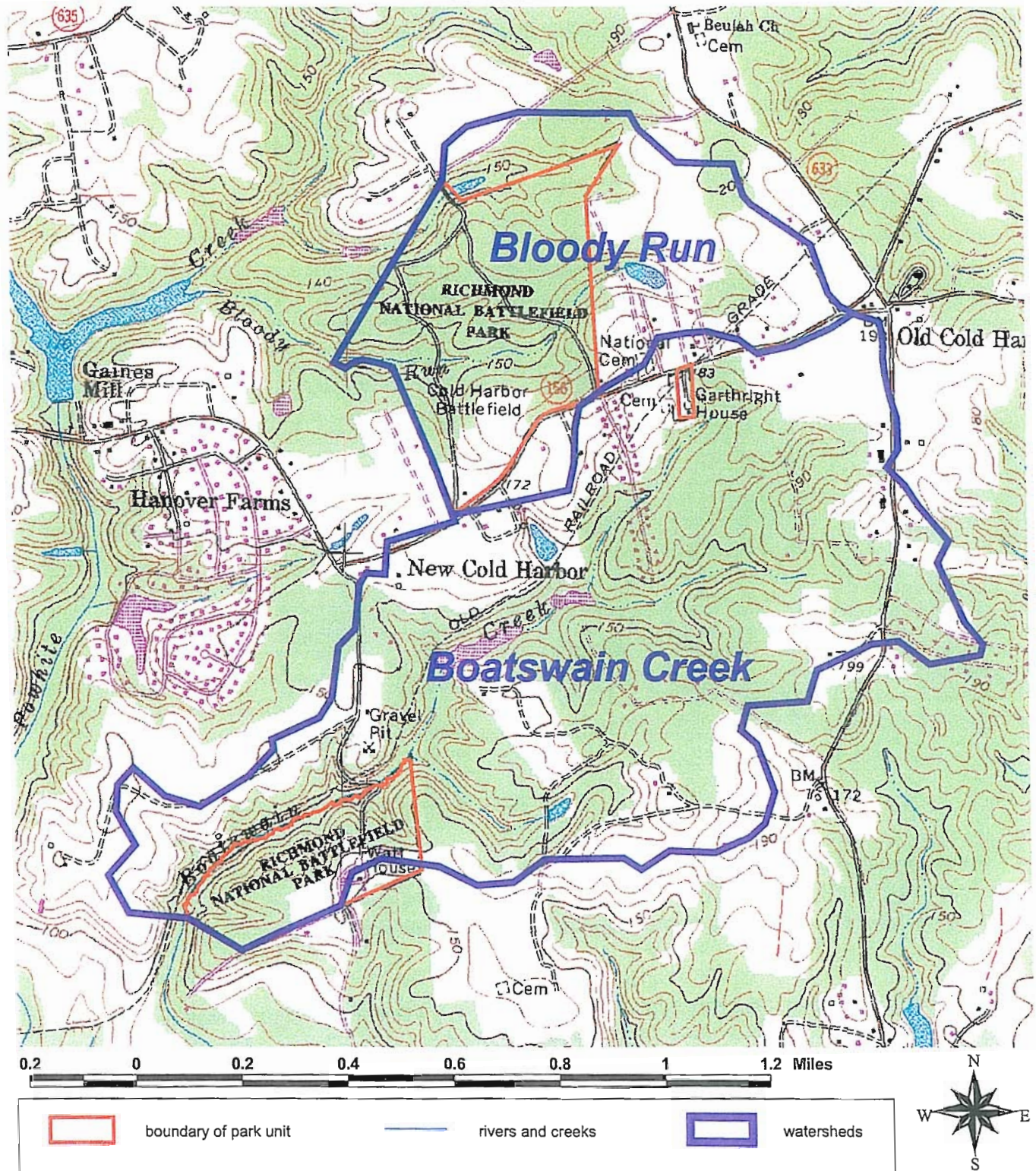
Figure 15. Map showing watershed contributing to the Cold Harbor unit, the Garthright House and the Gaines' Mill unit.
