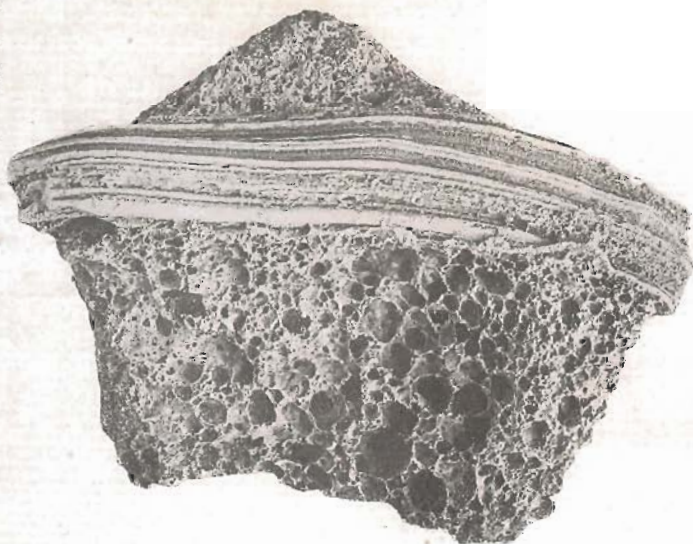
B.—A ribbon bomb "frozen" to a cinder. These long strips of lava are broken off the spindly bombs or ome. They owe their origin to the pulling apart of two clots of lava travelling at slightly different speeds or in different directions. Natural size.
