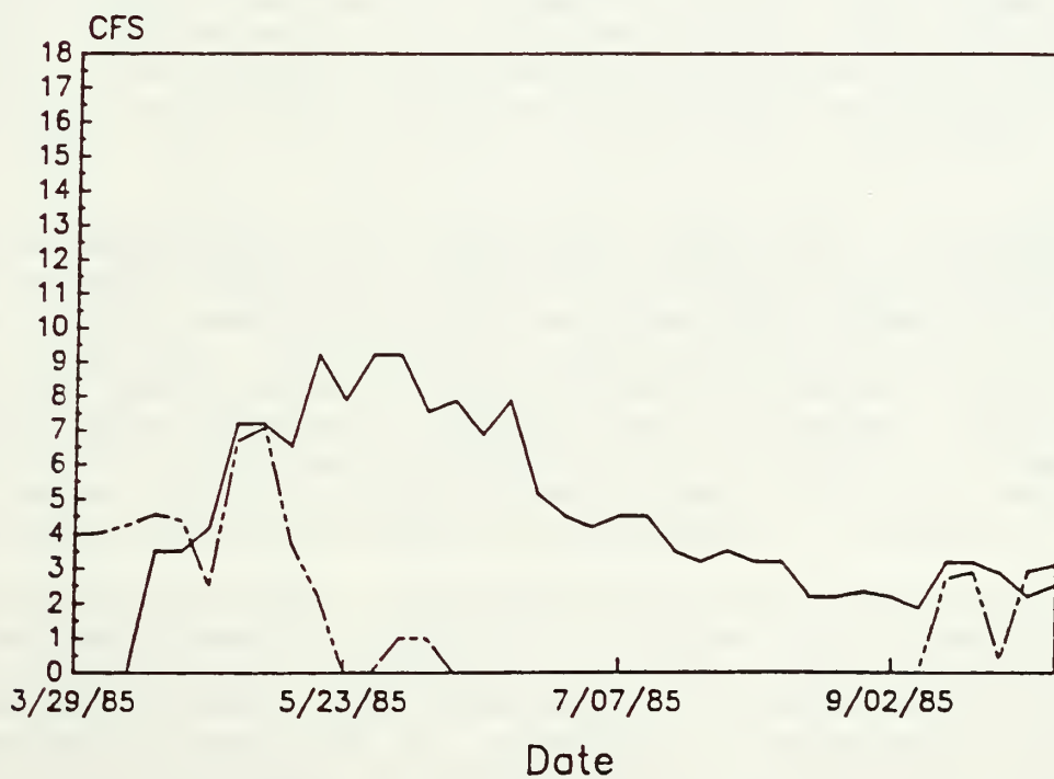
Figure 6. Stream flow pattern in Reese Creek, Yellowstone National Park, at the upper and lower staff gauge sites, 1984 and 1985.
