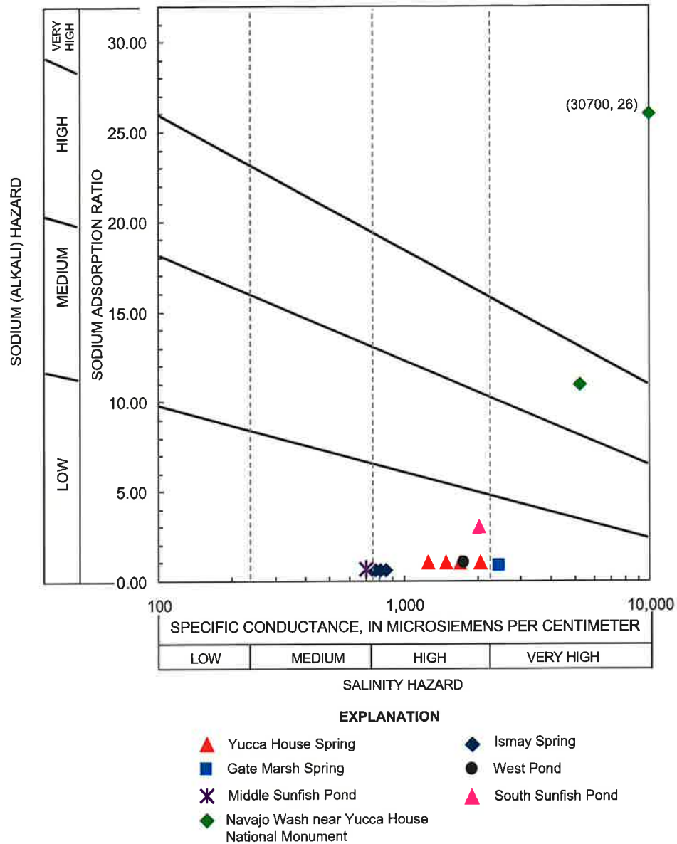
Figure 18. Salinity and sodium (alkali) crop hazard and water-quality results from Yucca House National Monument.
