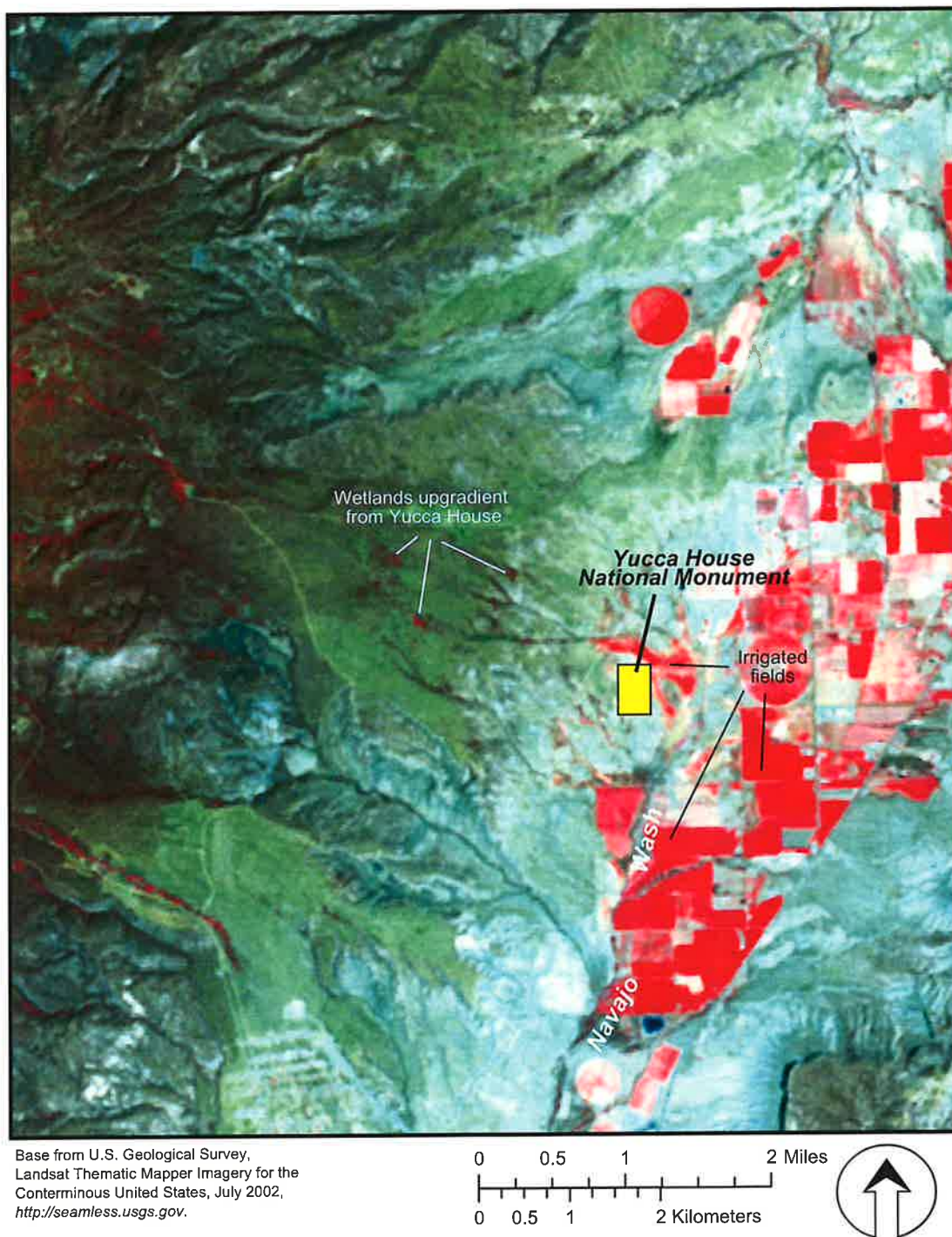
Figure 9. Color infrared imagery showing water-loving plants (phreatophytes) in bright red colors.
