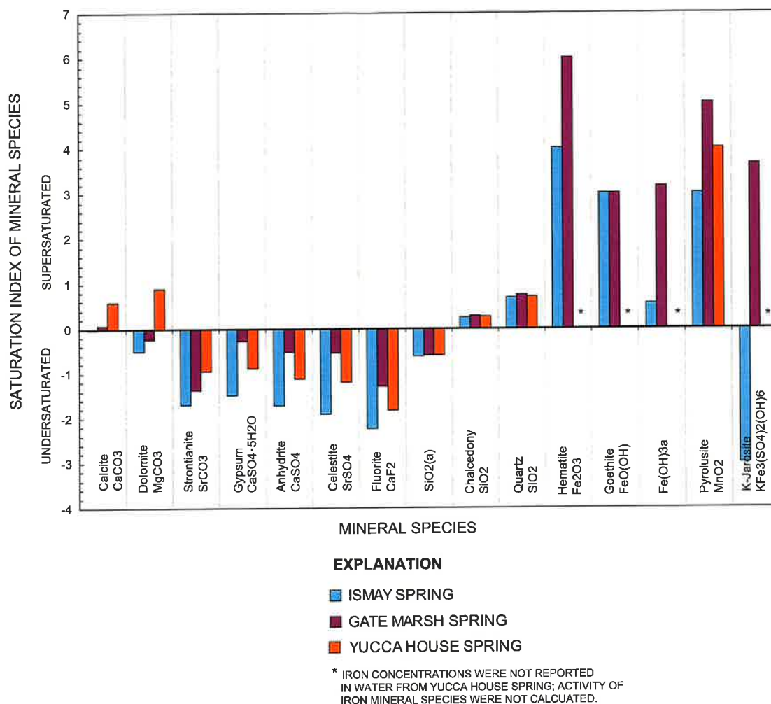
Figure 15. Saturation index of mineral species for springs in the Yucca House area. Saturation index less than zero indicates undersaturation, and the mineral species would be dissolving in a water-rock interaction environment. Saturation index greater than zero indicates saturation, and the mineral would be precipitating from the dissolved phase into the solid phase.
