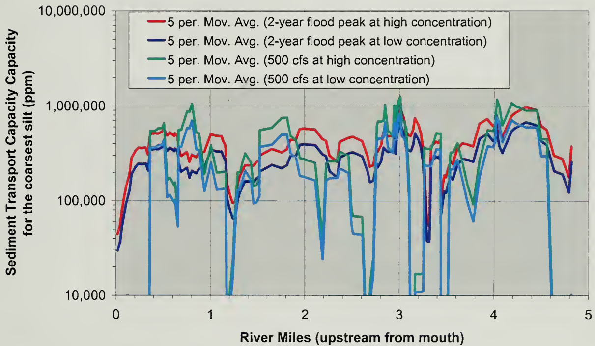
Figure B1. Hydraulic capacity to transport coarse silt particles (0.062 mm) along the Elwha River is shown for river discharges of 500 and 14,470 ft 3 /s. When sediment concentrations are high (40,000 mg/l), the sediment transport capacity increases due to the increase in density and viscosity of the fluid-sediment mixture.
