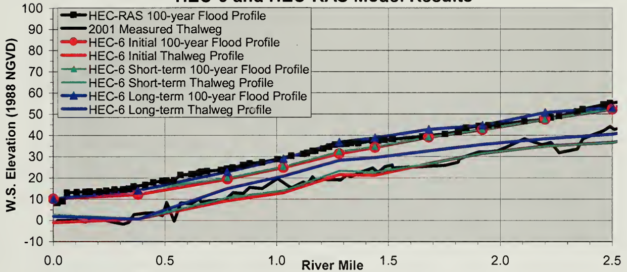
Figure 3. Comparison of HEC-6 and HEC-RAS model results for the reach between river miles 0 and 2.5.
