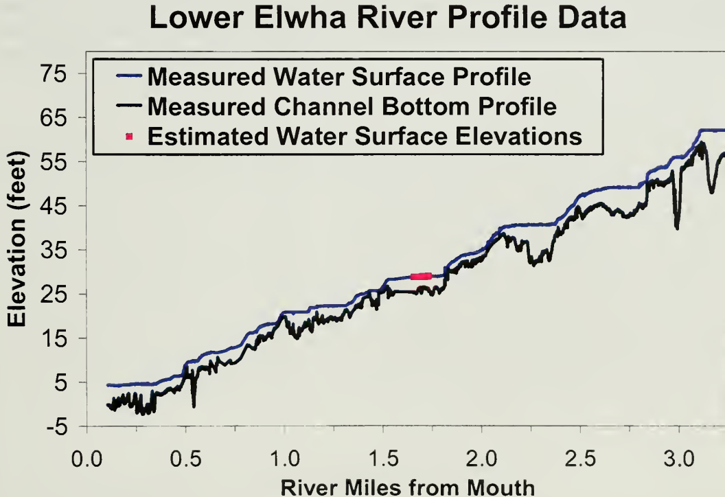
Figure 7. The longitudinal profile of the lower Elwha River is relatively steep with an average slope of 0.0034. This profile was produced from the 2001 river channel survey data at an average discharge of 990 ft 3 /s.
