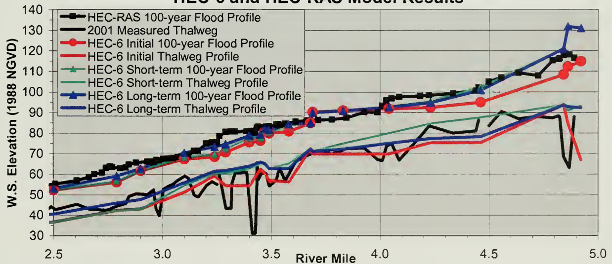
Figure 4. Comparison of HEC-6 and HEC-RAS model results for the reach between river miles 2.5 and 5.
