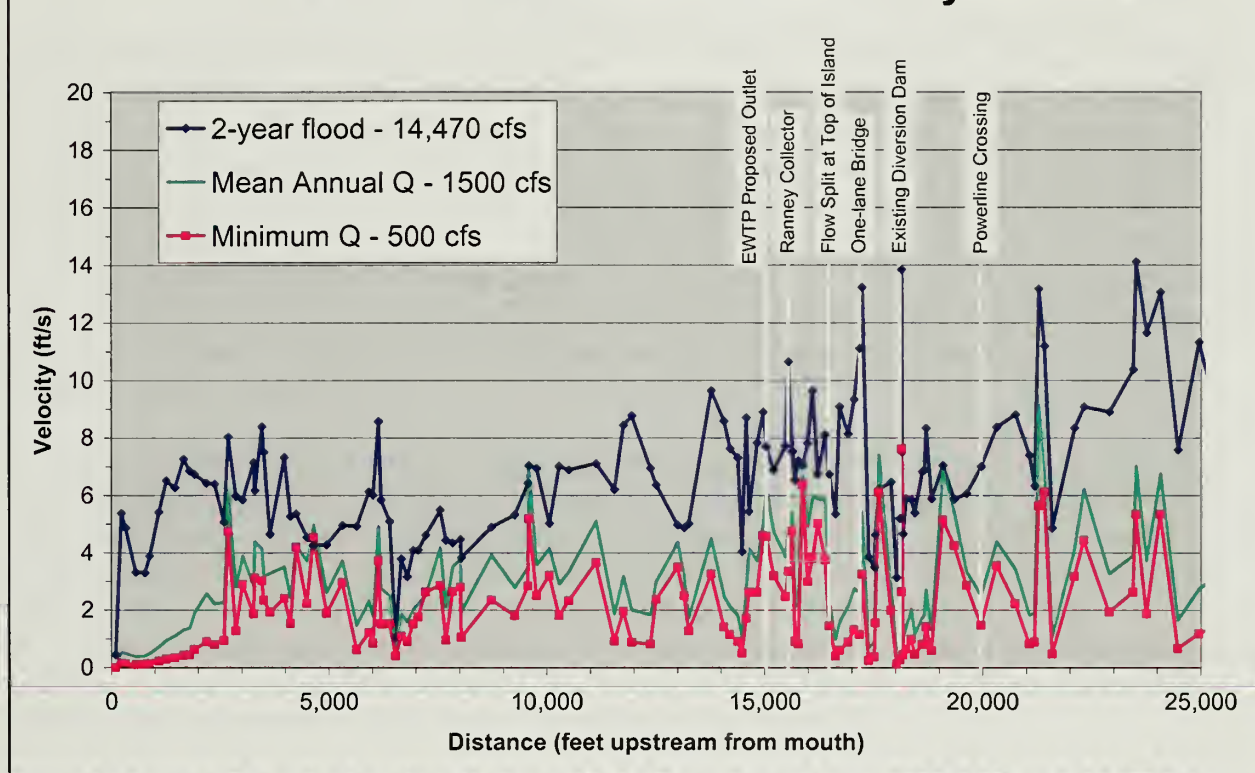
Figure 6. Average flow velocities along the lower Elwha River during flows of 500, 1,500 and, 14,470 \text{ft}^3/\text{s} .
