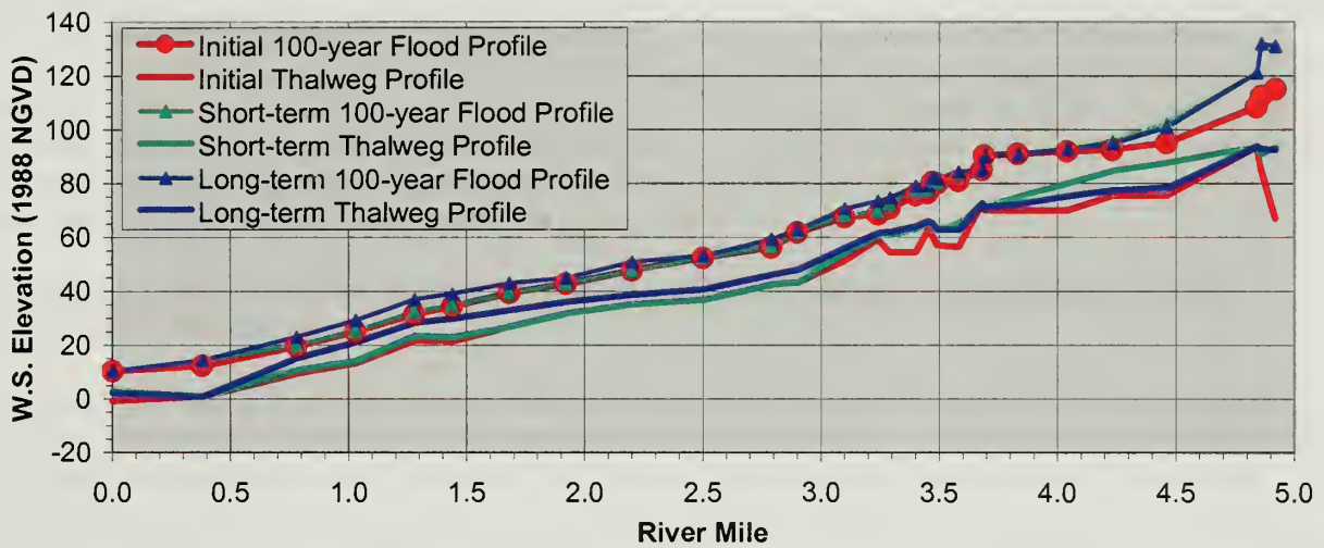
Figure 1. Longitudinal River Profile of HEC-6 Model Results.
