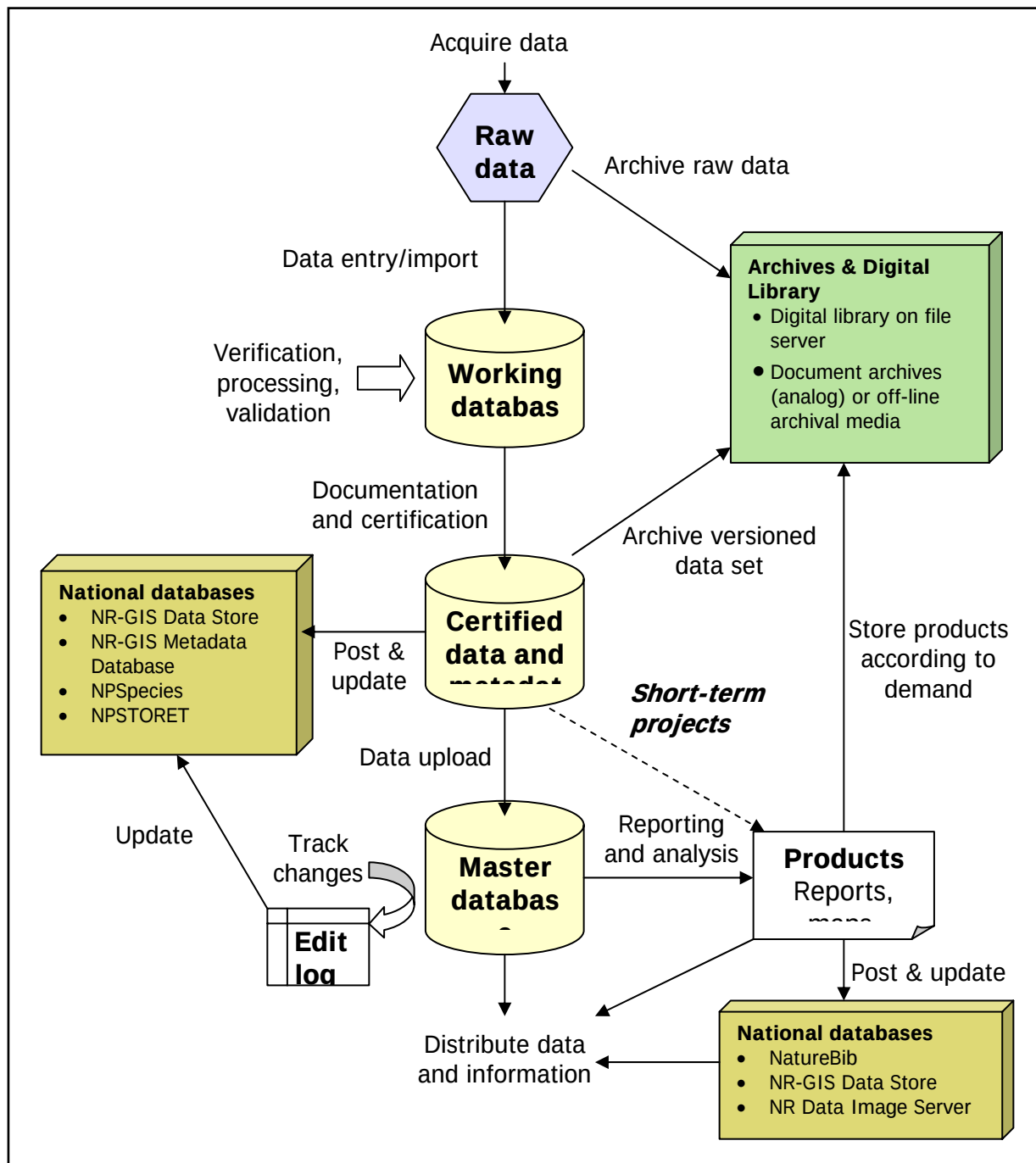
Figure 0.4 Diagram of the typical project data life cycle.
