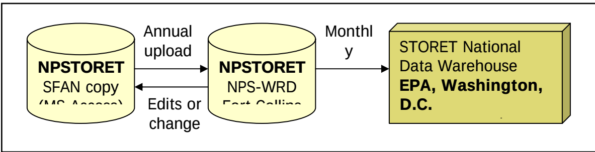
Figure 0.5 Data flow diagram for water quality data.
