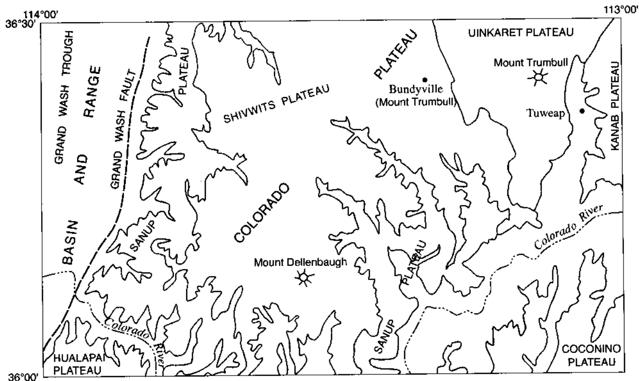
Figure 1. Index map of the Mount Trumbull 30' x 60' quadrangle, Arizona showing the physiographic provinces and subprovinces.
